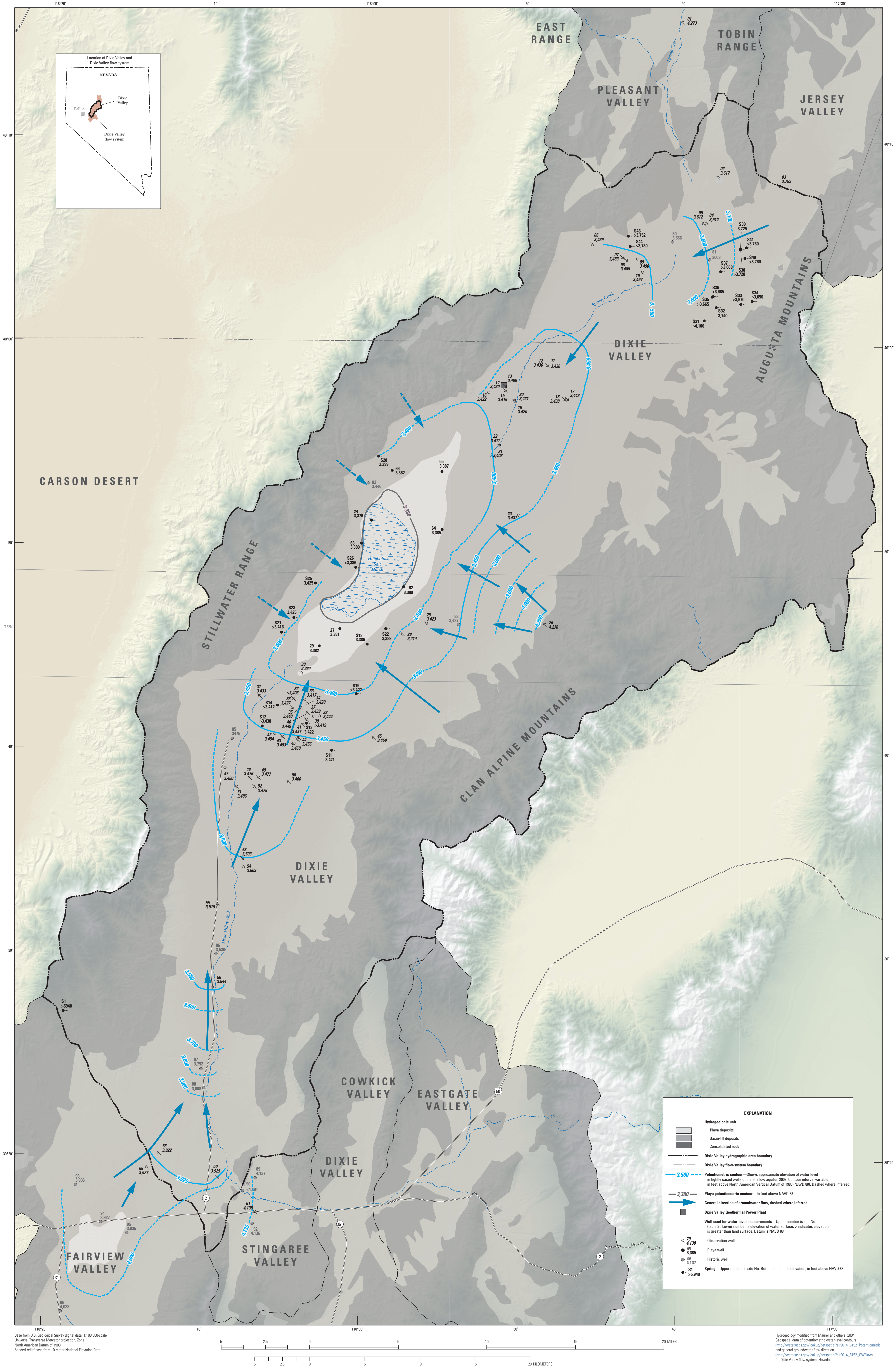
Potentiometric Water-Level Elevation at Selected Wells and Potentiometric Contours of Water-Level Elevation, Dixie Valley, West-Central Nevada, Autumn 2009
