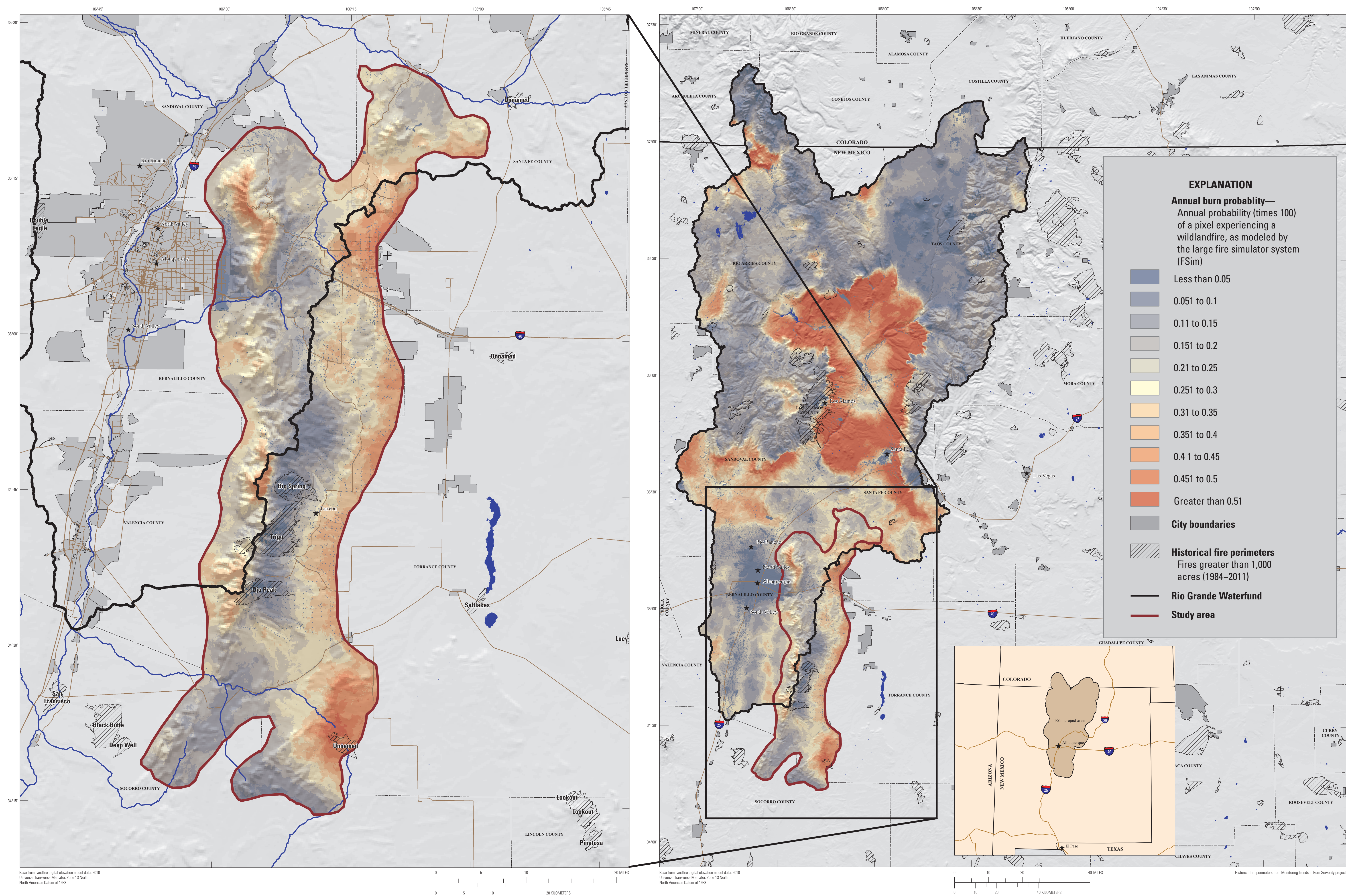
Figure 5. Results of burn probability simulation using large fire simulation system.
