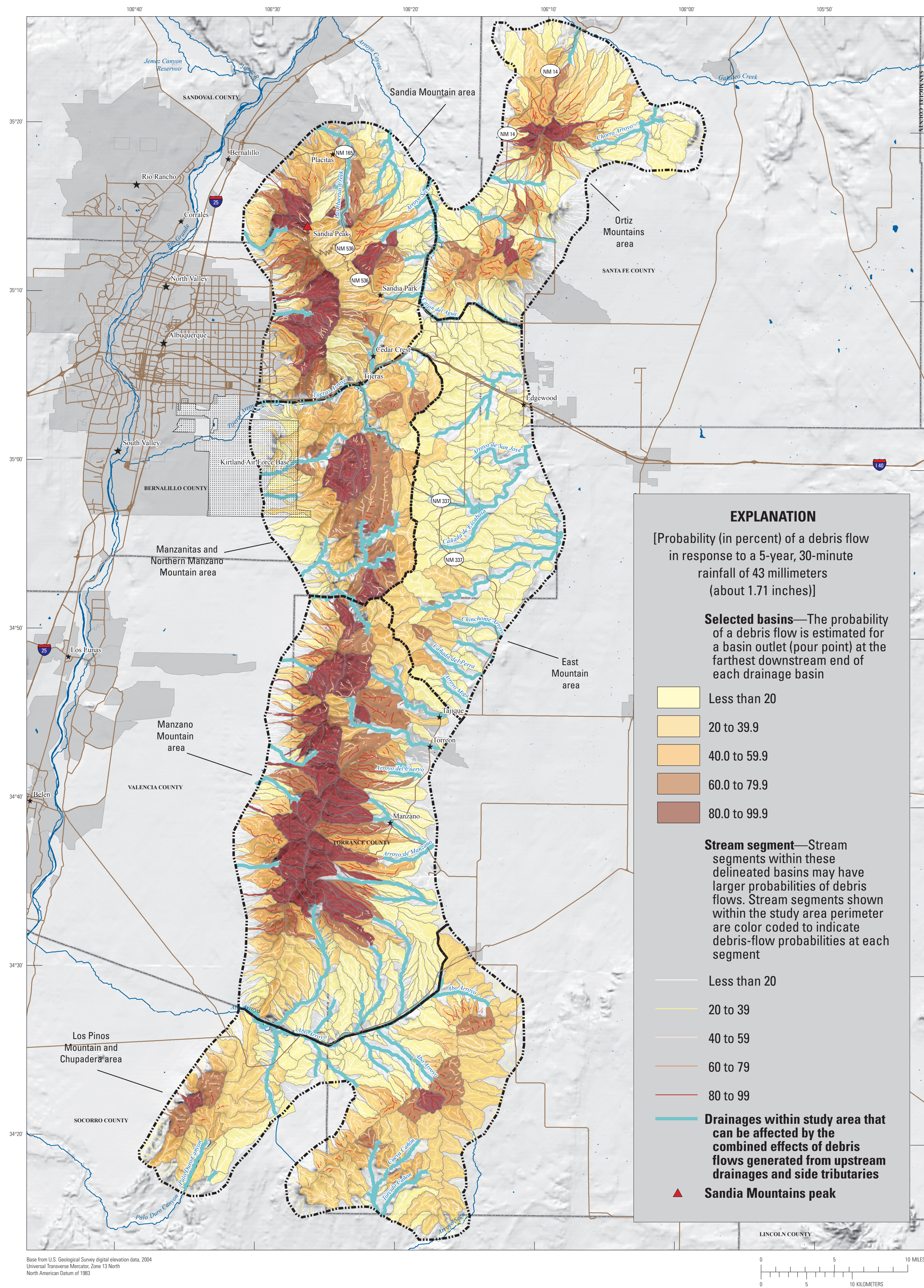
Figure 6. Debris-flow probability and debris-flow volume.
