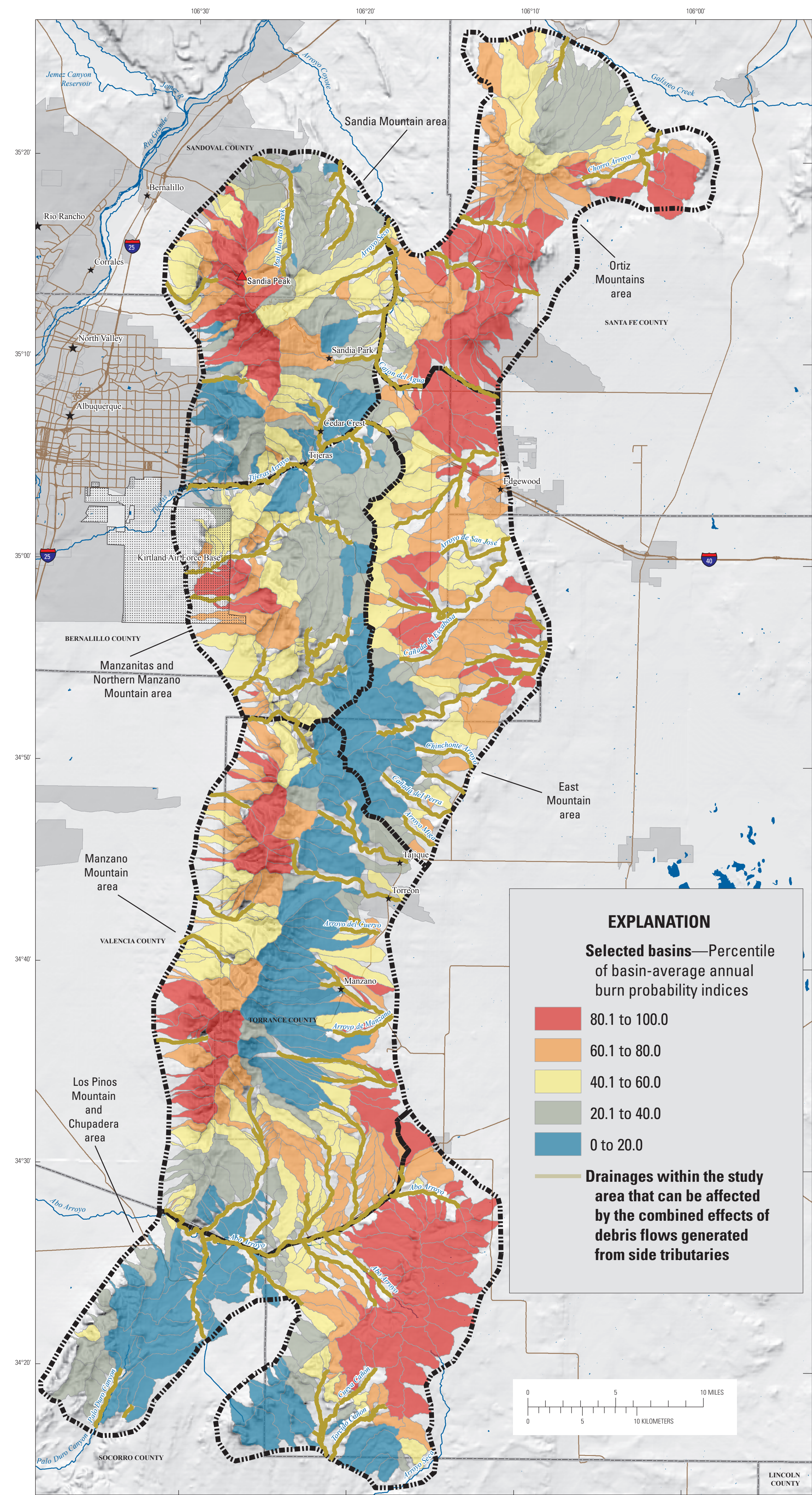
Figure 8. Percentile of continuously parameterized burn probability indices and integrated debris-flow hazard indices plate.
