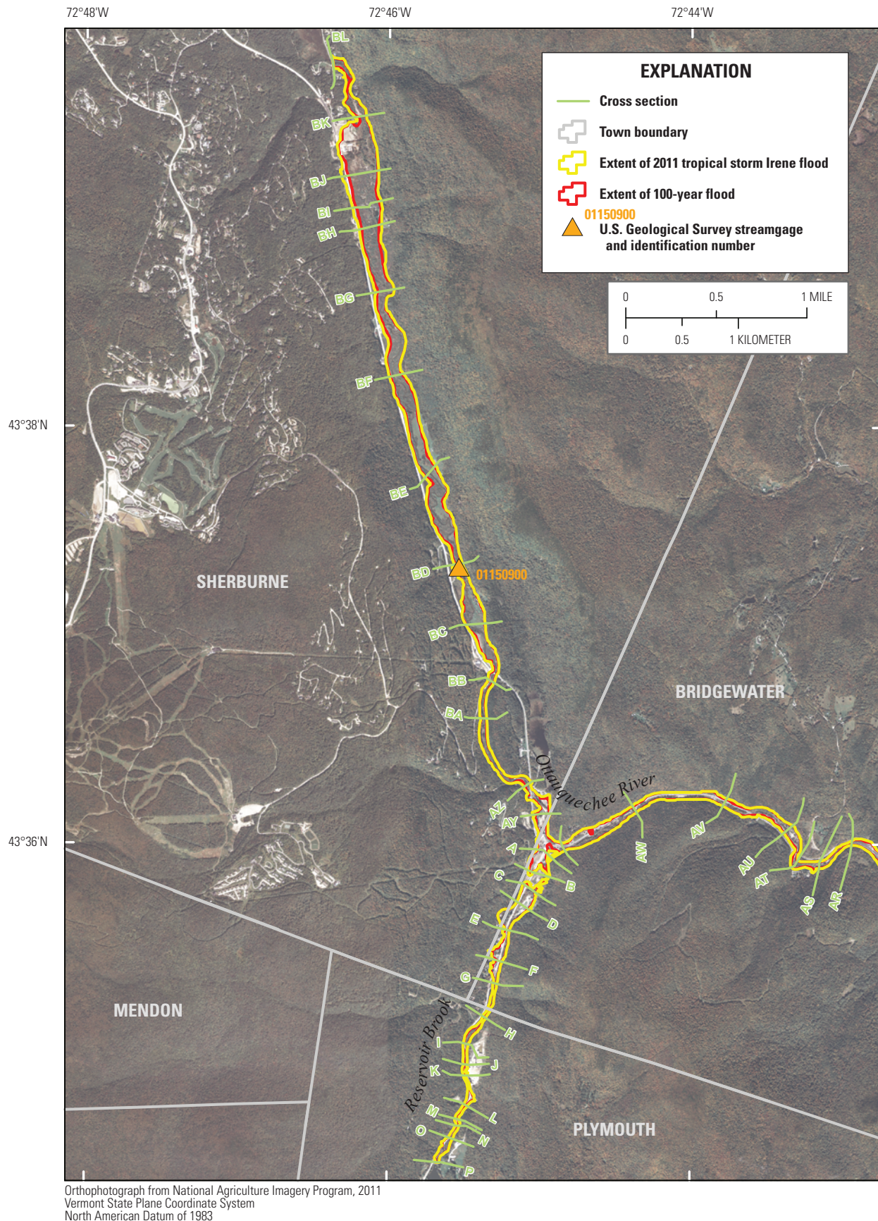
Figure 1-2. Flood inundation on the Ottauquechee River and Reservoir Brook, Vermont, and the locations of cross sections and U.S. Geological Survey streamgage 01150900 Ottauquechee River near West Bridgewater, Vt., in Plymouth and Sherburne and parts of Bridgewater, Vt.
