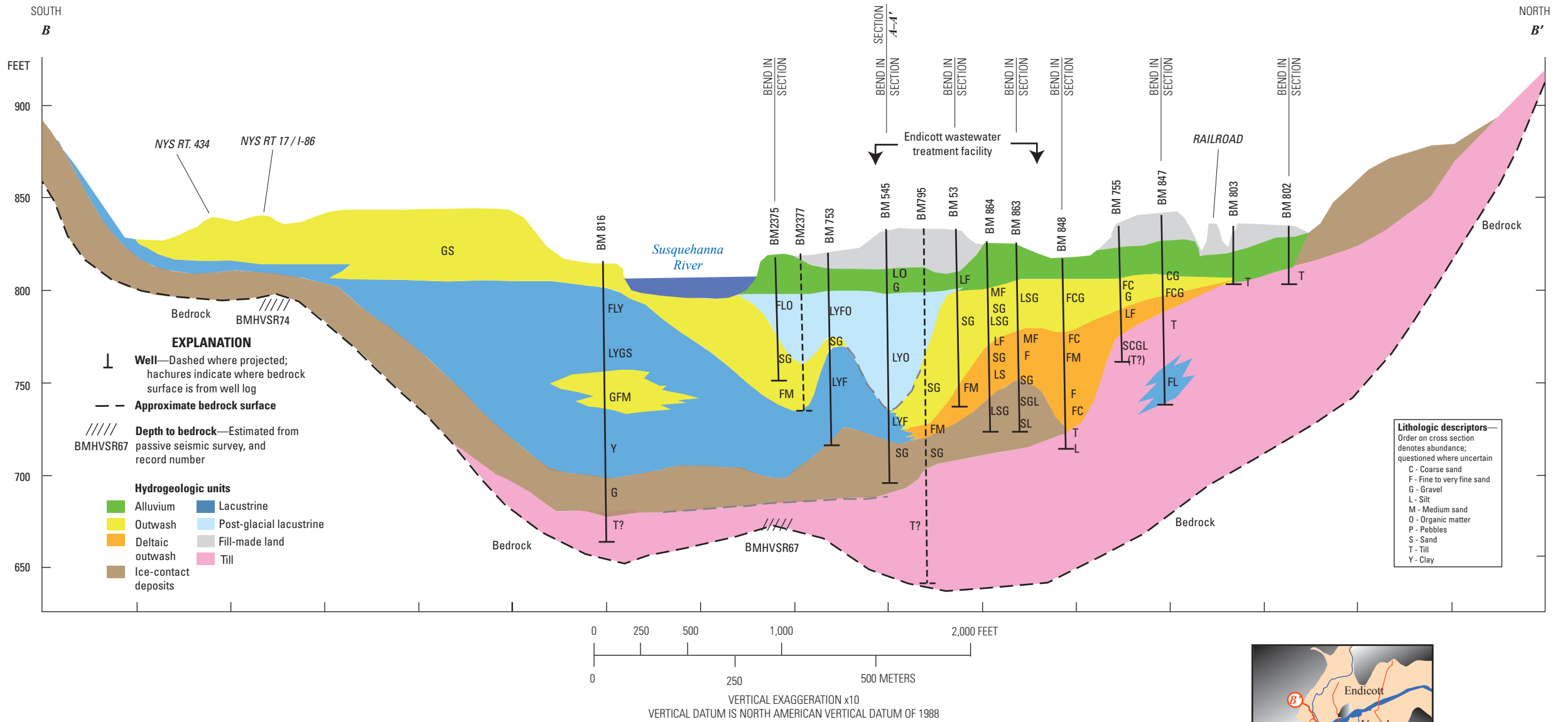
Figure 6. Geologic section B-B' in the Susquehanna River valley, near Endicott and Vestal, southwestern Broome County, New York. Section lines are shown in figure 2.
