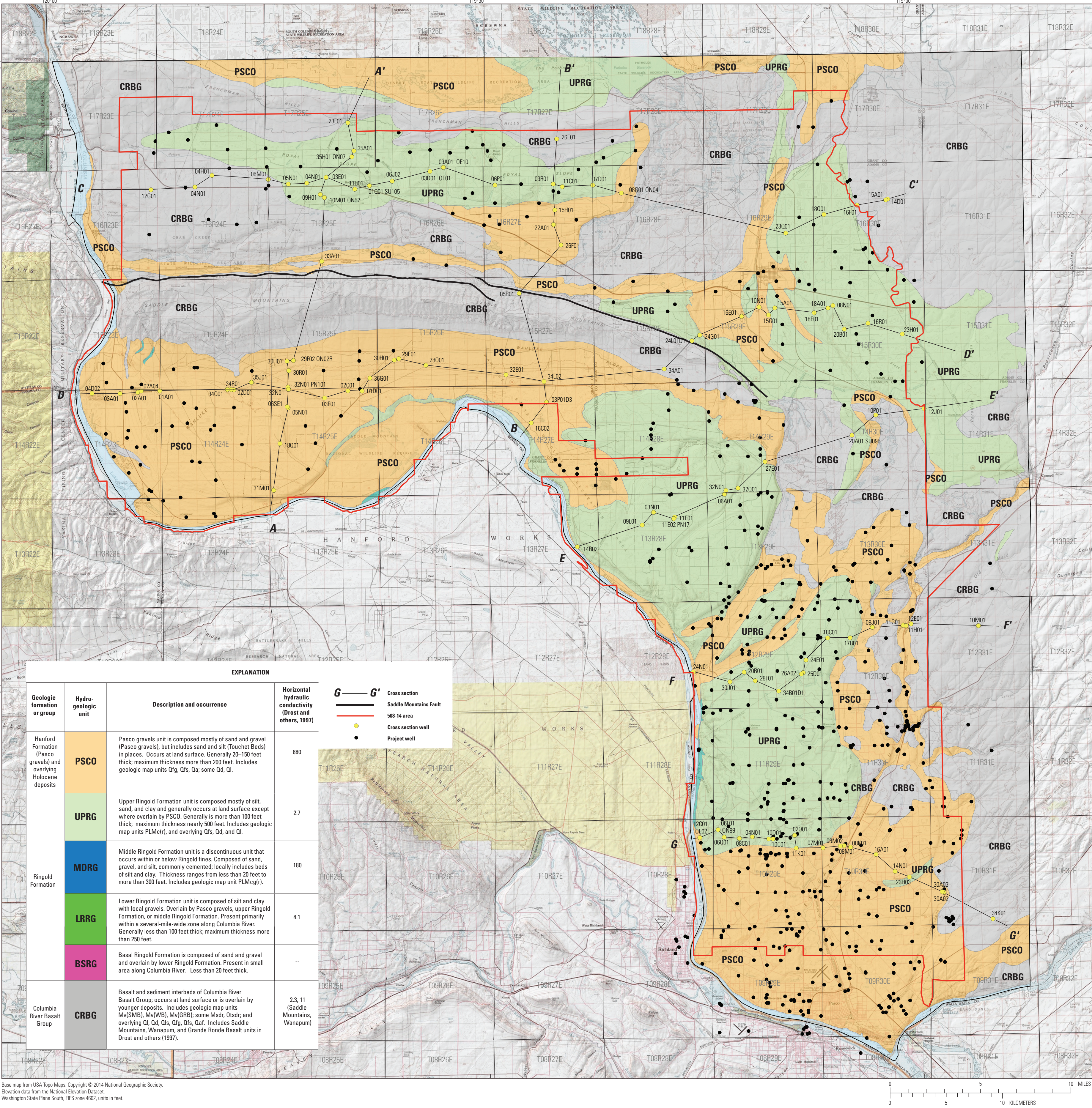
Hydrogeologic Unit Map, Hydrogeologic Sections, and Locations of Project Wells, Eastern Pasco Basin, Washington
