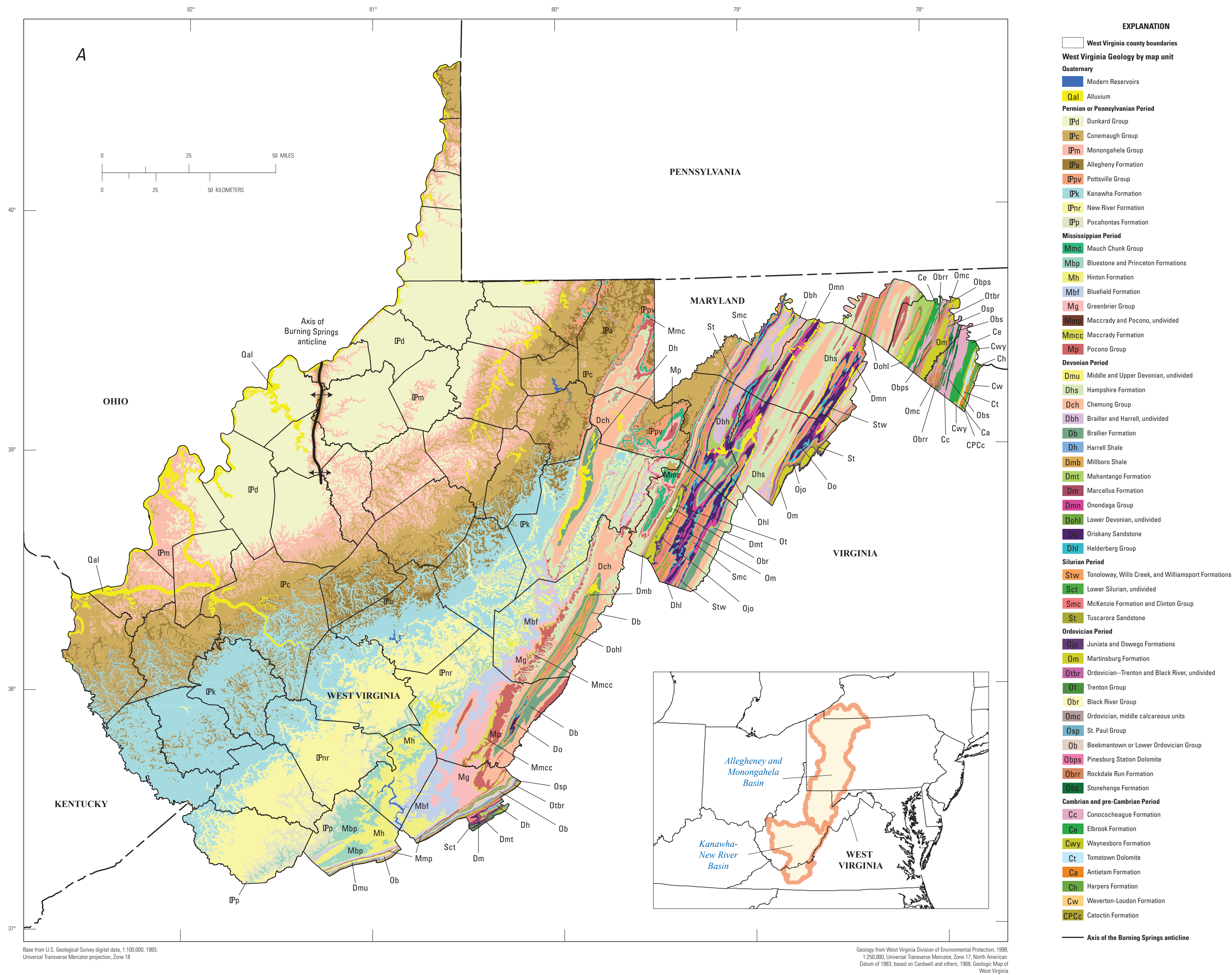
Figure 3A. Major geologic formations in West Virginia.
