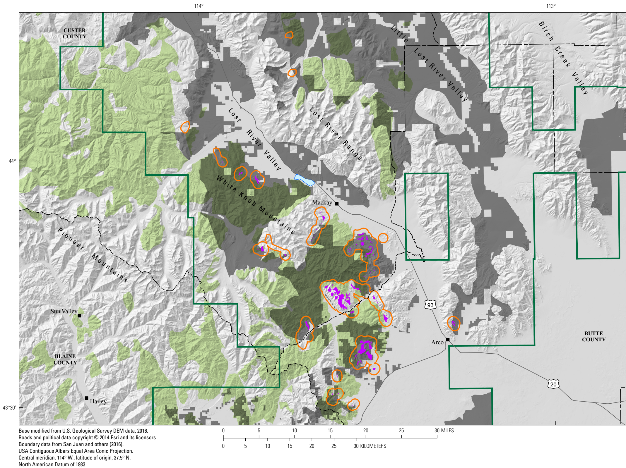
Figure 23. Inset map showing details of mineral-resource-potential tracts for jasperoid precious-metals occurrences in context of permissive geology in the central part of the study area for the North-Central Idaho Sagebrush Focal Area.
