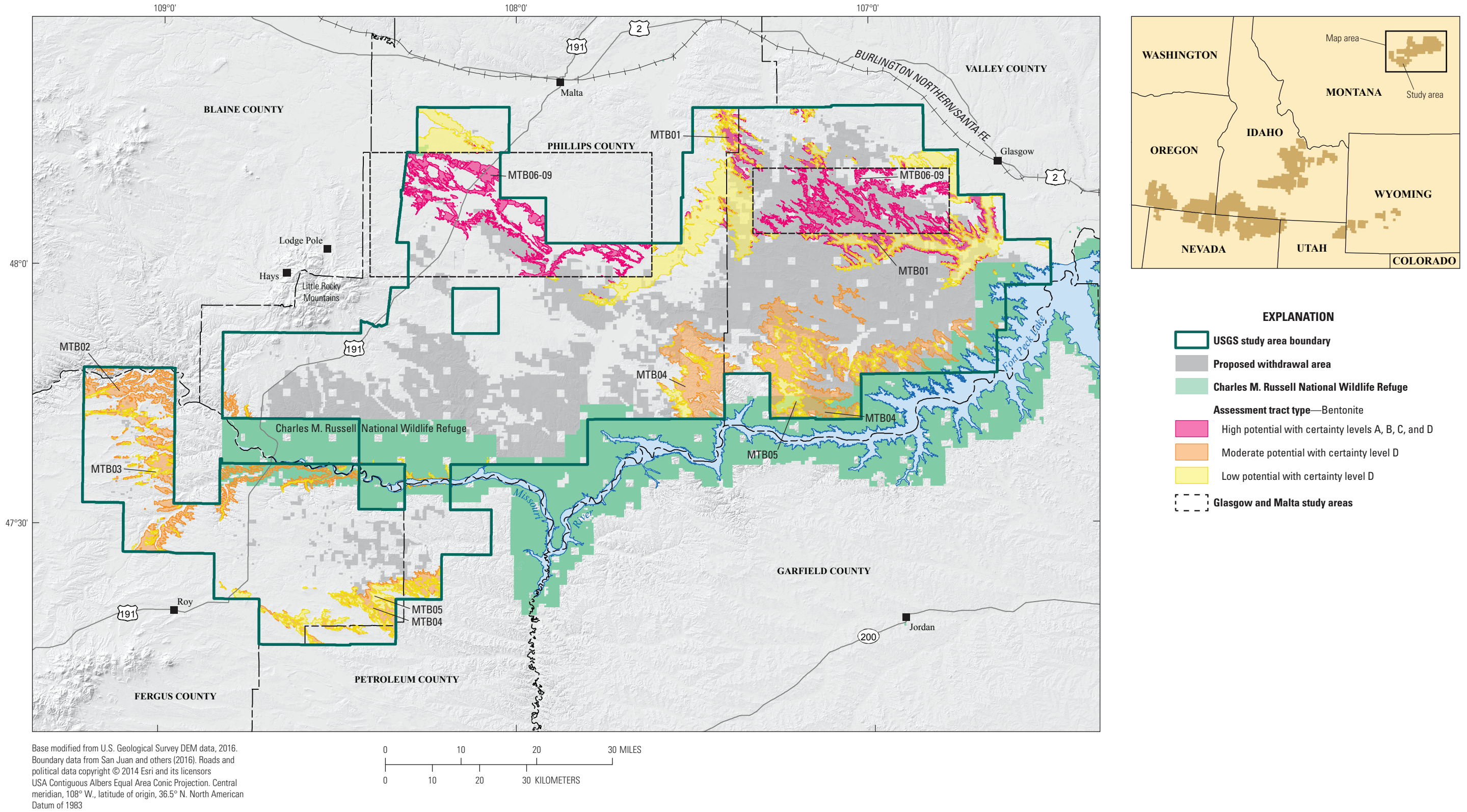
Figure 27. Mineral potential map for sedimentary bentonite deposits in the North-Central Montana Sagebrush Focal Area. This map shows how the two approaches used to assess bentonite in the study area were integrated for the geographic information system database that accompanies the assessment reports (San Juan and others, 2016). USGS, U.S. Geological Survey.
