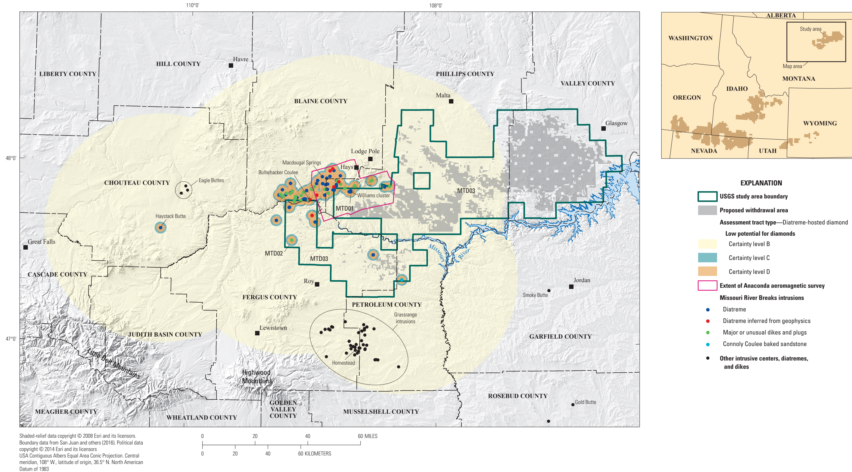
Figure 29. Map showing the location of diatremes and related igneous rocks in the study area and the surrounding region (modified from Hearn, 1979, 2004; McGee and Hearn, 1989; Irving and Hearn, 2003; Faure, 2010; Anderson and others, 2016). Map also shows mineral potential for diamond deposits in the North-Central Montana Sagebrush Focal Area. USGS, U.S. Geological Survey.
