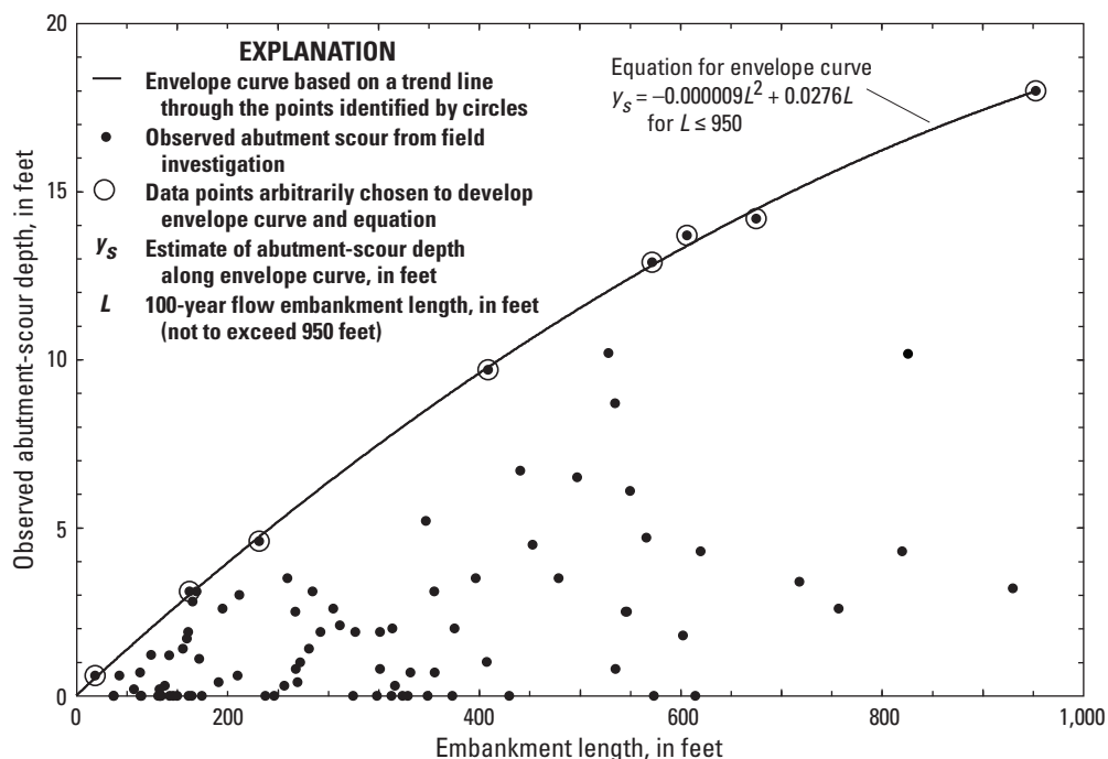
Figure 26. The South Carolina Piedmont clear-water abutment-scour envelope curve with respect to the embankment length blocking flow (from Benedict, 2003).
