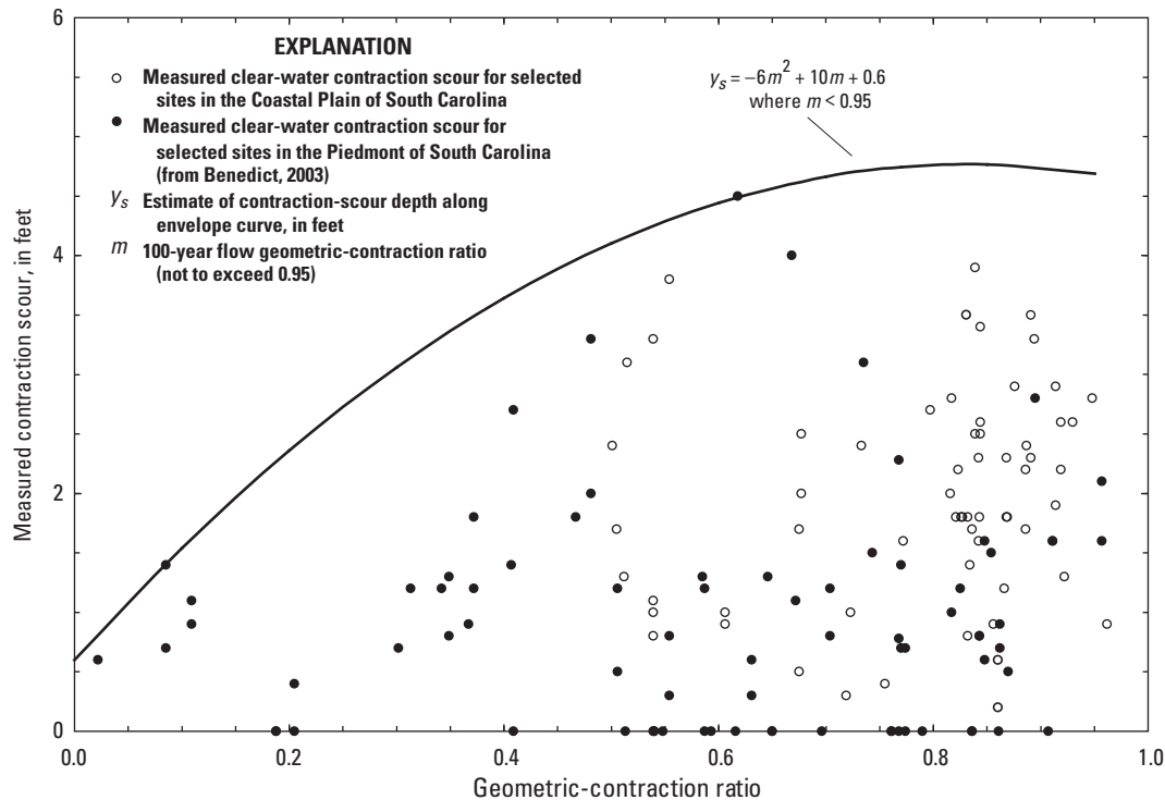
Figure 43. The South Carolina clear-water contraction-scour envelope curve for the Piedmont and Coastal Plain (from Benedict and Caldwell, 2006).
