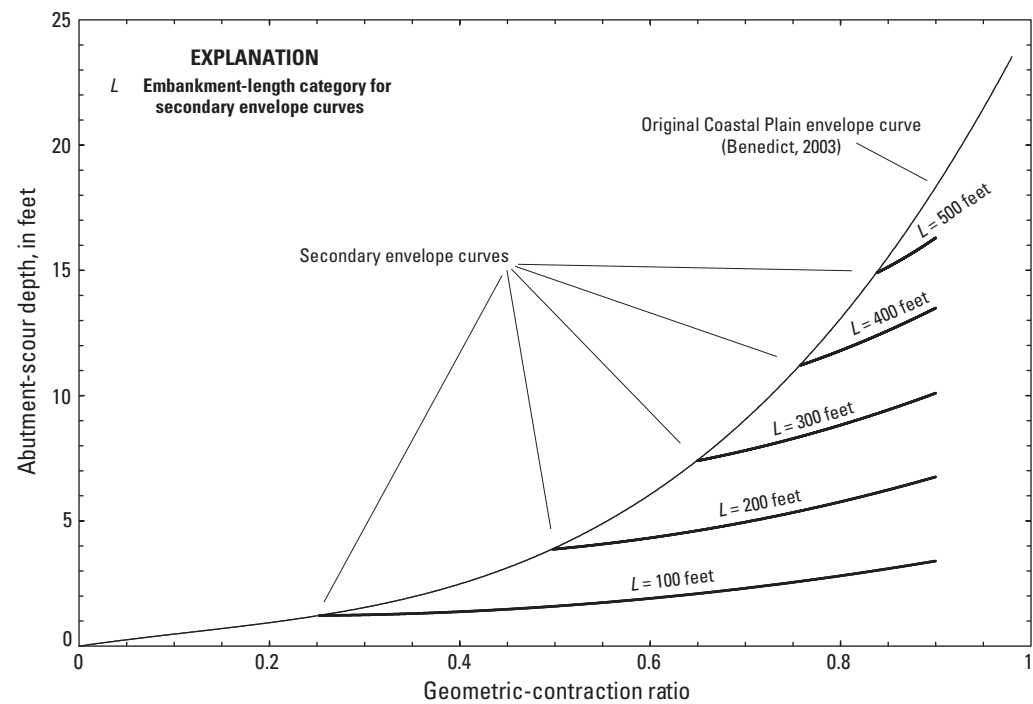
Figure 34. Relation of clear-water abutment-scour depth to the geometric-contraction ratio for selected categories of embankment lengths in the Coastal Plain of South Carolina (from Benedict and Caldwell, 2012).
