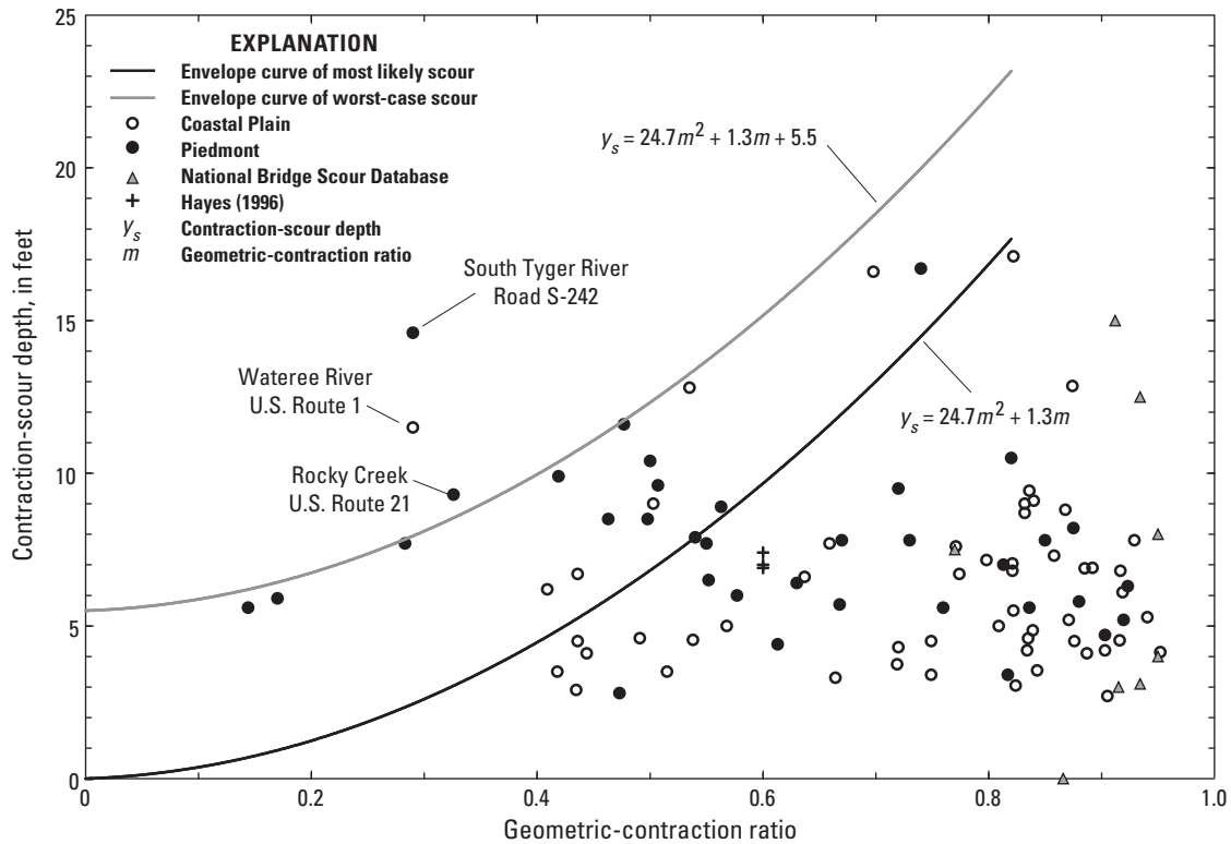
Figure 50. The South Carolina live-bed contraction-scour envelope curve for the “worst case scour” for the live-bed contraction-scour data (from Benedict and Caldwell, 2009).
