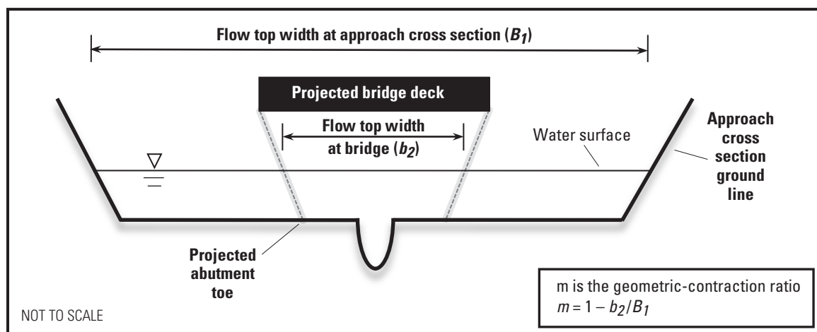
Figure 29. Definition of the geometric-contraction ratio.
