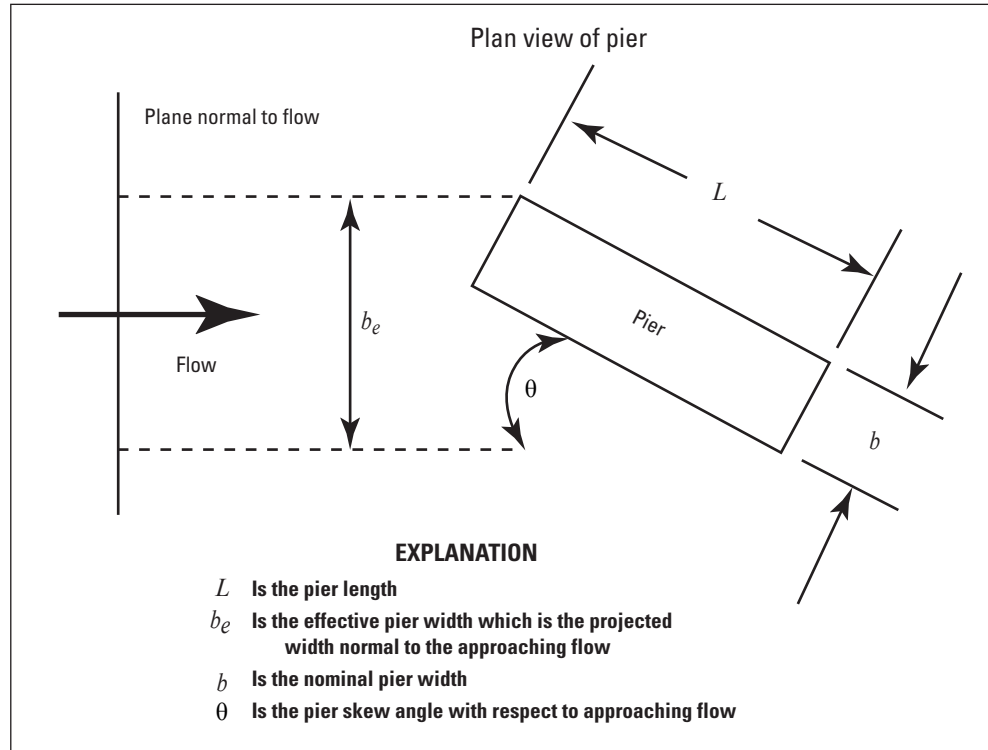
Figure 6. Definition of nominal and effective pier width (modified from Sheppard and others, 2011).
