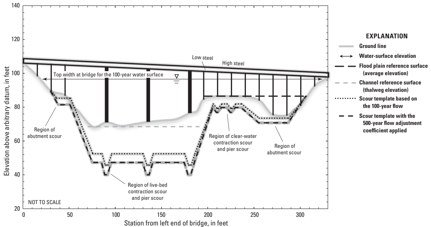
Figure 66. Region of potential scour determined from the South Carolina bridge-scour envelope curves for example 3, Enoree River at Road S-87 in Newberry County, South Carolina, with the 500-year flow adjustment coefficient applied.
