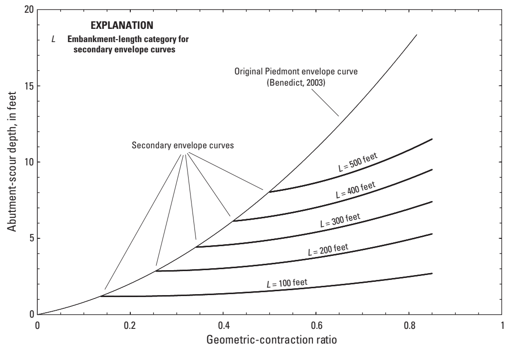
Figure 33. Relation of clear-water abutment-scour depth to the geometric-contraction ratio for selected categories of embankment lengths in the Piedmont of South Carolina (from Benedict and Caldwell, 2012).
