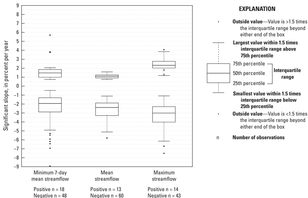
Figure 6-2. Boxplots showing slopes of significant monotonic trends in three annual streamflow metrics at water-quality sites without significant change points (alpha = 0.05) for the trend period 1982–2012. For each metric, positive slopes are summarized in the upper boxplot, and negative slopes are in the lower boxplot.
