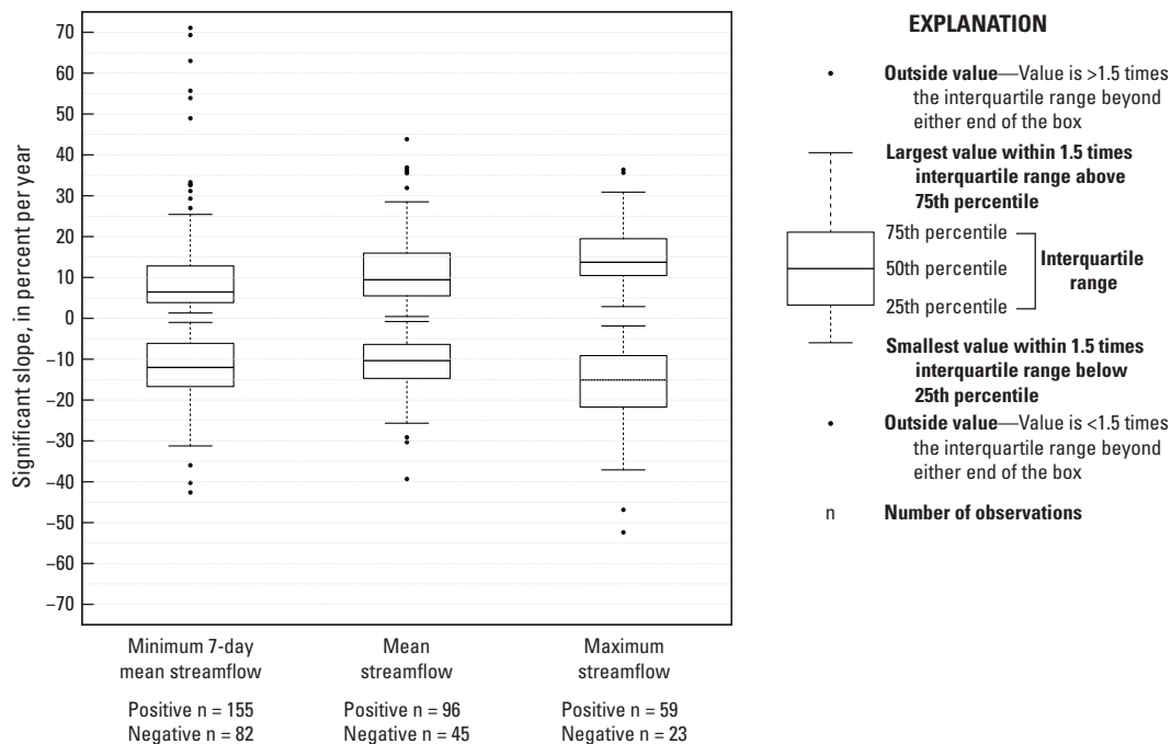
Figure 6-4. Boxplots showing slopes of significant monotonic trends in three annual streamflow metrics at water-quality sites without significant change points (alpha = 0.05) for the trend period 2002–12. For each metric, positive slopes are summarized in the upper boxplot, and negative slopes are in the lower boxplot.
