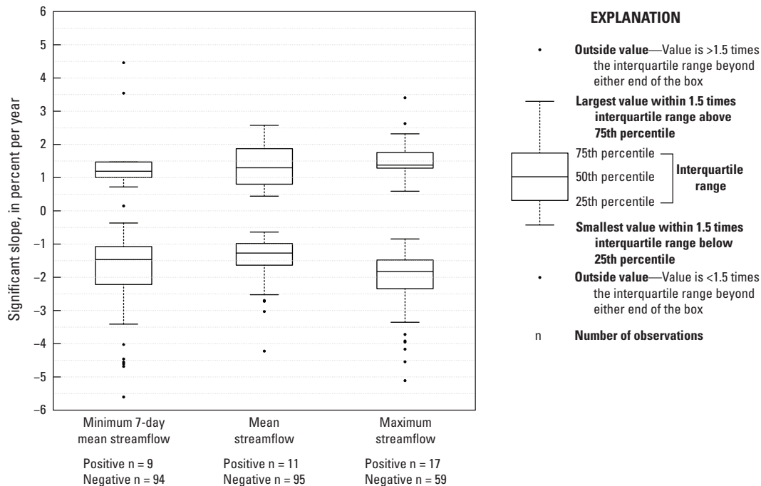
Figure 6-1. Boxplots showing slopes of significant monotonic trends in three annual streamflow metrics at water-quality sites without significant change points (alpha = 0.05) for the trend period 1972–2012. For each metric, positive slopes are summarized in the upper boxplot, and negative slopes are in the lower boxplot.
