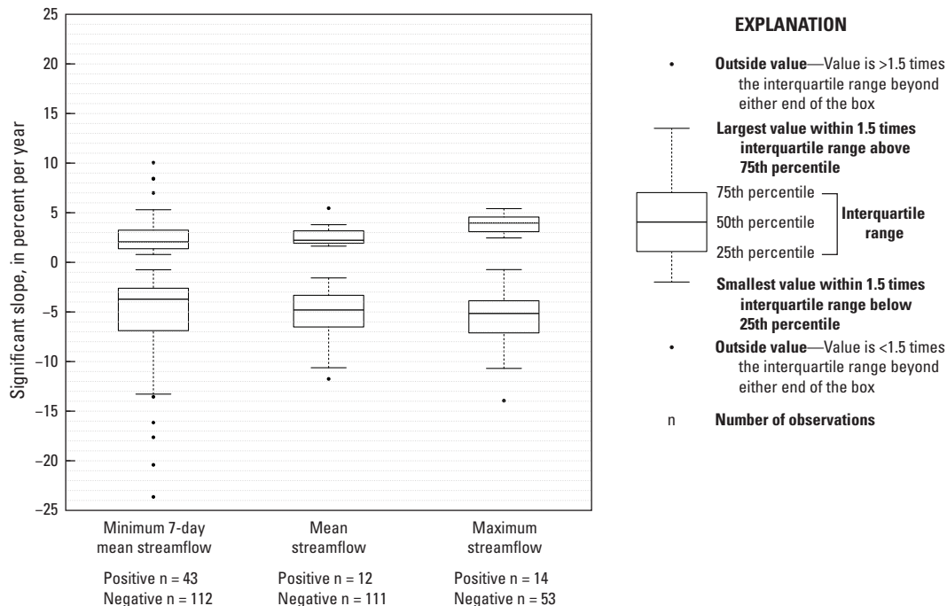
Figure 6-3. Boxplots showing slopes of significant monotonic trends in three annual streamflow metrics at water-quality sites without significant change points (alpha = 0.05) for the trend period 1992–2012. For each metric, positive slopes are summarized in the upper boxplot, and negative slopes are in the lower boxplot.
