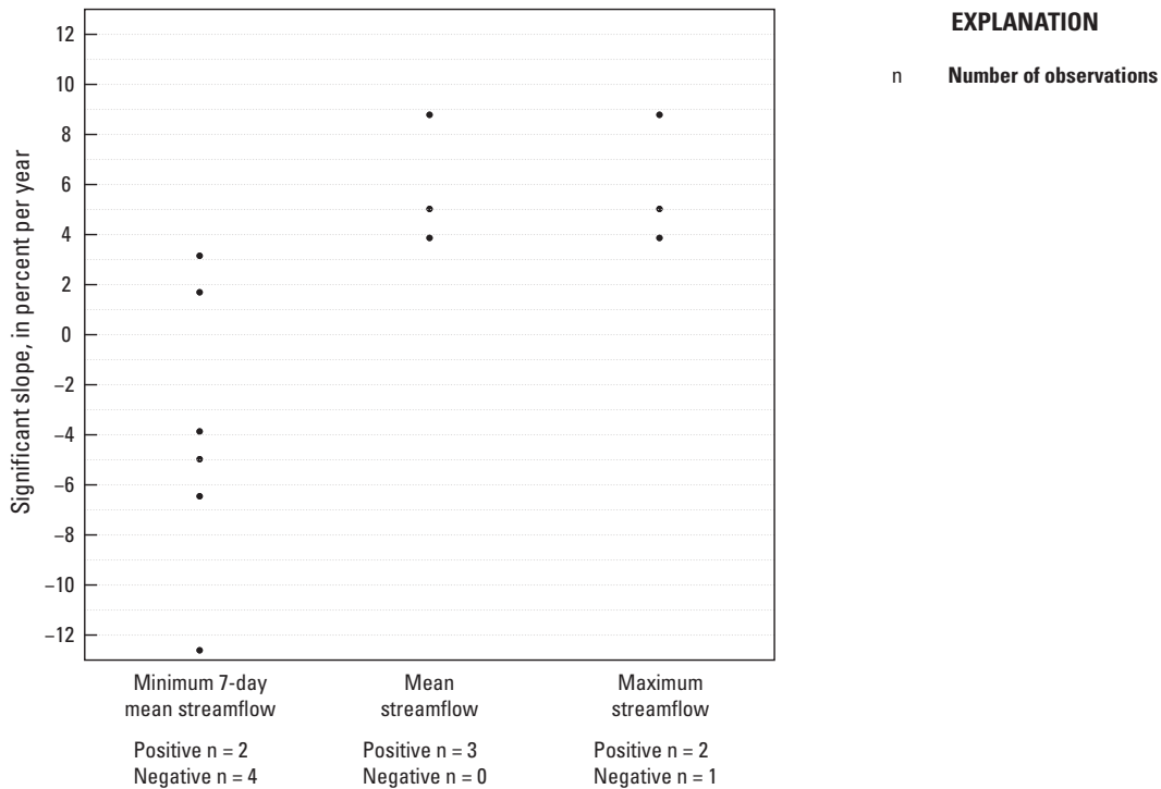
Figure 6-5. Graphs showing slopes of significant monotonic trends in three annual streamflow metrics at pesticide sites without significant change points (alpha = 0.05) for the trend period 2002–12.
