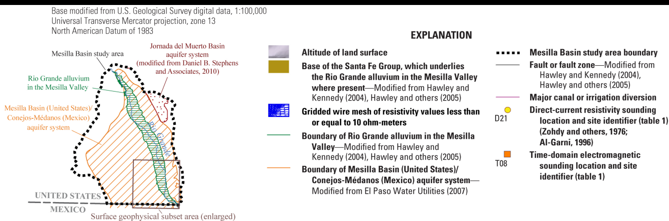
Figure 14. Three-dimensional representation of resistivity values less than or equal to 10 ohm-meters from the combined inverse modeling results of the direct-current resistivity and time-domain electromagnetic soundings in the surface geophysical subset area of the Mesilla Basin study area in Doña Ana County, New Mexico, and El Paso County, Texas.
