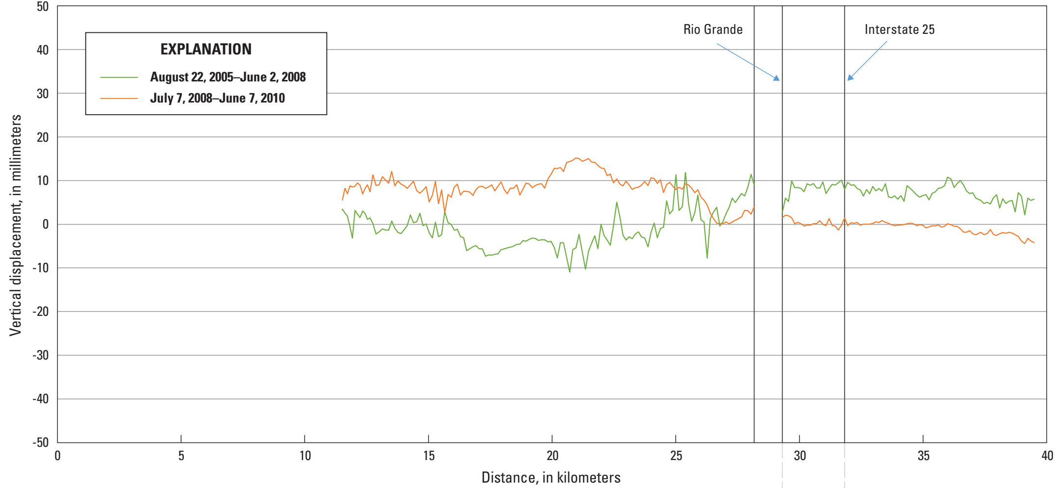
A. InSAR measured elevation change along geology profile AA-AA'
