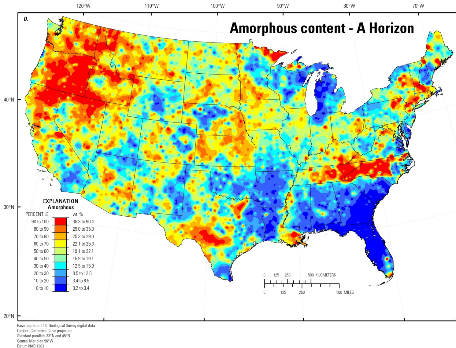
Figure 188. A, Histogram and summary statistics; B, Boxplot; C, Empirical cumulative distribution function; and D, Distribution of amorphous component in the soil A horizon, conterminous United States (LLD, lower limit of determination; wt. %, weight percent).—Continued
