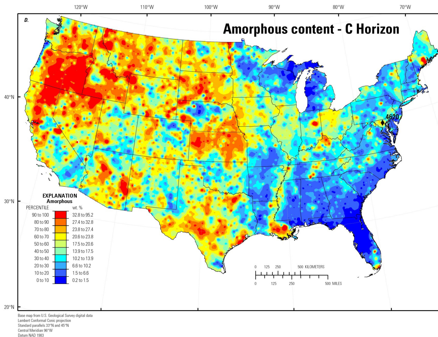
Figure 189. A, Histogram and summary statistics; B, Boxplot; C, Empirical cumulative distribution function; and D, Distribution of amorphous component in the soil C horizon, conterminous United States (LLD, lower limit of determination; wt. %, weight percent).—Continued
