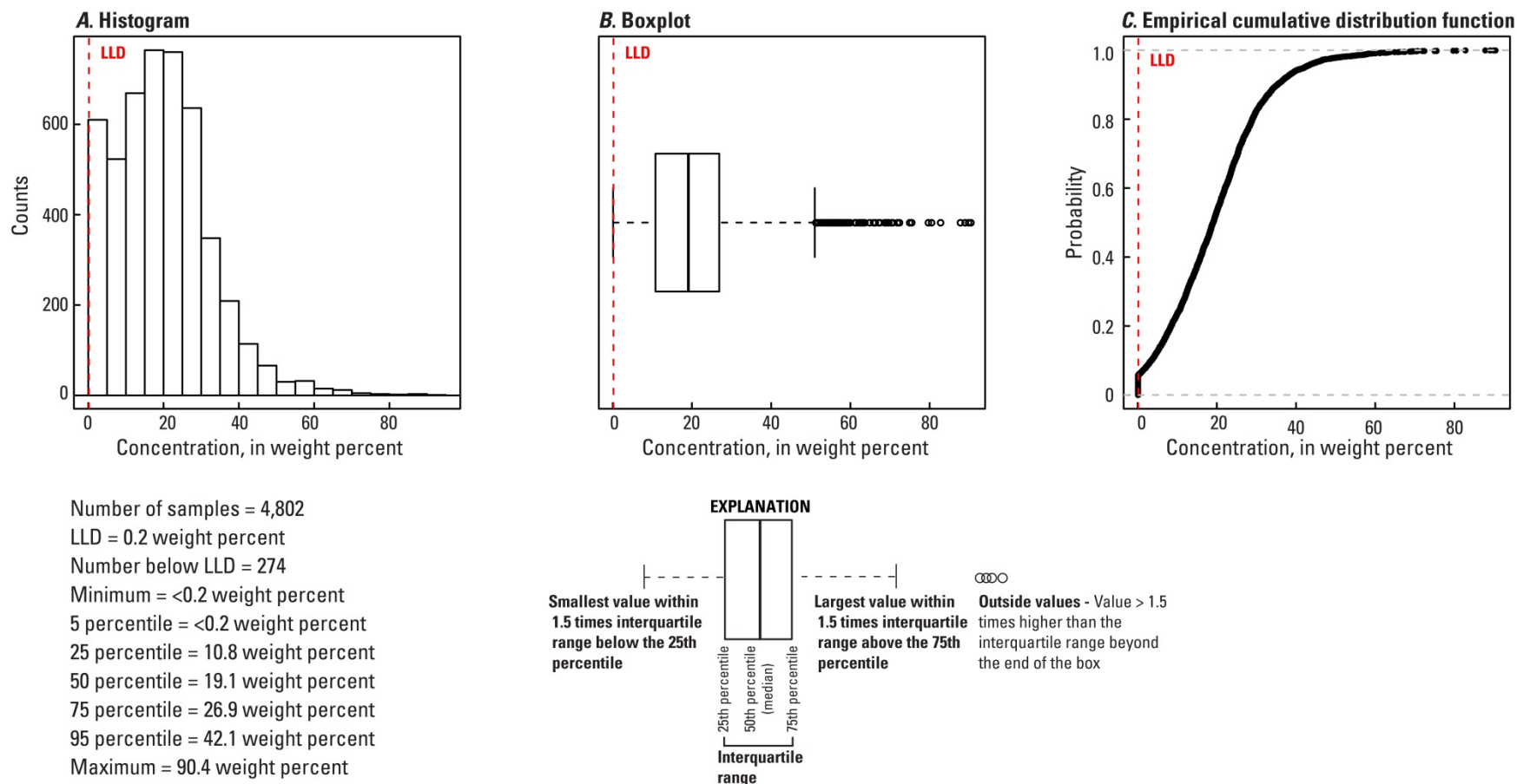
Figure 188. A, Histogram and summary statistics; B, Boxplot; C, Empirical cumulative distribution function; and D, Distribution of amorphous component in the soil A horizon, conterminous United States (LLD, lower limit of determination; wt. %, weight percent).
