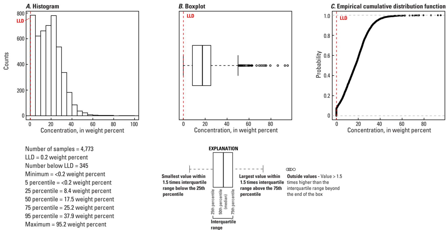
Figure 189. A, Histogram and summary statistics; B, Boxplot; C, Empirical cumulative distribution function; and D, Distribution of amorphous component in the soil C horizon, conterminous United States (LLD, lower limit of determination; wt. %, weight percent).
