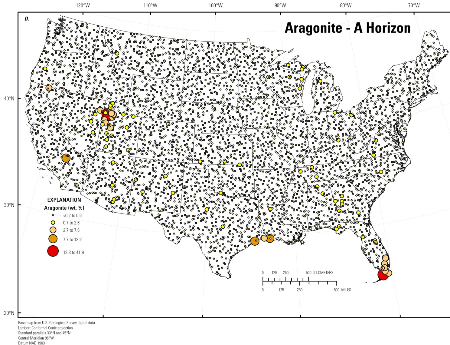
Figure 162. A, Histogram and summary statistics; B, Boxplot; C, Empirical cumulative distribution function; and D, Distribution of aragonite in the soil A horizon, conterminous United States (LLD, lower limit of determination; wt. %, weight percent).—Continued
