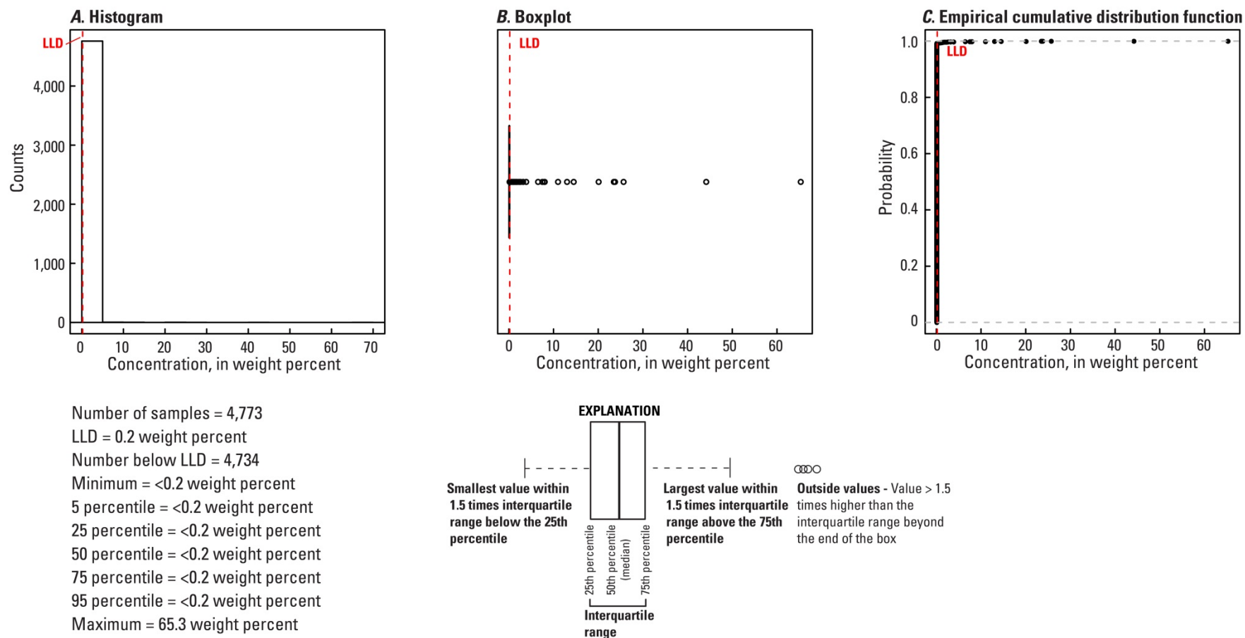
Figure 163. A, Histogram and summary statistics; B, Boxplot; C, Empirical cumulative distribution function; and D, Distribution of aragonite in the soil C horizon, conterminous United States (LLD, lower limit of determination; wt. %, weight percent).
