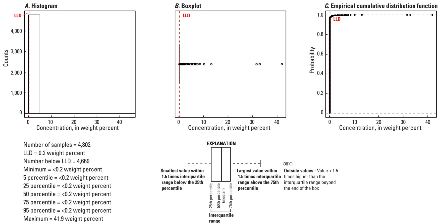
Figure 162. A, Histogram and summary statistics; B, Boxplot; C, Empirical cumulative distribution function; and D, Distribution of aragonite in the soil A horizon, conterminous United States (LLD, lower limit of determination; wt. %, weight percent).
