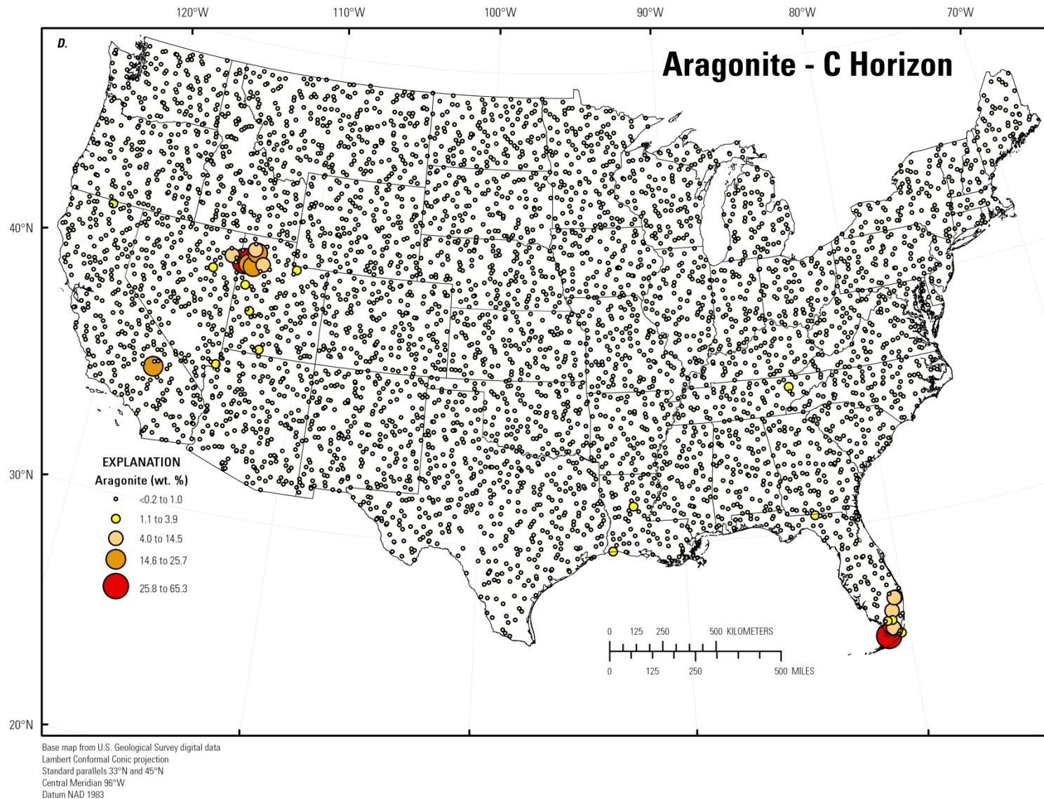
Figure 163. A, Histogram and summary statistics; B, Boxplot; C, Empirical cumulative distribution function; and D, Distribution of aragonite in the soil C horizon, conterminous United States (LLD, lower limit of determination; wt. %, weight percent).—Continued
