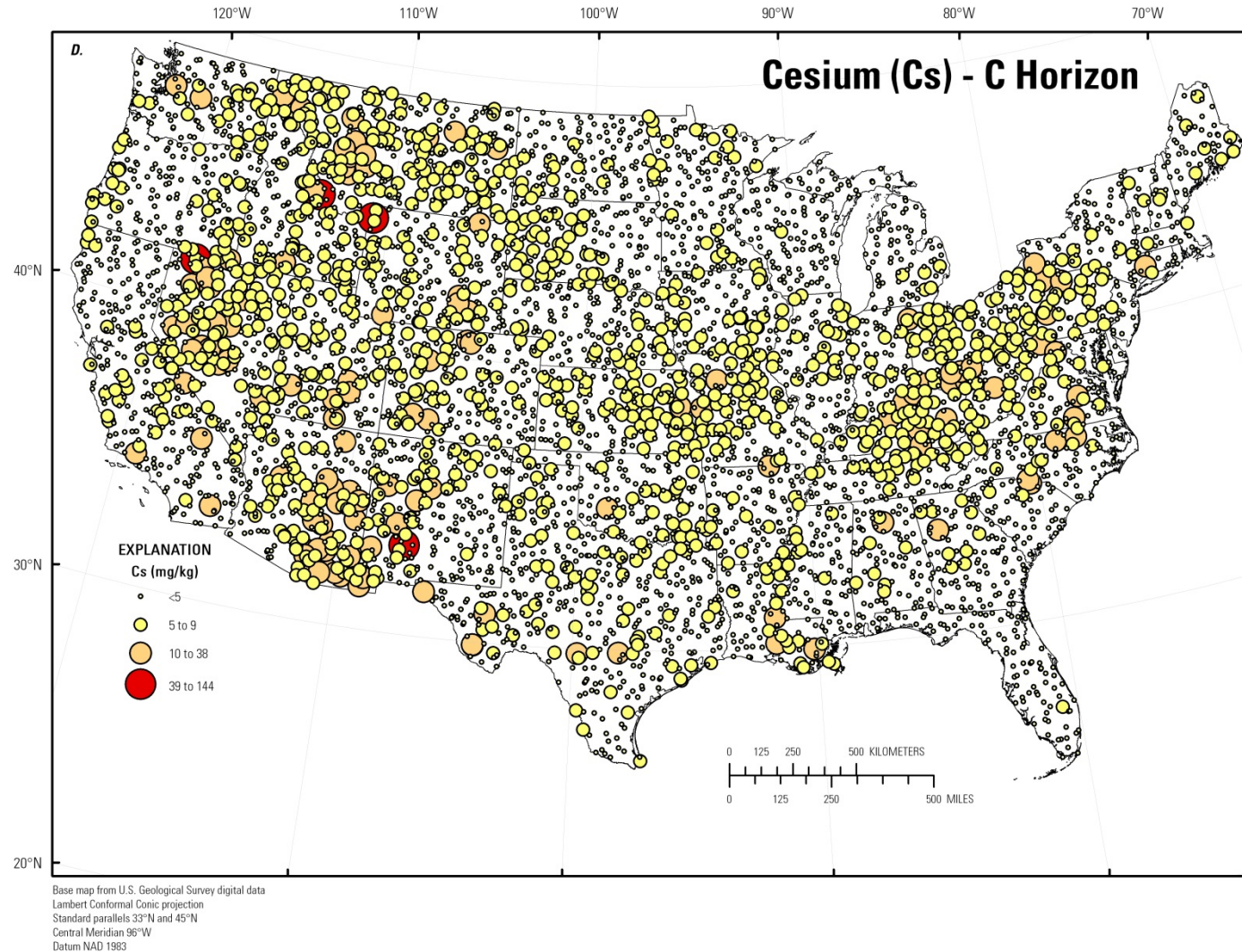
Figure 37. A, Histogram and summary statistics; B, Boxplot; C, Empirical cumulative distribution function; and D, Distribution of cesium (Cs) in the soil C horizon, conterminous United States (LLD, lower limit of determination; MAD, median absolute deviation; CV, coefficient of variation; ND, not determined; mg/kg, milligrams per kilogram).—Continued
