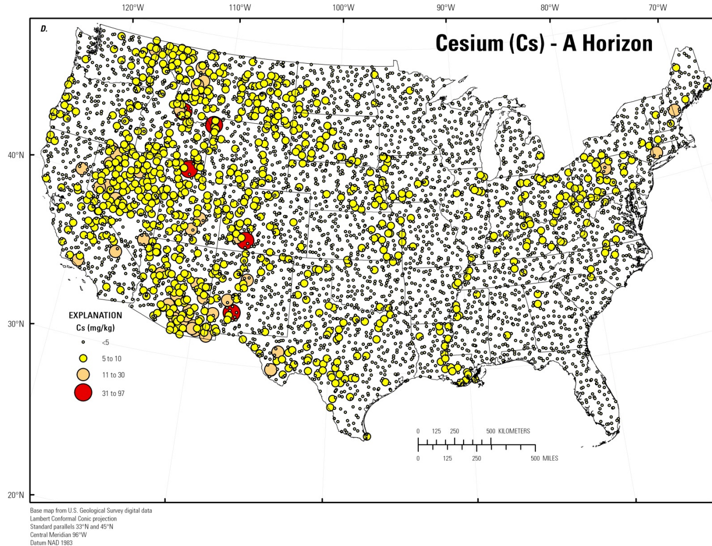
Figure 36. A, Histogram and summary statistics; B, Boxplot; C, Empirical cumulative distribution function; and D, Distribution of cesium (Cs) in the soil A horizon, conterminous United States (LLD, lower limit of determination; MAD, median absolute deviation; CV, coefficient of variation; ND, not determined; mg/kg, milligrams per kilogram).—Continued
