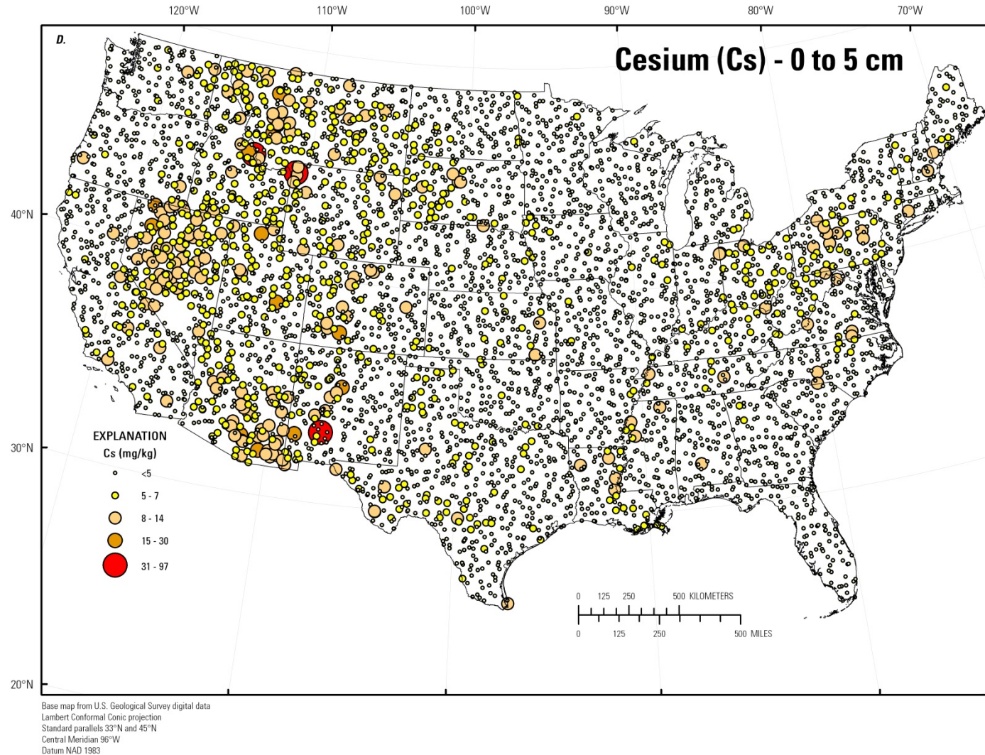
Figure 35. A, Histogram and summary statistics; B, Boxplot; C, Empirical cumulative distribution function; and D, Distribution of cesium (Cs) in surface soils collected from a depth of 0 to 5 centimeters, conterminous United States (LLD, lower limit of determination; MAD, median absolute deviation; CV, coefficient of variation; ND, not determined; mg/kg, milligrams per kilogram; cm, centimeters).—Continued
