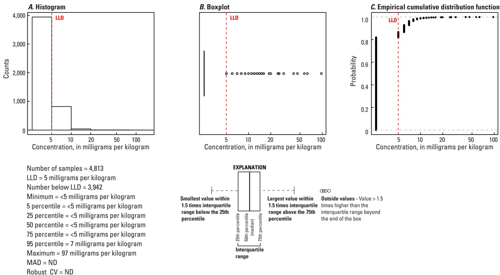
Figure 36. A, Histogram and summary statistics; B, Boxplot; C, Empirical cumulative distribution function; and D, Distribution of cesium (Cs) in the soil A horizon, conterminous United States (LLD, lower limit of determination; MAD, median absolute deviation; CV, coefficient of variation; ND, not determined; mg/kg, milligrams per kilogram).
