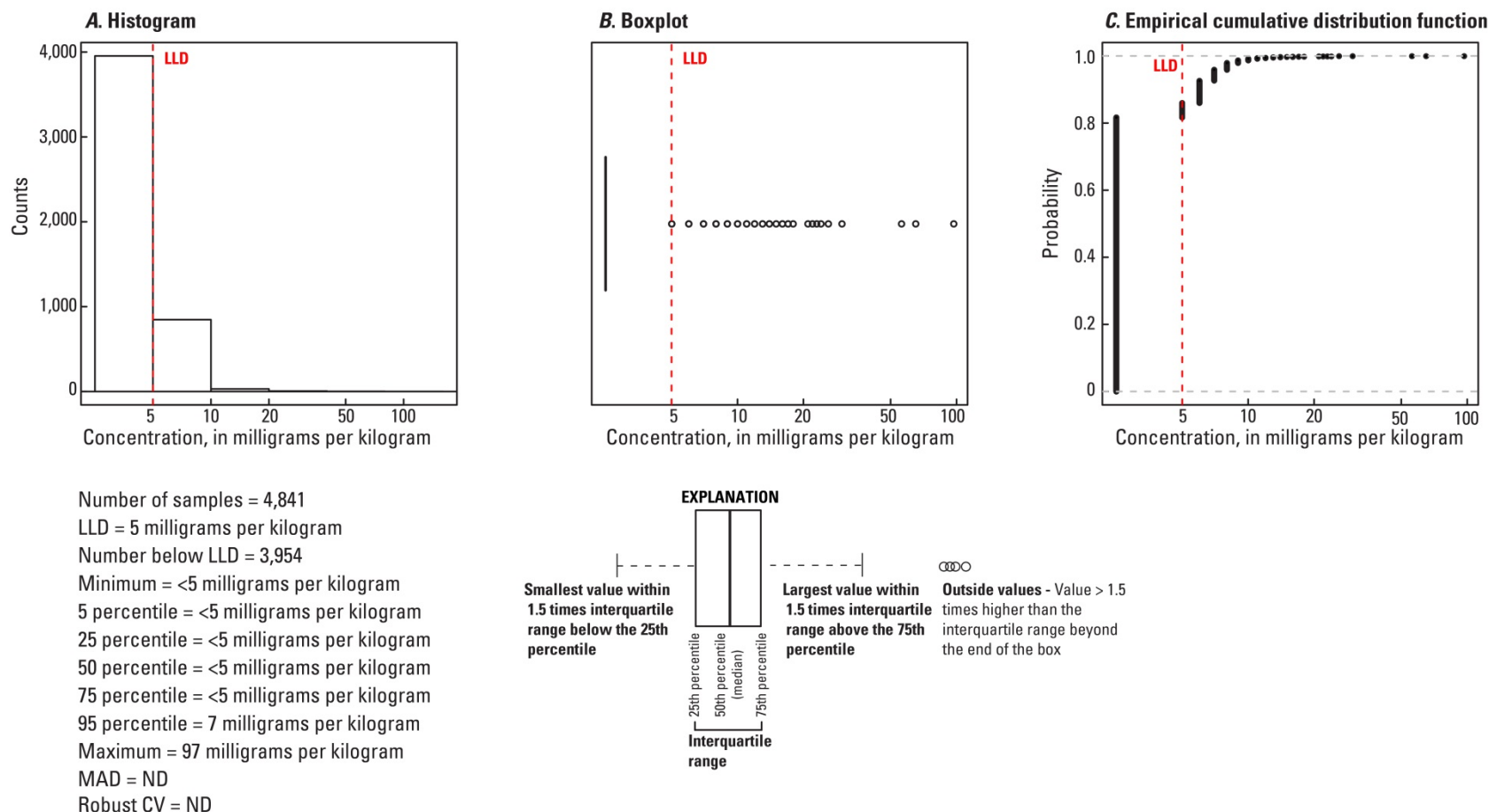
Figure 35. A, Histogram and summary statistics; B, Boxplot; C, Empirical cumulative distribution function; and D, Distribution of cesium (Cs) in surface soils collected from a depth of 0 to 5 centimeters, conterminous United States (LLD, lower limit of determination; MAD, median absolute deviation; CV, coefficient of variation; ND, not determined; mg/kg, milligrams per kilogram; cm, centimeters).
