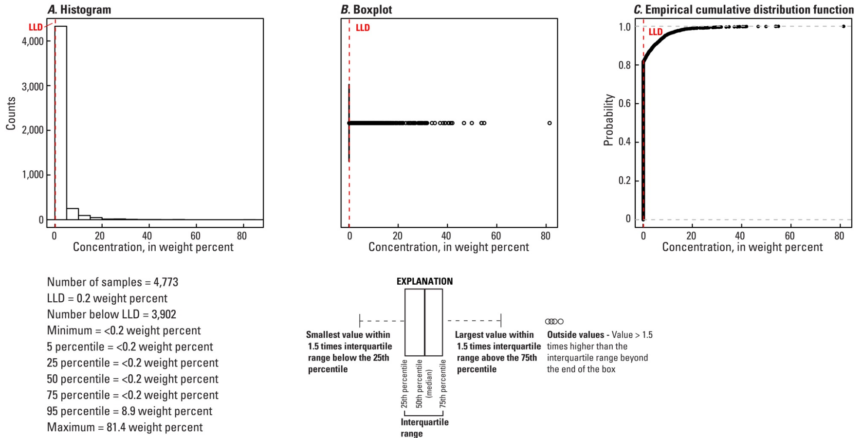
Figure 161. A, Histogram and summary statistics; B, Boxplot; C, Empirical cumulative distribution function; and D, Distribution of dolomite in the soil C horizon, conterminous United States (LLD, lower limit of determination; wt. %, weight percent).
