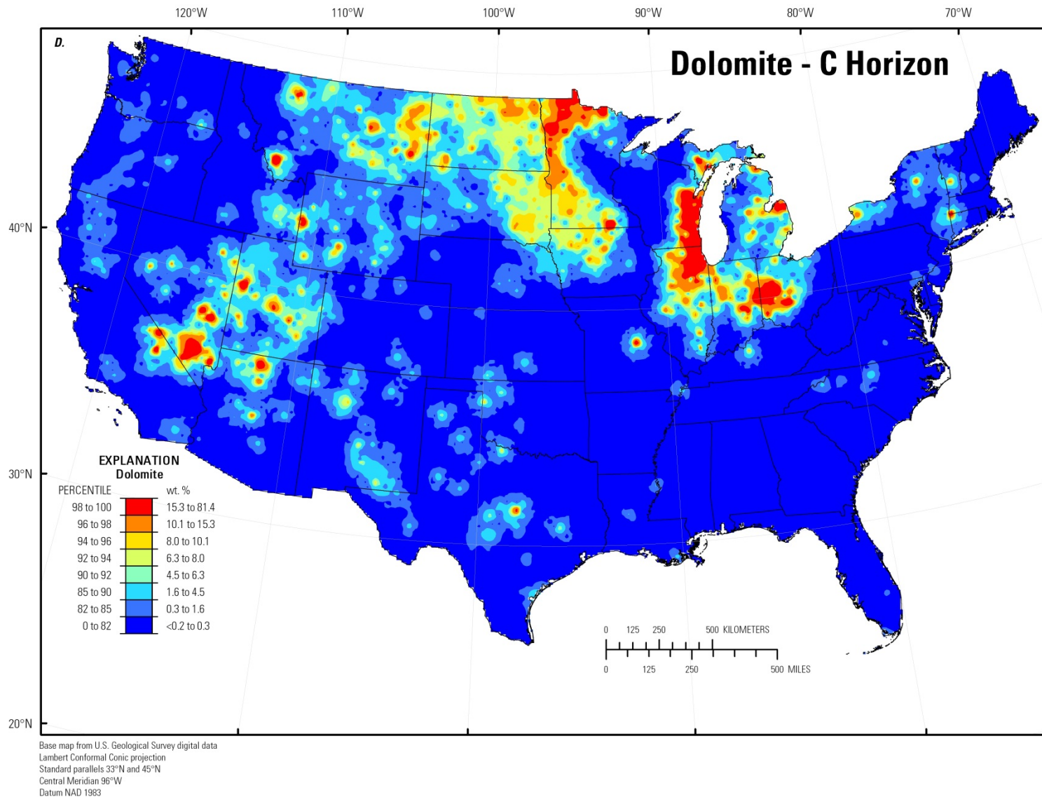
Figure 161. A, Histogram and summary statistics; B, Boxplot; C, Empirical cumulative distribution function; and D, Distribution of dolomite in the soil C horizon, conterminous United States (LLD, lower limit of determination; wt. %, weight percent).—Continued
