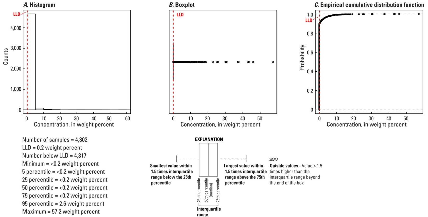
Figure 160. A, Histogram and summary statistics; B, Boxplot; C, Empirical cumulative distribution function; and D, Distribution of dolomite in the soil A horizon, conterminous United States (LLD, lower limit of determination; wt. %, weight percent).
