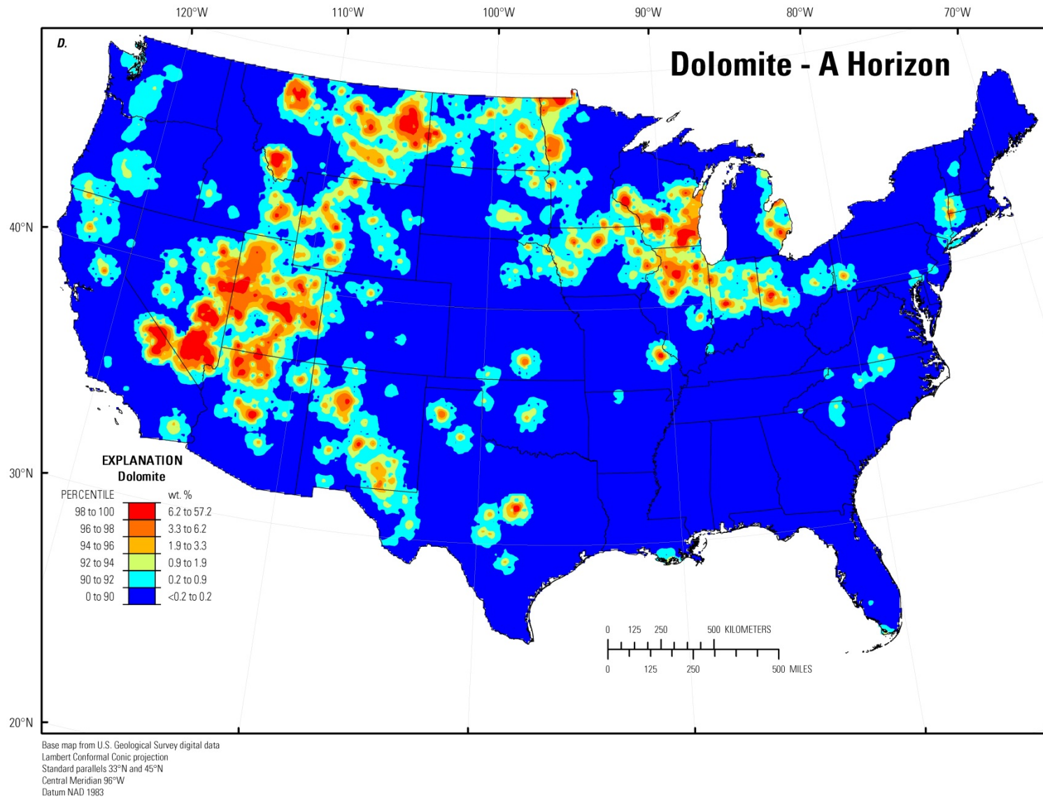
Figure 160. A, Histogram and summary statistics; B, Boxplot; C, Empirical cumulative distribution function; and D, Distribution of dolomite in the soil A horizon, conterminous United States (LLD, lower limit of determination; wt. %, weight percent).—Continued
