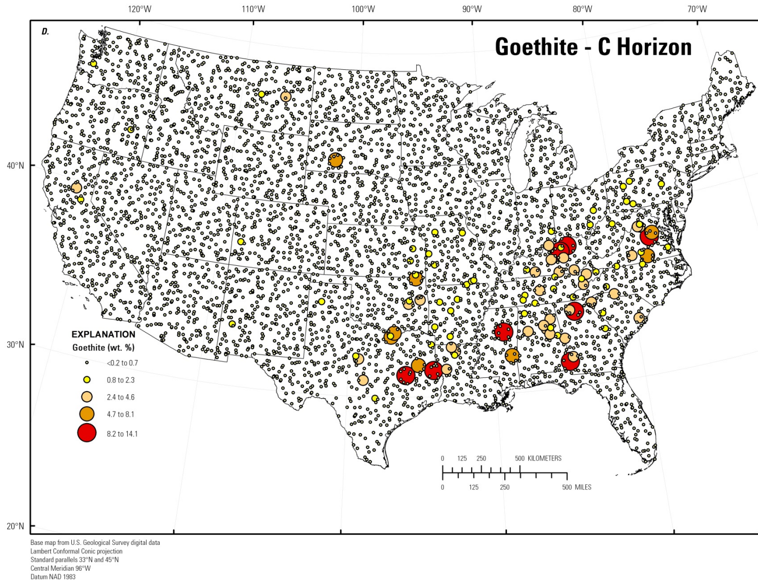
Figure 183. A, Histogram and summary statistics; B, Boxplot; C, Empirical cumulative distribution function; and D, Distribution of goethite in the soil C horizon, conterminous United States (LLD, lower limit of determination; wt. %, weight percent).—Continued
