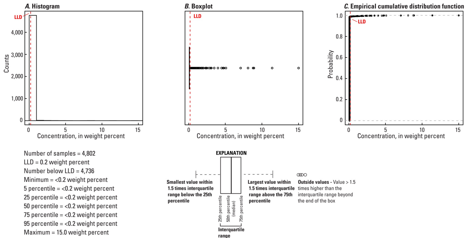
Figure 182. A, Histogram and summary statistics; B, Boxplot; C, Empirical cumulative distribution function; and D, Distribution of goethite in the soil A horizon, conterminous United States (LLD, lower limit of determination; wt. %, weight percent).
