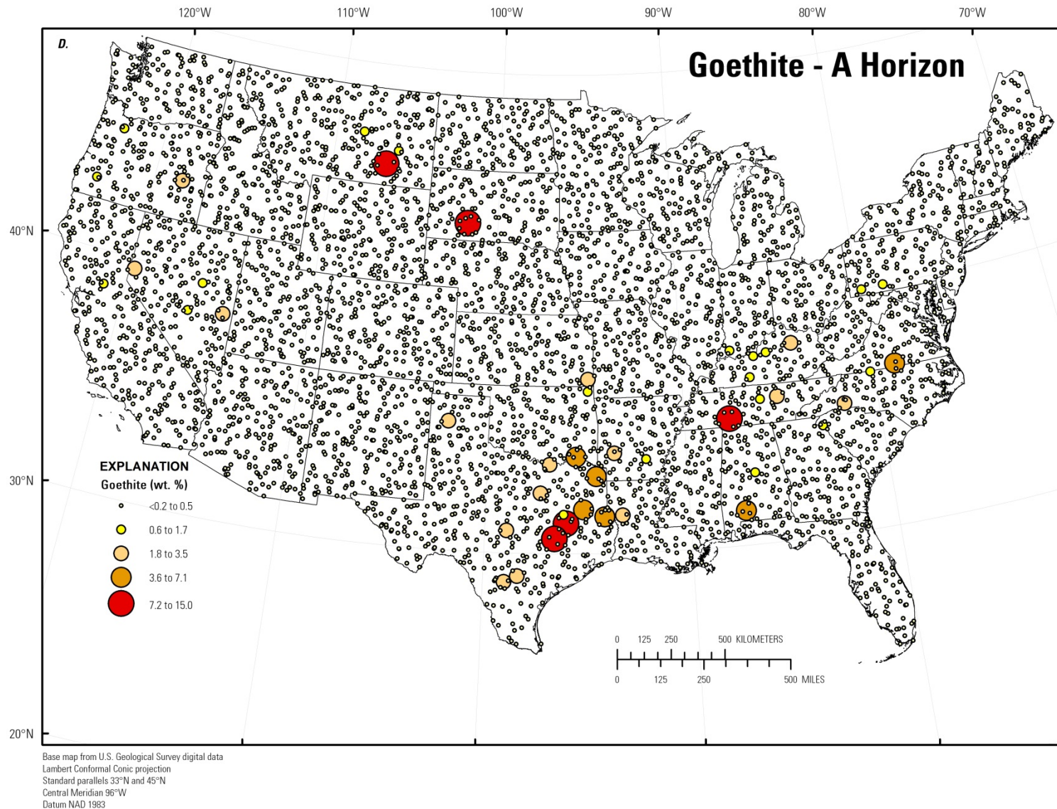
Figure 182. A, Histogram and summary statistics; B, Boxplot; C, Empirical cumulative distribution function; and D, Distribution of goethite in the soil A horizon, conterminous United States (LLD, lower limit of determination; wt. %, weight percent).—Continued
