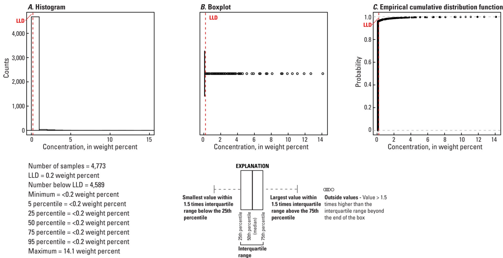
Figure 183. A, Histogram and summary statistics; B, Boxplot; C, Empirical cumulative distribution function; and D, Distribution of goethite in the soil C horizon, conterminous United States (LLD, lower limit of determination; wt. %, weight percent).
