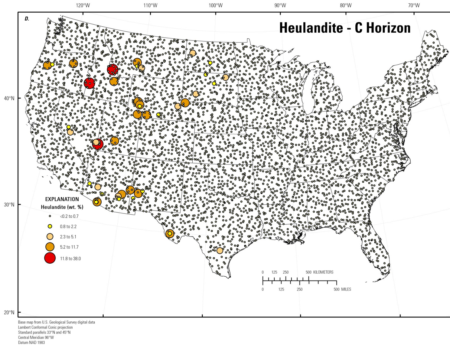
Figure 169. A, Histogram and summary statistics; B, Boxplot; C, Empirical cumulative distribution function; and D, Distribution of heulandite in the soil C horizon, conterminous United States (LLD, lower limit of determination; wt. %, weight percent).—Continued
