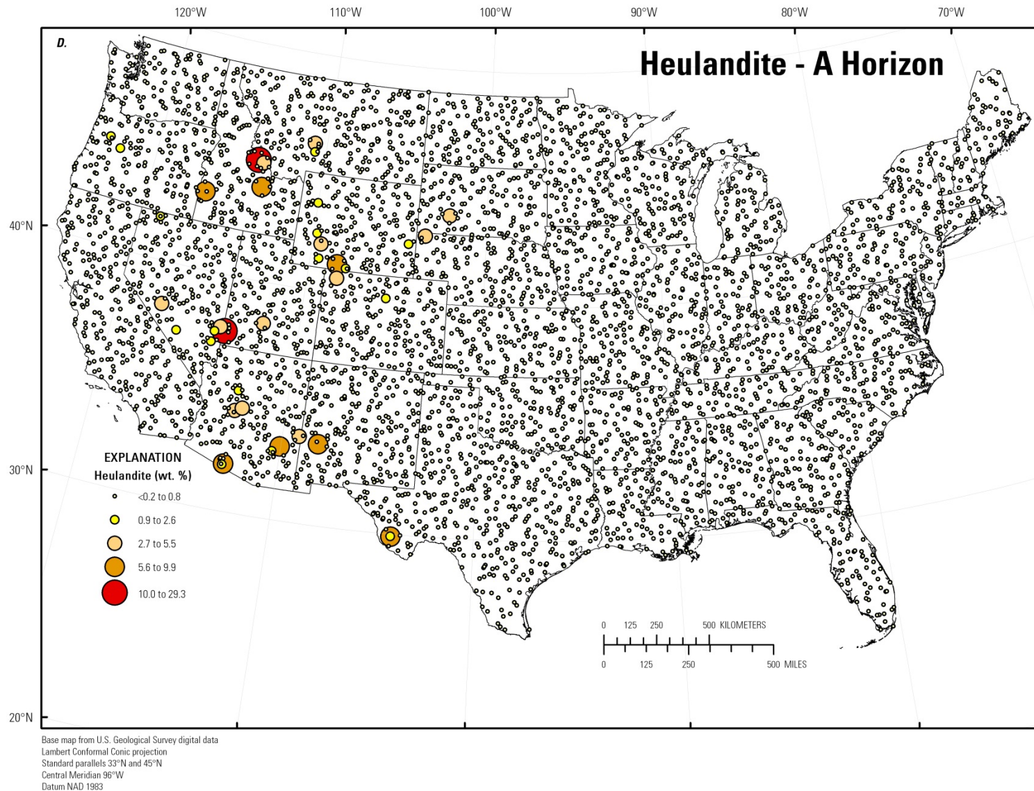
Figure 168. A, Histogram and summary statistics; B, Boxplot; C, Empirical cumulative distribution function; and D, Distribution of heulandite in the soil A horizon, conterminous United States (LLD, lower limit of determination; wt. %, weight percent).—Continued
