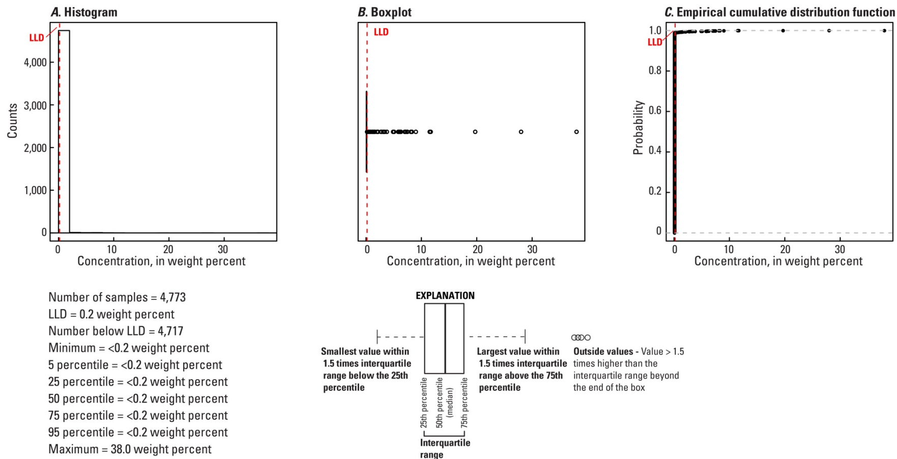
Figure 169. A, Histogram and summary statistics; B, Boxplot; C, Empirical cumulative distribution function; and D, Distribution of heulandite in the soil C horizon, conterminous United States (LLD, lower limit of determination; wt. %, weight percent).
