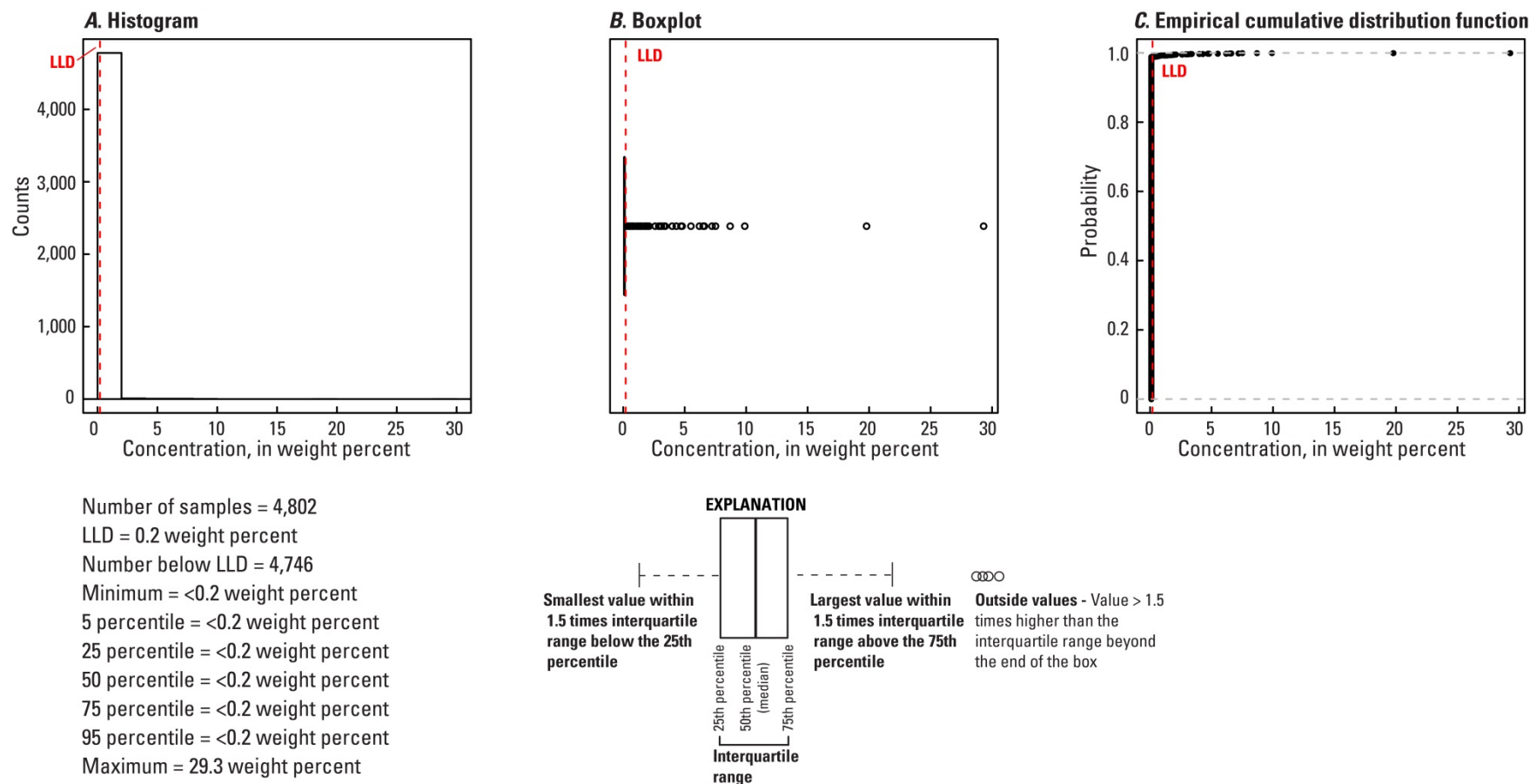
Figure 168. A, Histogram and summary statistics; B, Boxplot; C, Empirical cumulative distribution function; and D, Distribution of heulandite in the soil A horizon, conterminous United States (LLD, lower limit of determination; wt. %, weight percent).
