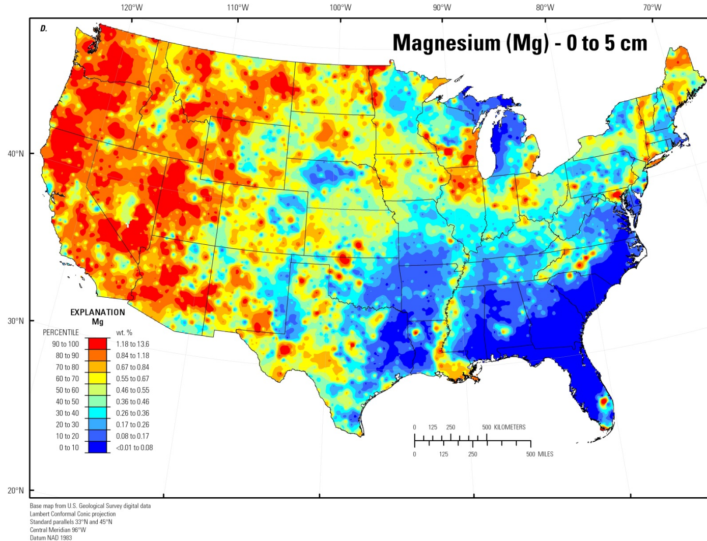
Figure 65. A, Histogram and summary statistics; B, Boxplot; C, Empirical cumulative distribution function; and D, Distribution of magnesium (Mg) in surface soils collected from a depth of 0 to 5 centimeters, conterminous United States (LLD, lower limit of determination; MAD, median absolute deviation; CV, coefficient of variation; wt. %, weight percent; cm, centimeters).—Continued
