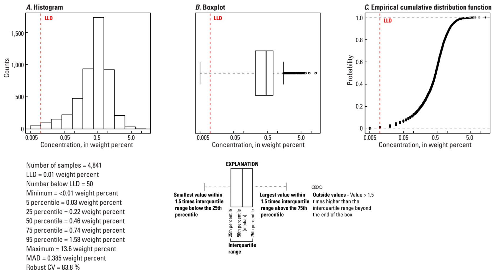
Figure 65. A, Histogram and summary statistics; B, Boxplot; C, Empirical cumulative distribution function; and D, Distribution of magnesium (Mg) in surface soils collected from a depth of 0 to 5 centimeters, conterminous United States (LLD, lower limit of determination; MAD, median absolute deviation; CV, coefficient of variation; wt. %, weight percent; cm, centimeters).
