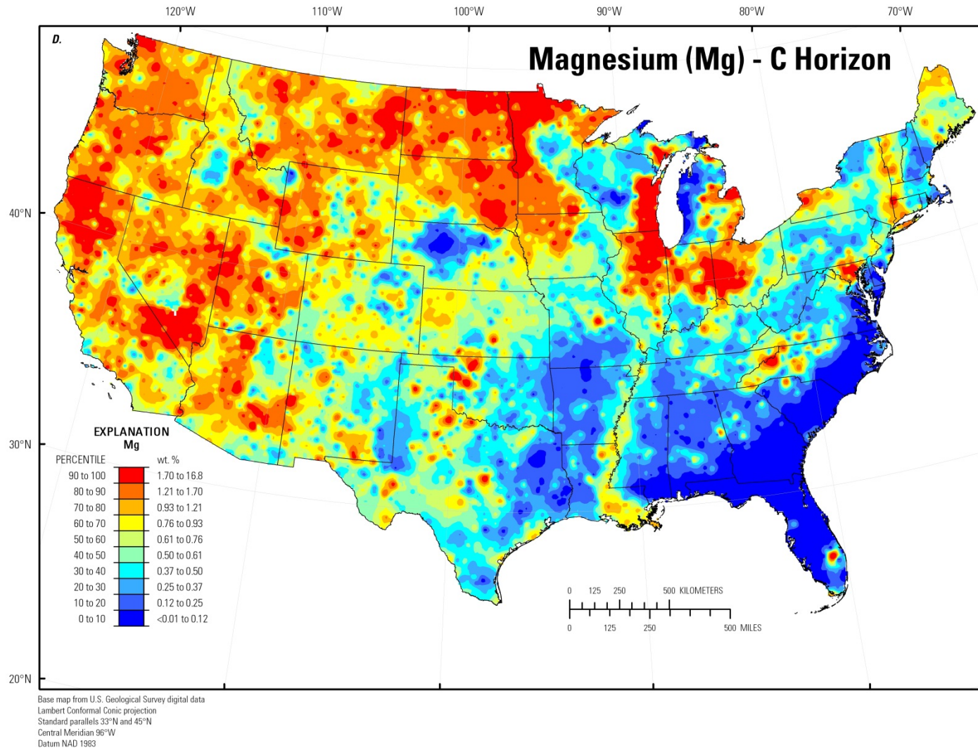
Figure 67. A, Histogram and summary statistics; B, Boxplot; C, Empirical cumulative distribution function; and D, Distribution of magnesium (Mg) in the soil C horizon, conterminous United States (LLD, lower limit of determination; MAD, median absolute deviation; CV, coefficient of variation; wt. %, weight percent).—Continued
