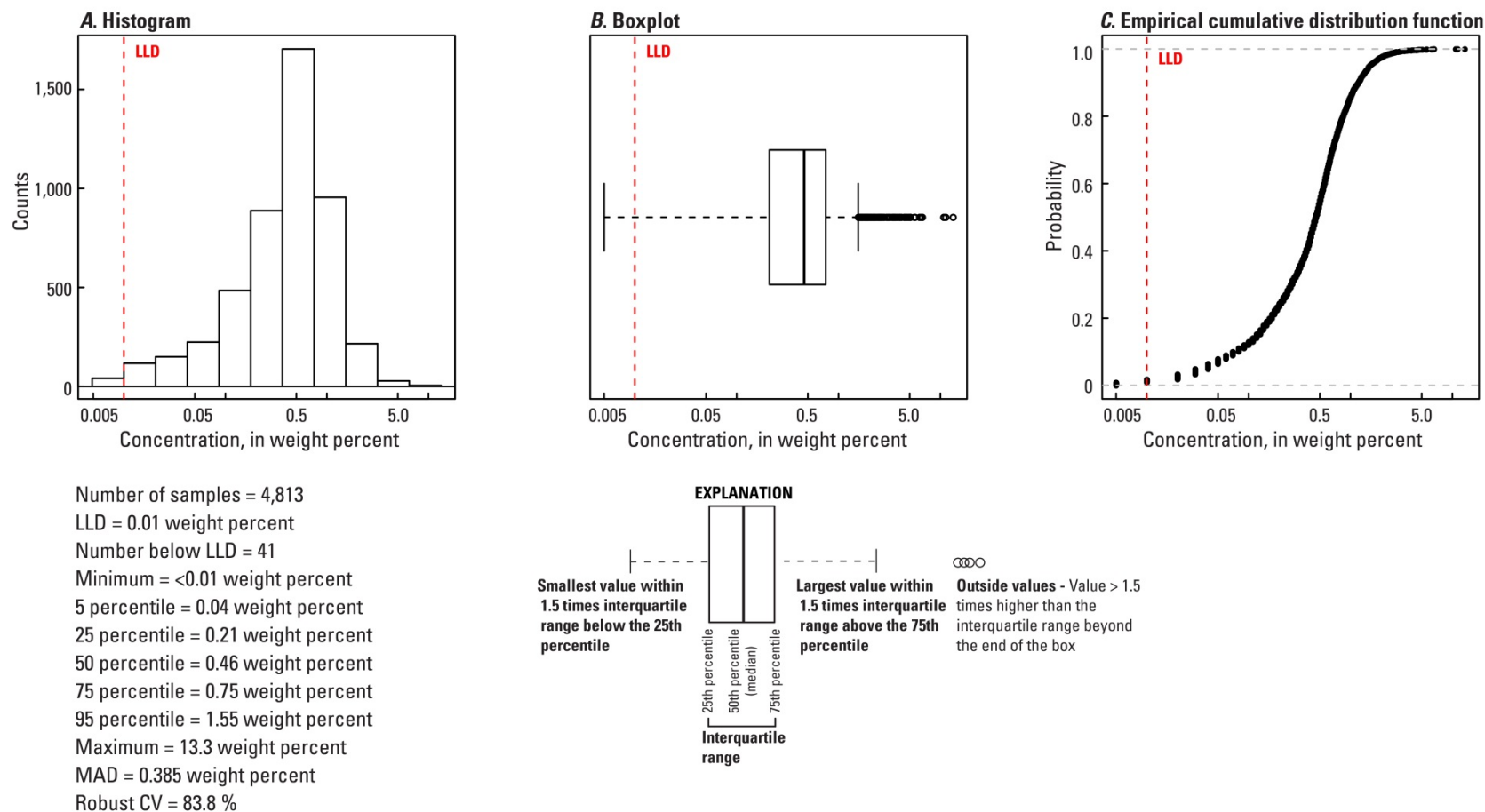
Figure 66. A, Histogram and summary statistics; B, Boxplot; C, Empirical cumulative distribution function; and D, Distribution of magnesium (Mg) in the soil A horizon, conterminous United States (LLD, lower limit of determination; MAD, median absolute deviation; CV, coefficient of variation; wt. %, weight percent).
