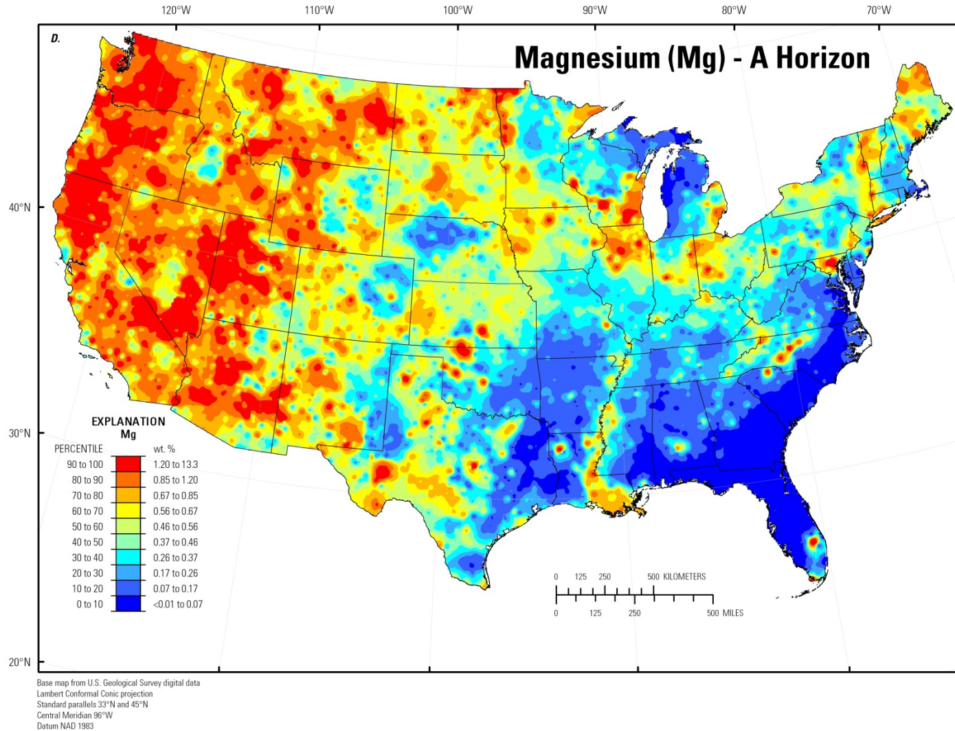
Figure 66. A, Histogram and summary statistics; B, Boxplot; C, Empirical cumulative distribution function; and D, Distribution of magnesium (Mg) in the soil A horizon, conterminous United States (LLD, lower limit of determination; MAD, median absolute deviation; CV, coefficient of variation; wt. %, weight percent).—Continued
