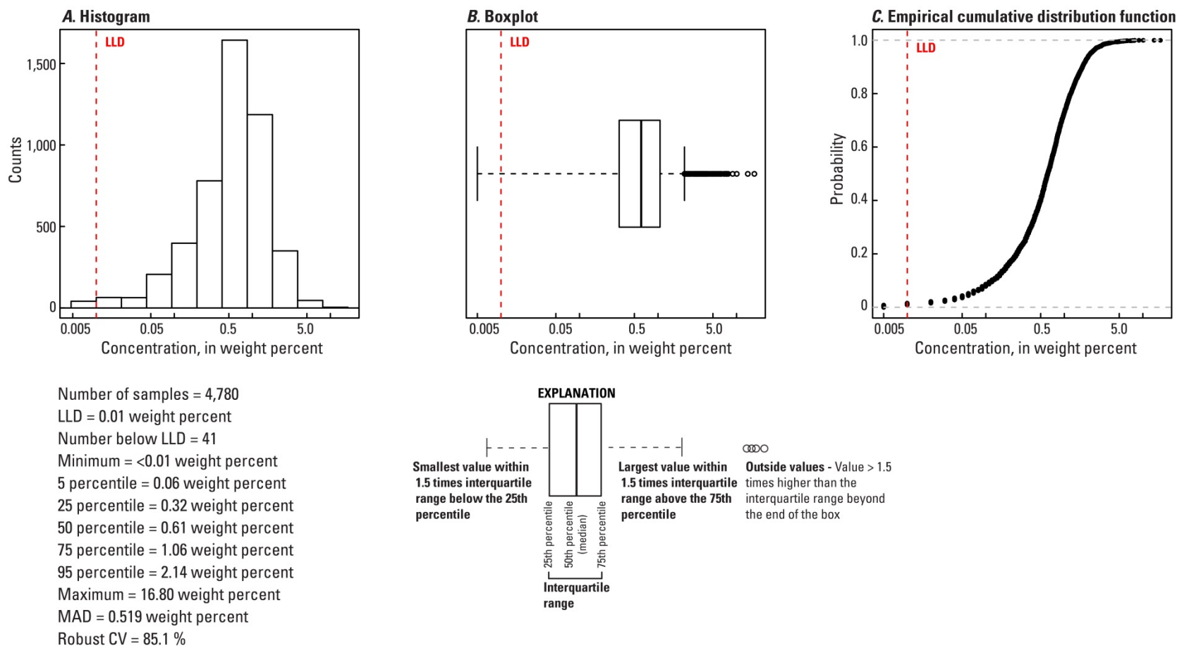
Figure 67. A, Histogram and summary statistics; B, Boxplot; C, Empirical cumulative distribution function; and D, Distribution of magnesium (Mg) in the soil C horizon, conterminous United States (LLD, lower limit of determination; MAD, median absolute deviation; CV, coefficient of variation; wt. %, weight percent).
