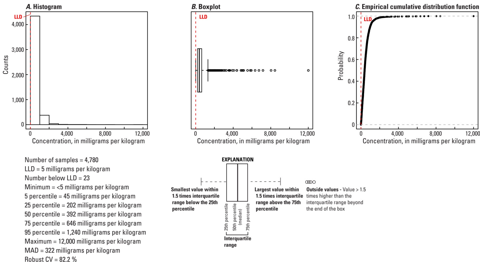
Figure 70. A, Histogram and summary statistics; B, Boxplot; C, Empirical cumulative distribution function; and D, Distribution of manganese (Mn) in the soil C horizon, conterminous United States (LLD, lower limit of determination; MAD, median absolute deviation; CV, coefficient of variation; mg/kg, milligrams per kilogram).
