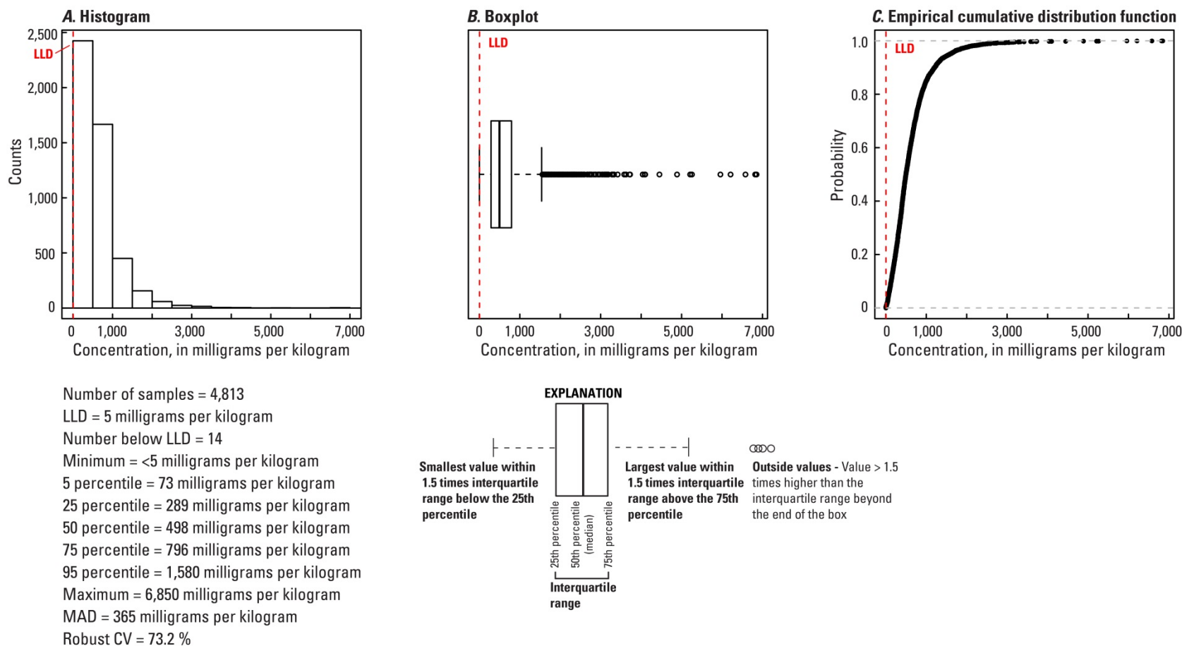
Figure 69. A, Histogram and summary statistics; B, Boxplot; C, Empirical cumulative distribution function; and D, Distribution of manganese (Mn) in the soil A horizon, conterminous United States (LLD, lower limit of determination; MAD, median absolute deviation; CV, coefficient of variation; mg/kg, milligrams per kilogram).
