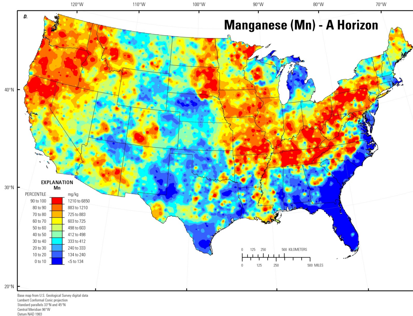
Figure 69. A, Histogram and summary statistics; B, Boxplot; C, Empirical cumulative distribution function; and D, Distribution of manganese (Mn) in the soil A horizon, conterminous United States (LLD, lower limit of determination; MAD, median absolute deviation; CV, coefficient of variation; mg/kg, milligrams per kilogram).—Continued
