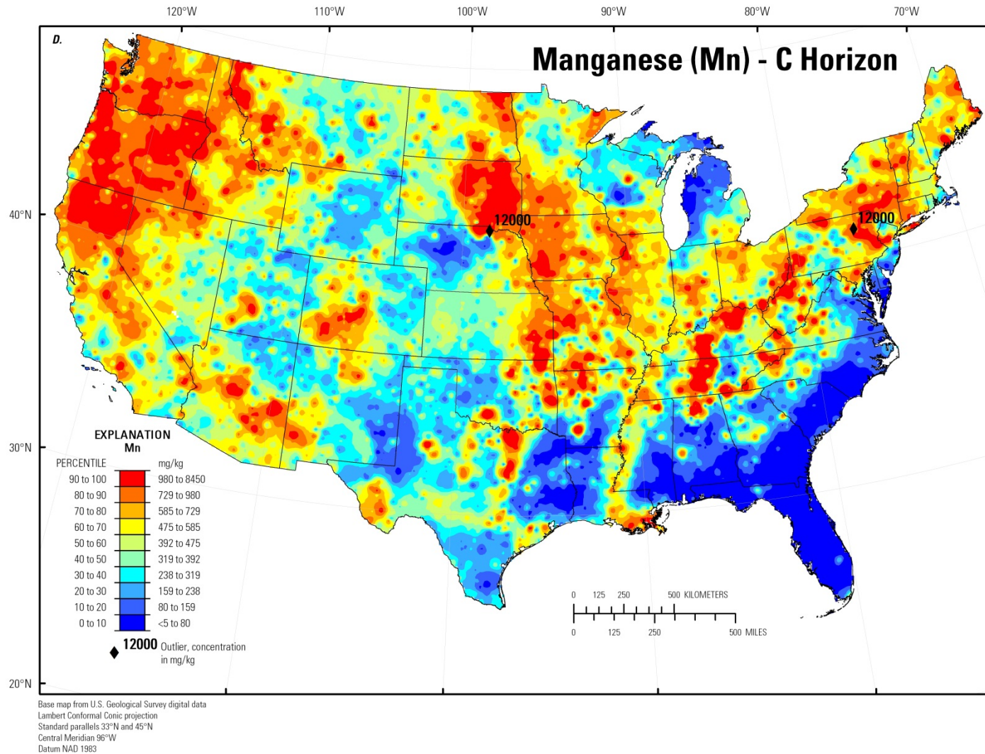
Figure 70. A, Histogram and summary statistics; B, Boxplot; C, Empirical cumulative distribution function; and D, Distribution of manganese (Mn) in the soil C horizon, conterminous United States (LLD, lower limit of determination; MAD, median absolute deviation; CV, coefficient of variation; mg/kg, milligrams per kilogram).—Continued
