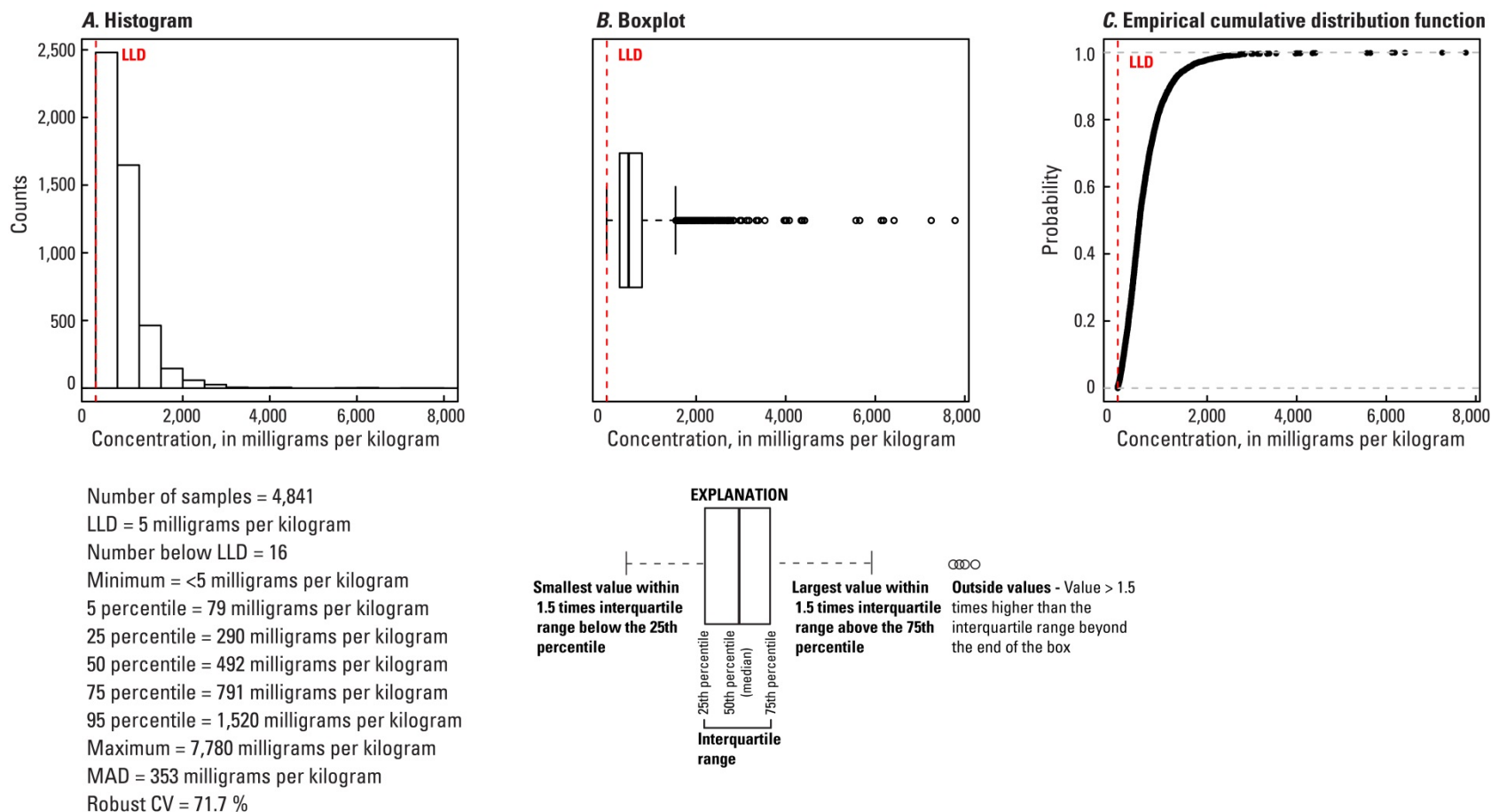
Figure 68. A, Histogram and summary statistics; B, Boxplot; C, Empirical cumulative distribution function; and D, Distribution of manganese (Mn) in surface soils collected from a depth of 0 to 5 centimeters, conterminous United States (LLD, lower limit of determination; MAD, median absolute deviation; CV, coefficient of variation; mg/kg, milligrams per kilogram; cm, centimeters).
