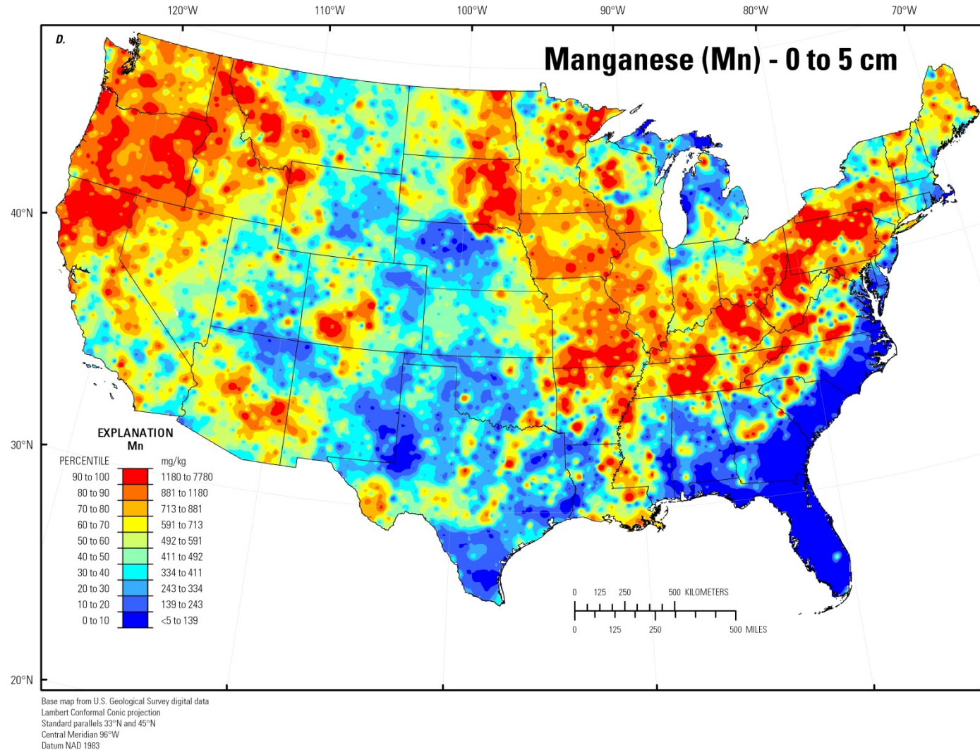
Figure 68. A, Histogram and summary statistics; B, Boxplot; C, Empirical cumulative distribution function; and D, Distribution of manganese (Mn) in surface soils collected from a depth of 0 to 5 centimeters, conterminous United States (LLD, lower limit of determination; MAD, median absolute deviation; CV, coefficient of variation; mg/kg, milligrams per kilogram; cm, centimeters).—Continued
