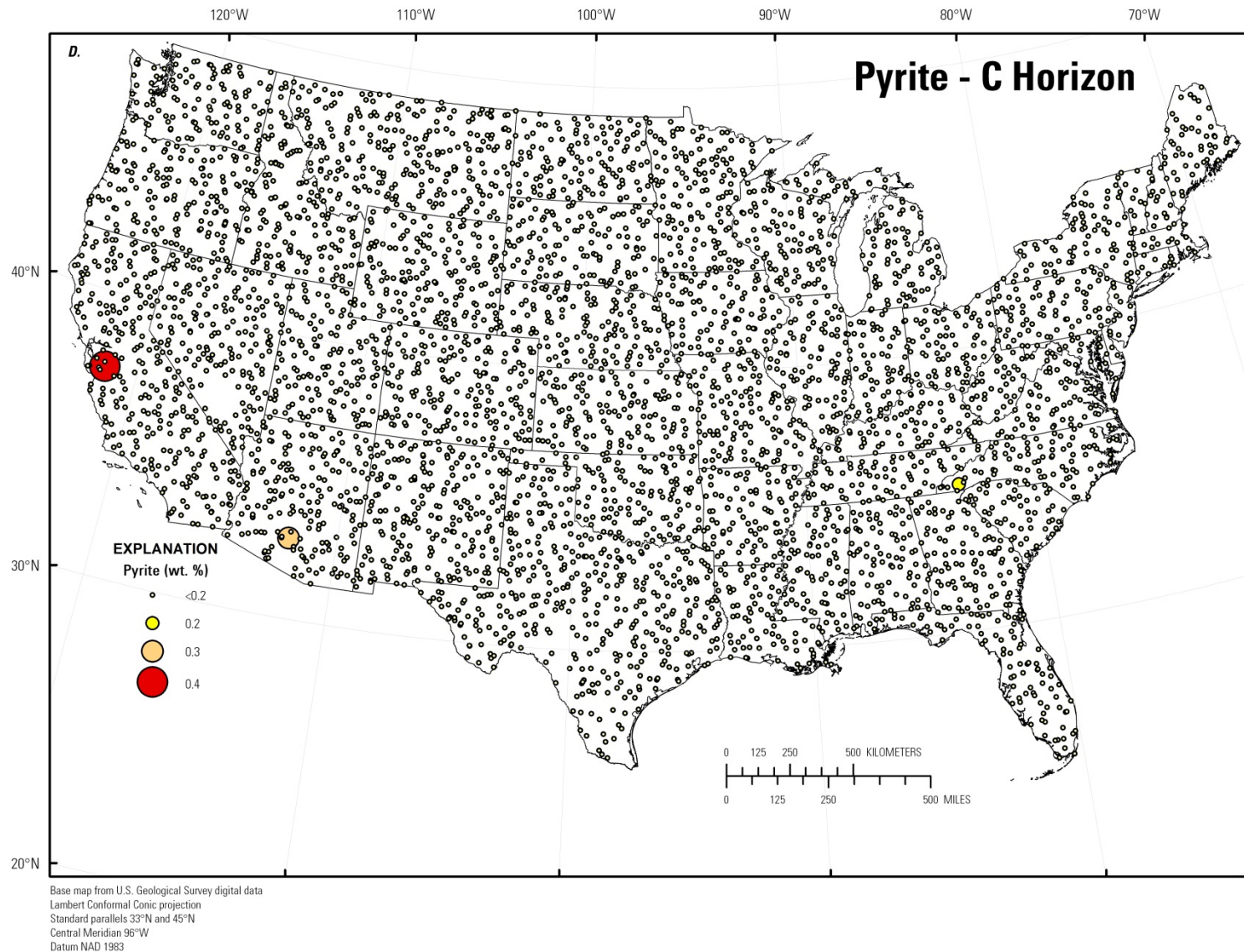
Figure 187. A, Histogram and summary statistics; B, Boxplot; C, Empirical cumulative distribution function; and D, Distribution of pyrite in the soil C horizon, conterminous United States (LLD, lower limit of determination; wt. %, weight percent).—Continued
