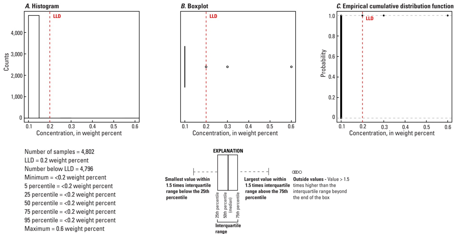
Figure 186. A, Histogram and summary statistics; B, Boxplot; C, Empirical cumulative distribution function; and D, Distribution of pyrite in the soil A horizon, conterminous United States (LLD, lower limit of determination; wt. %, weight percent).
