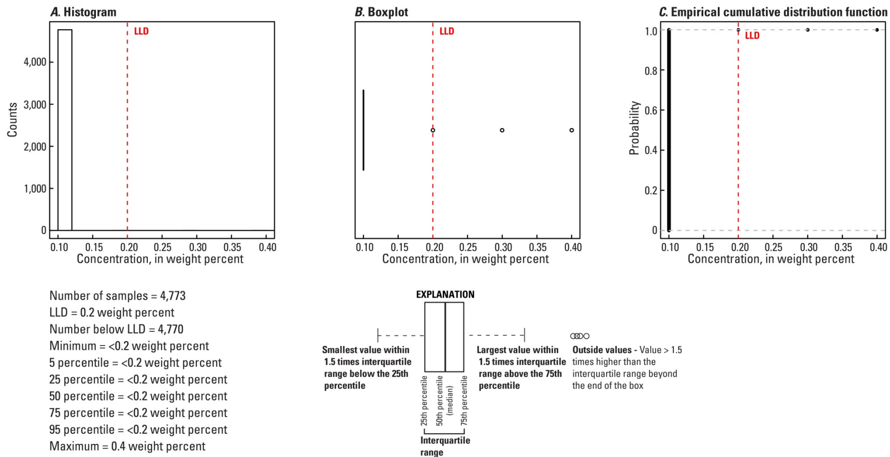
Figure 187. A, Histogram and summary statistics; B, Boxplot; C, Empirical cumulative distribution function; and D, Distribution of pyrite in the soil C horizon, conterminous United States (LLD, lower limit of determination; wt. %, weight percent).
