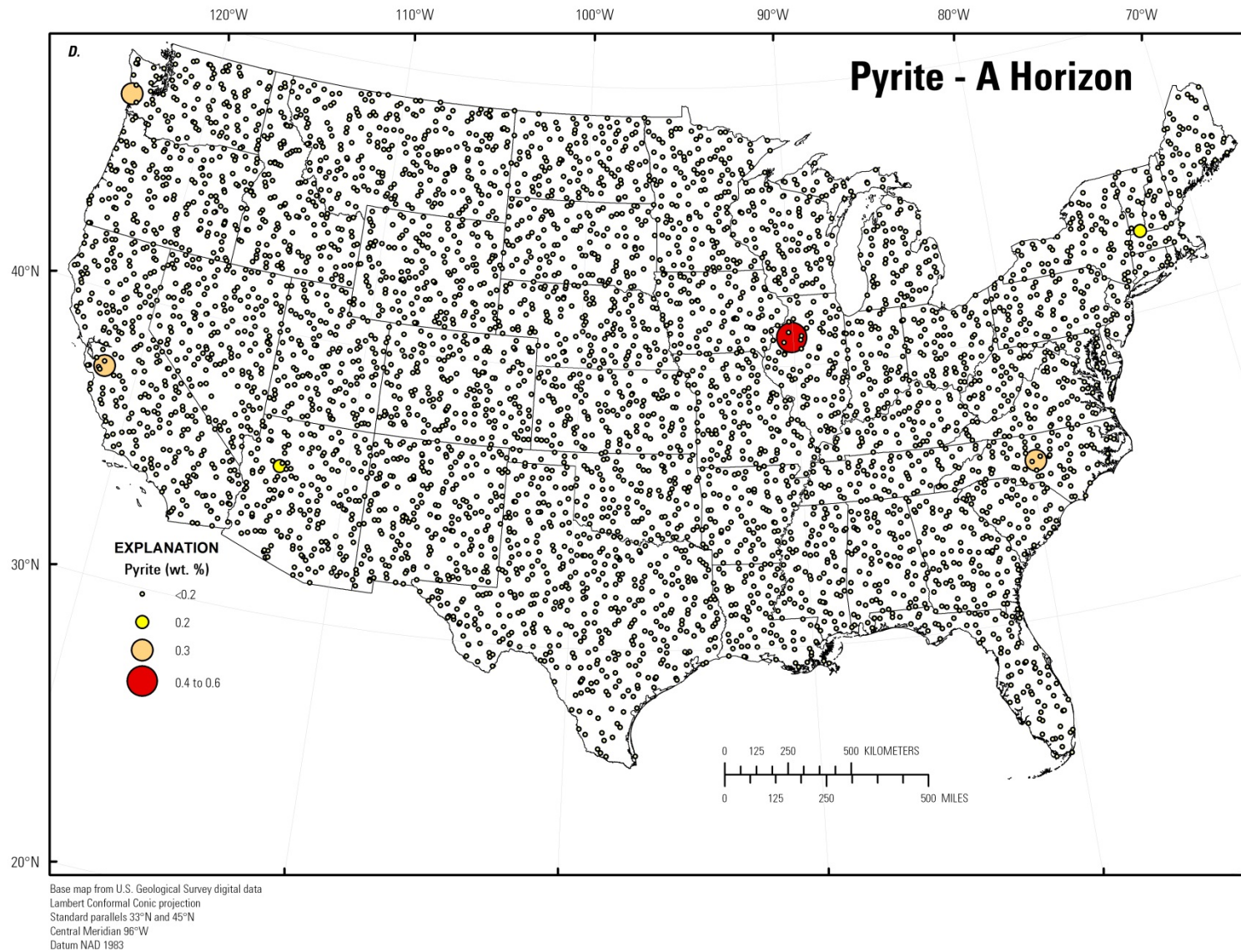
Figure 186. A, Histogram and summary statistics; B, Boxplot; C, Empirical cumulative distribution function; and D, Distribution of pyrite in the soil A horizon, conterminous United States (LLD, lower limit of determination; wt. %, weight percent).—Continued
