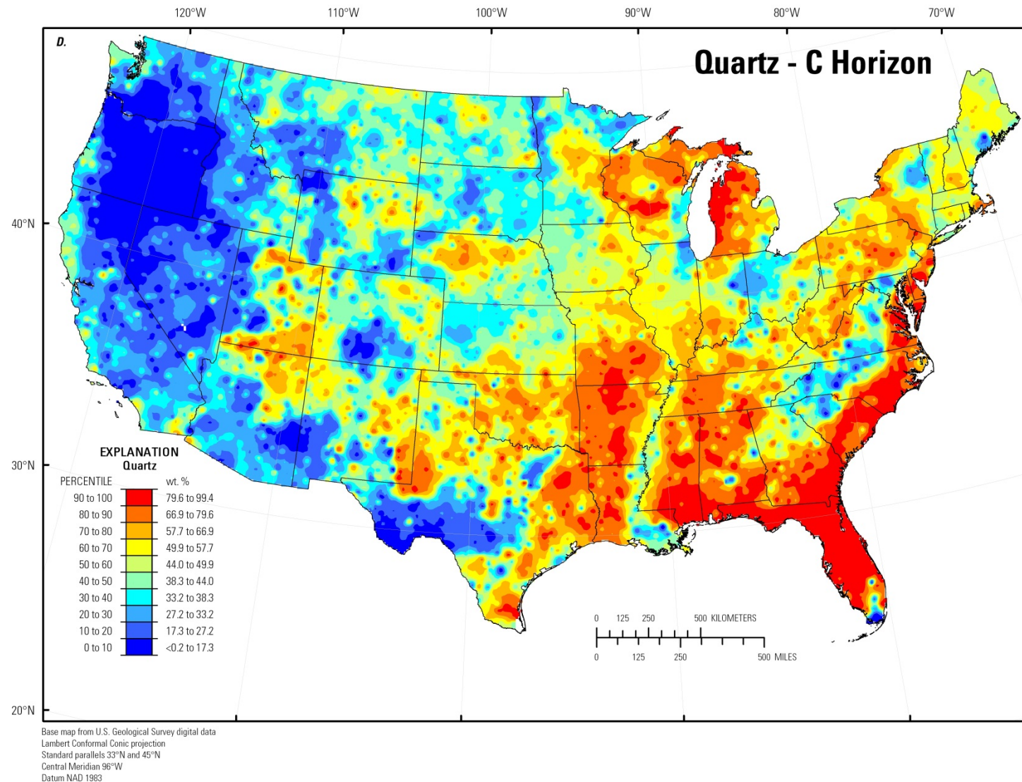
Figure 141. A, Histogram and summary statistics; B, Boxplot; C, Empirical cumulative distribution function; and D, Distribution of quartz in the soil C horizon, conterminous United States (LLD, lower limit of determination; wt. %, weight percent).—Continued
