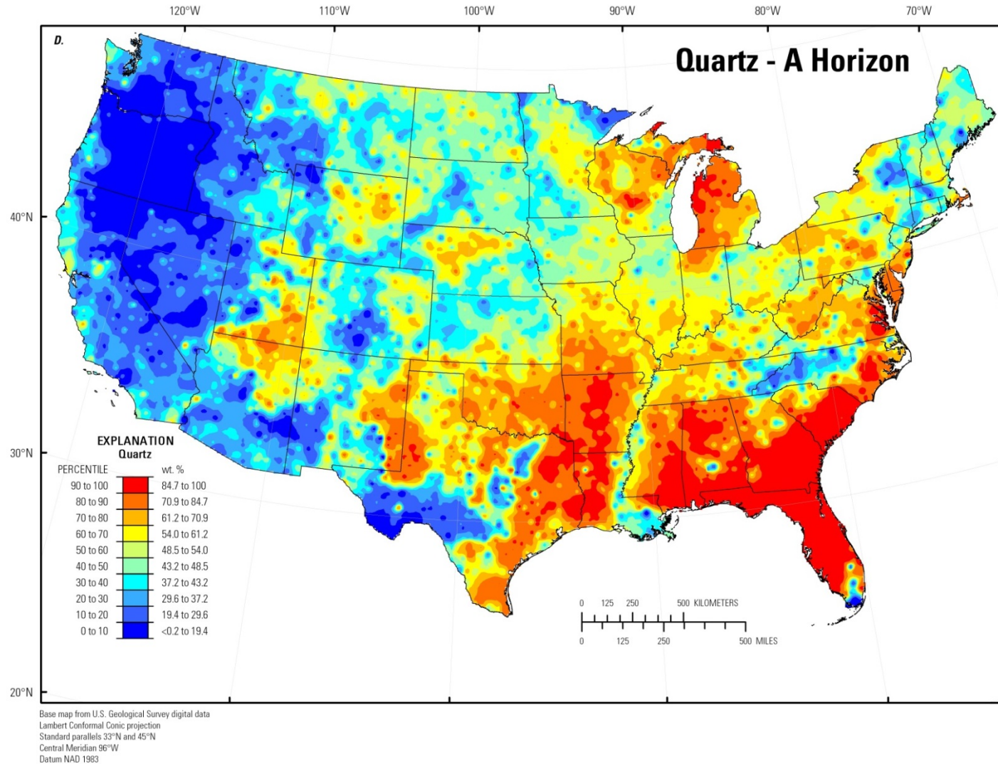
Figure 140. A, Histogram and summary statistics; B, Boxplot; C, Empirical cumulative distribution function; and D, Distribution of quartz in the soil A horizon, conterminous United States (LLD, lower limit of determination; wt. %, weight percent).—Continued
