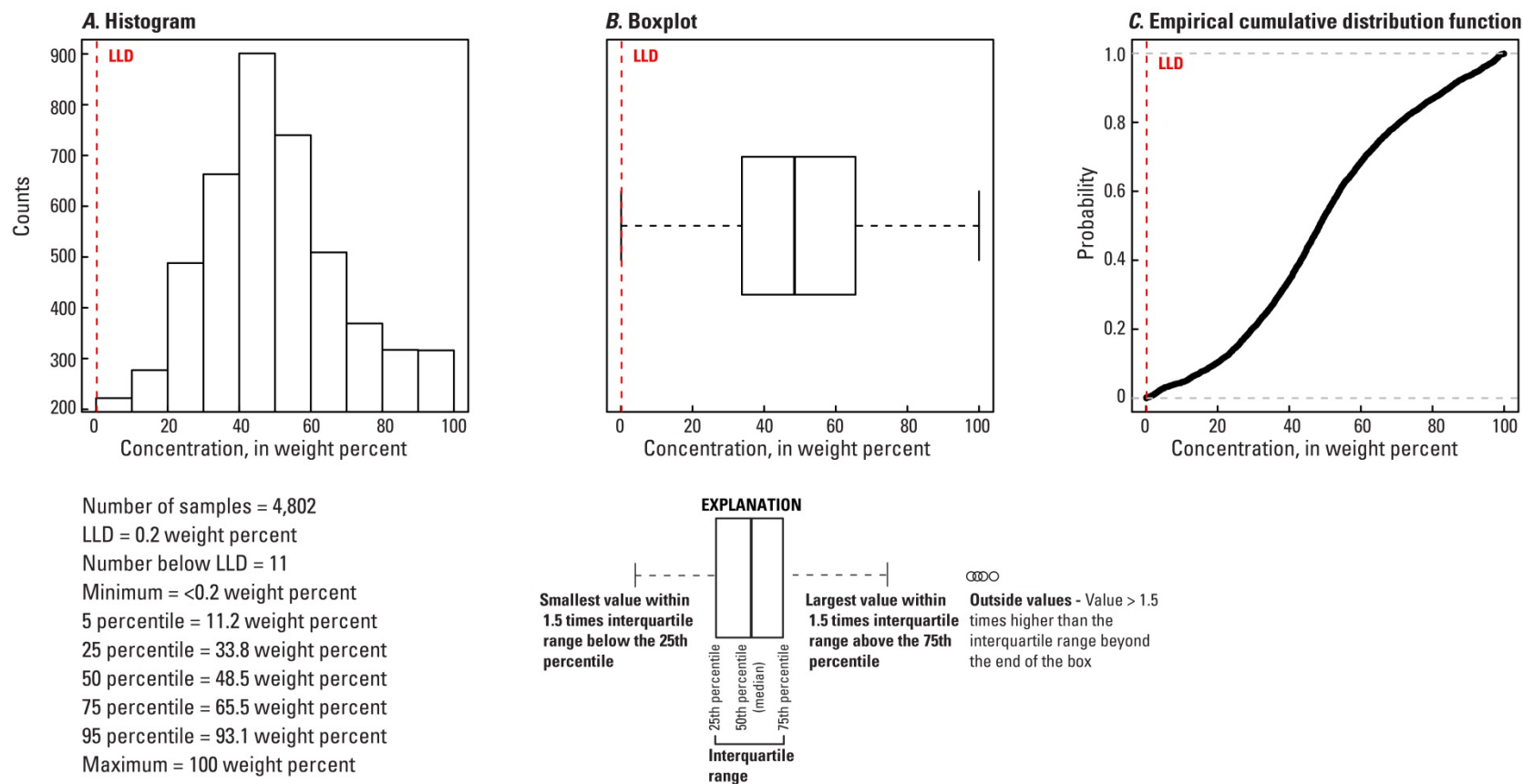
Figure 140. A, Histogram and summary statistics; B, Boxplot; C, Empirical cumulative distribution function; and D, Distribution of quartz in the soil A horizon, conterminous United States (LLD, lower limit of determination; wt. %, weight percent).
