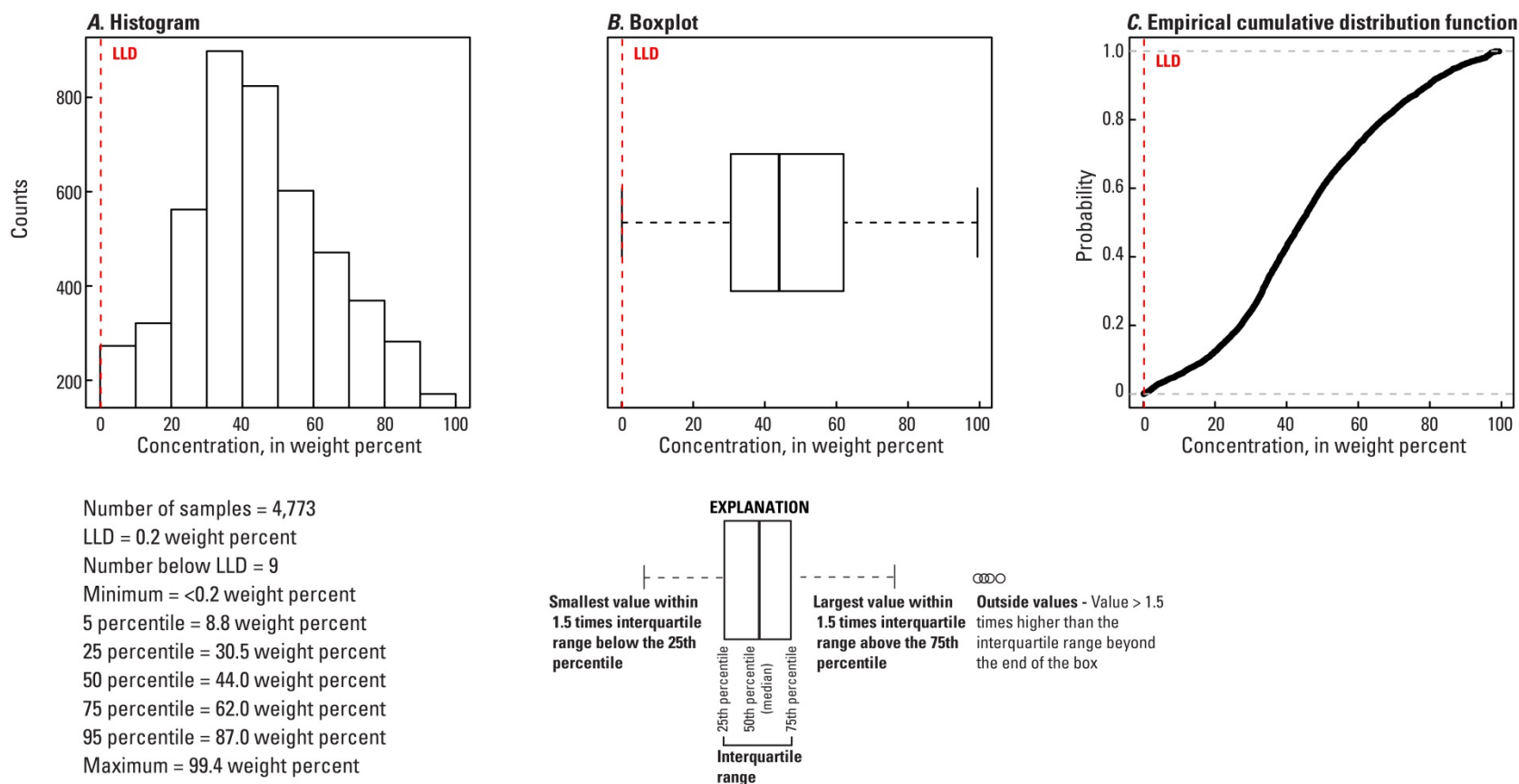
Figure 141. A, Histogram and summary statistics; B, Boxplot; C, Empirical cumulative distribution function; and D, Distribution of quartz in the soil C horizon, conterminous United States (LLD, lower limit of determination; wt. %, weight percent).
