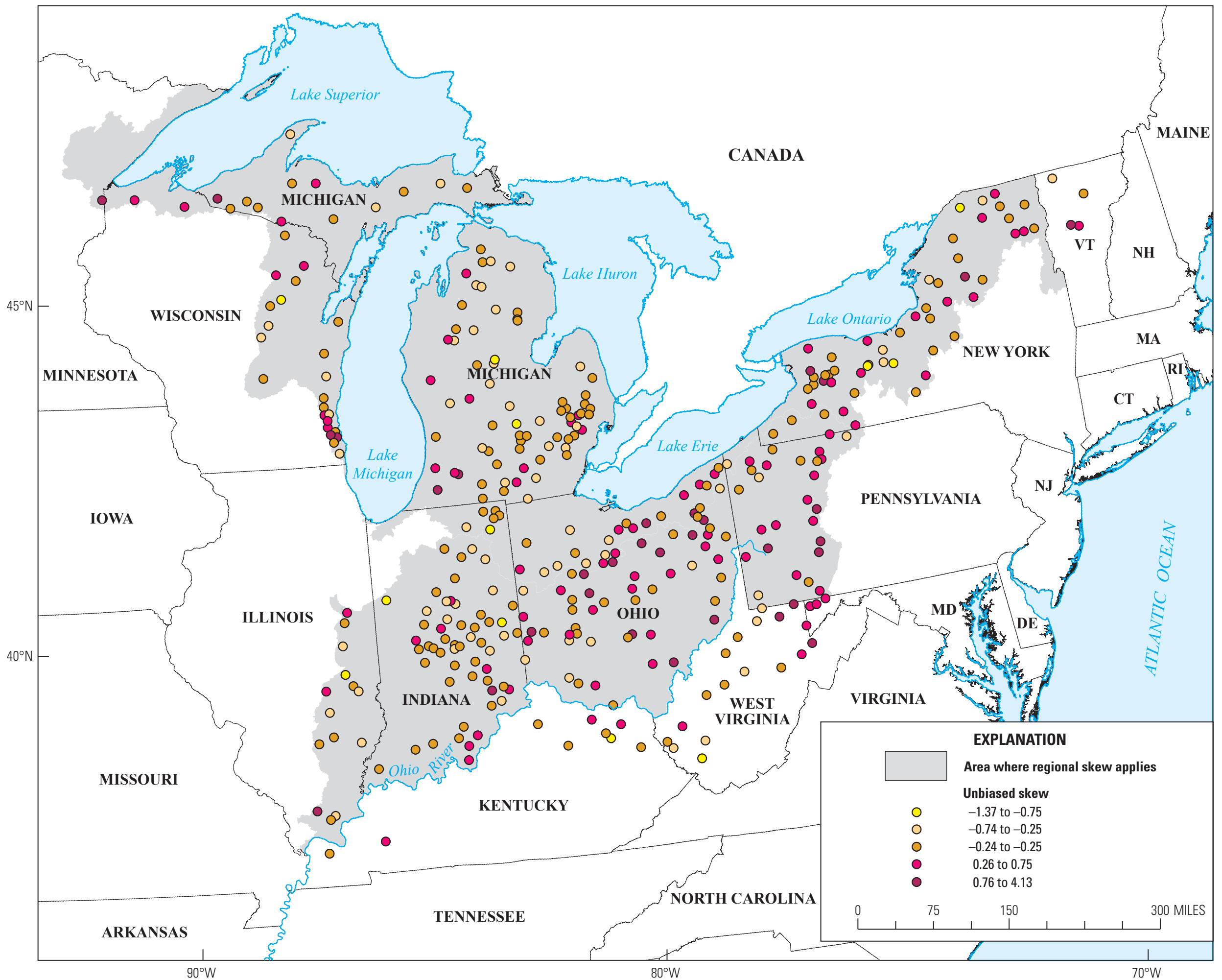
Figure 3. Map showing unbiased station skew of streamgages in the Great Lakes and Ohio River Basins used in the regional skew analysis.
