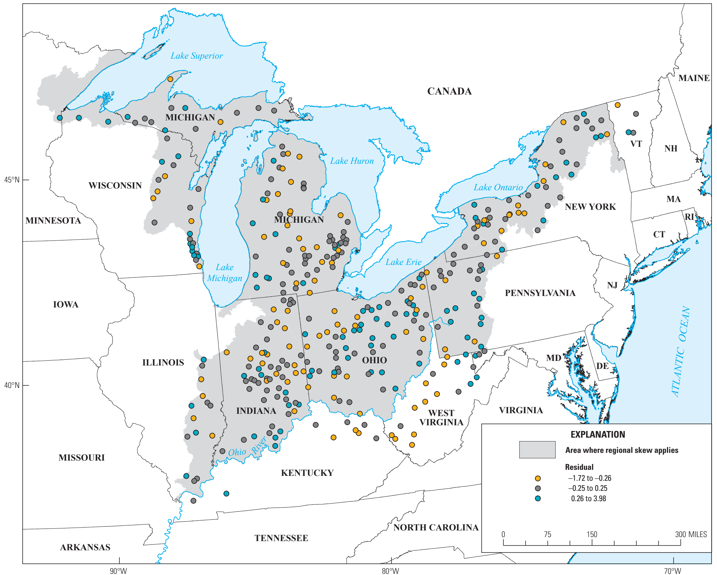
Figure 5. Map showing residuals from constant model of skew for 368 streamgages in the Great Lakes and Ohio River Basins used in the regional skew analysis.
