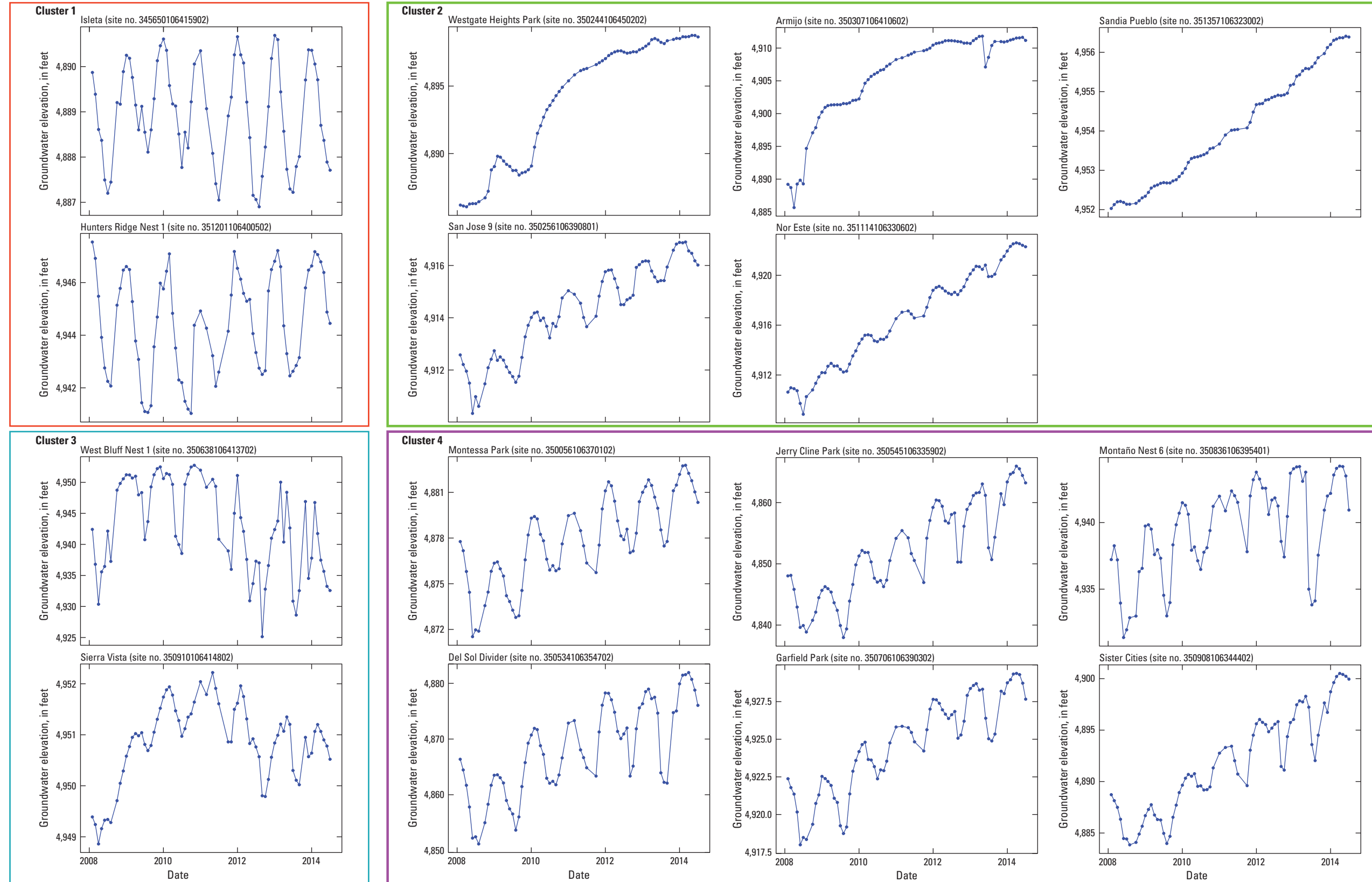
Figure 23. Clustered monthly median hydrographs plotted using A, the same fixed y-axis range and B, an independent y-axis range for all plots.
