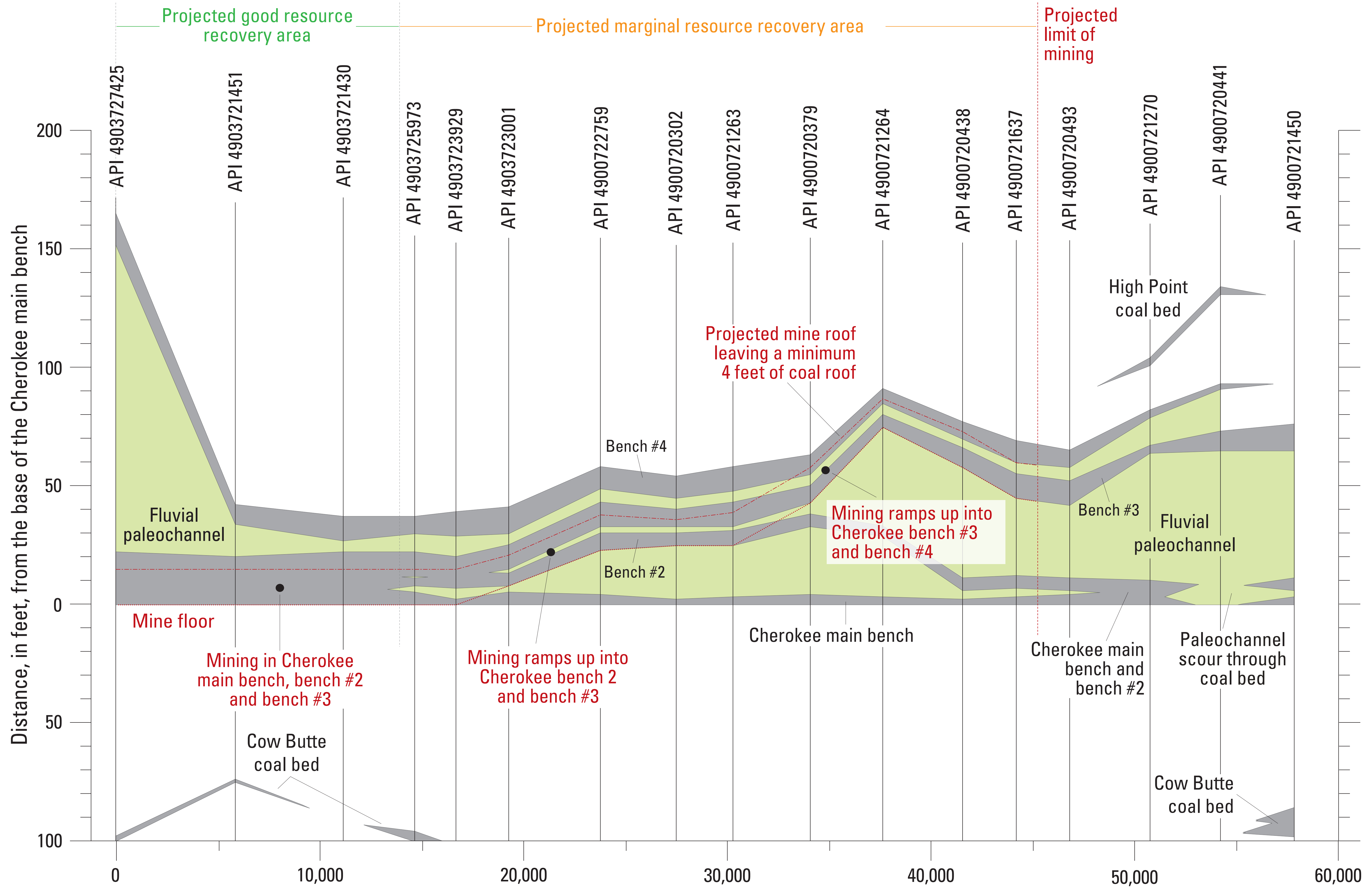
Distance, in feet VERTICAL SCALE GREATLY EXAGGERATED DATUM IS NAVD 88
