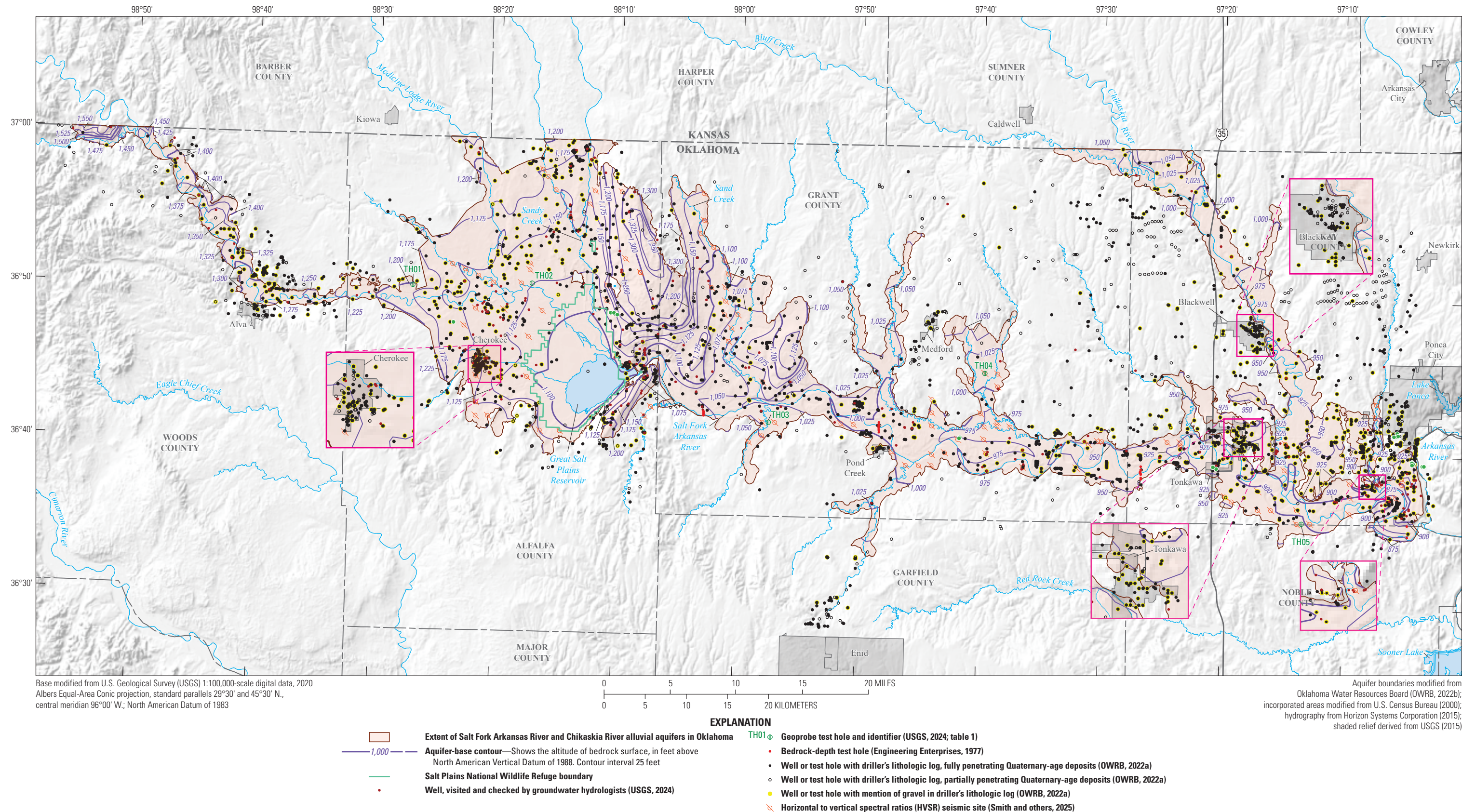
Figure 14. Altitude of the base of the Salt Fork Arkansas River and Chikaskia River alluvial aquifers, northern Oklahoma, decreasing in altitude from west to east.
