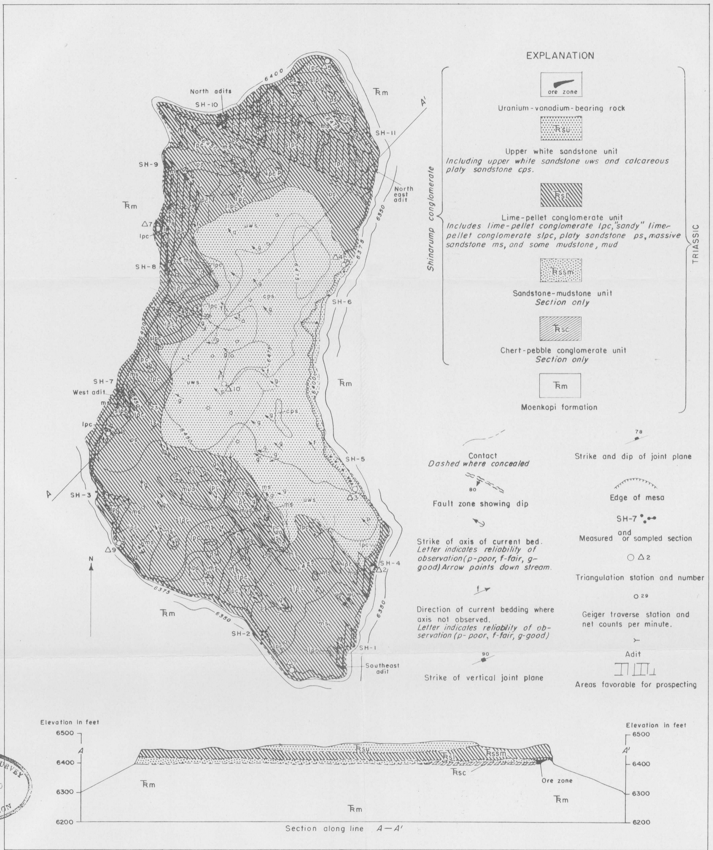
FIGURE 3.- GEOLOGIC SECTION AND MAP OF THE SURFACE OF SHINARUMP MESA, EMERY COUNTY, UTAH
