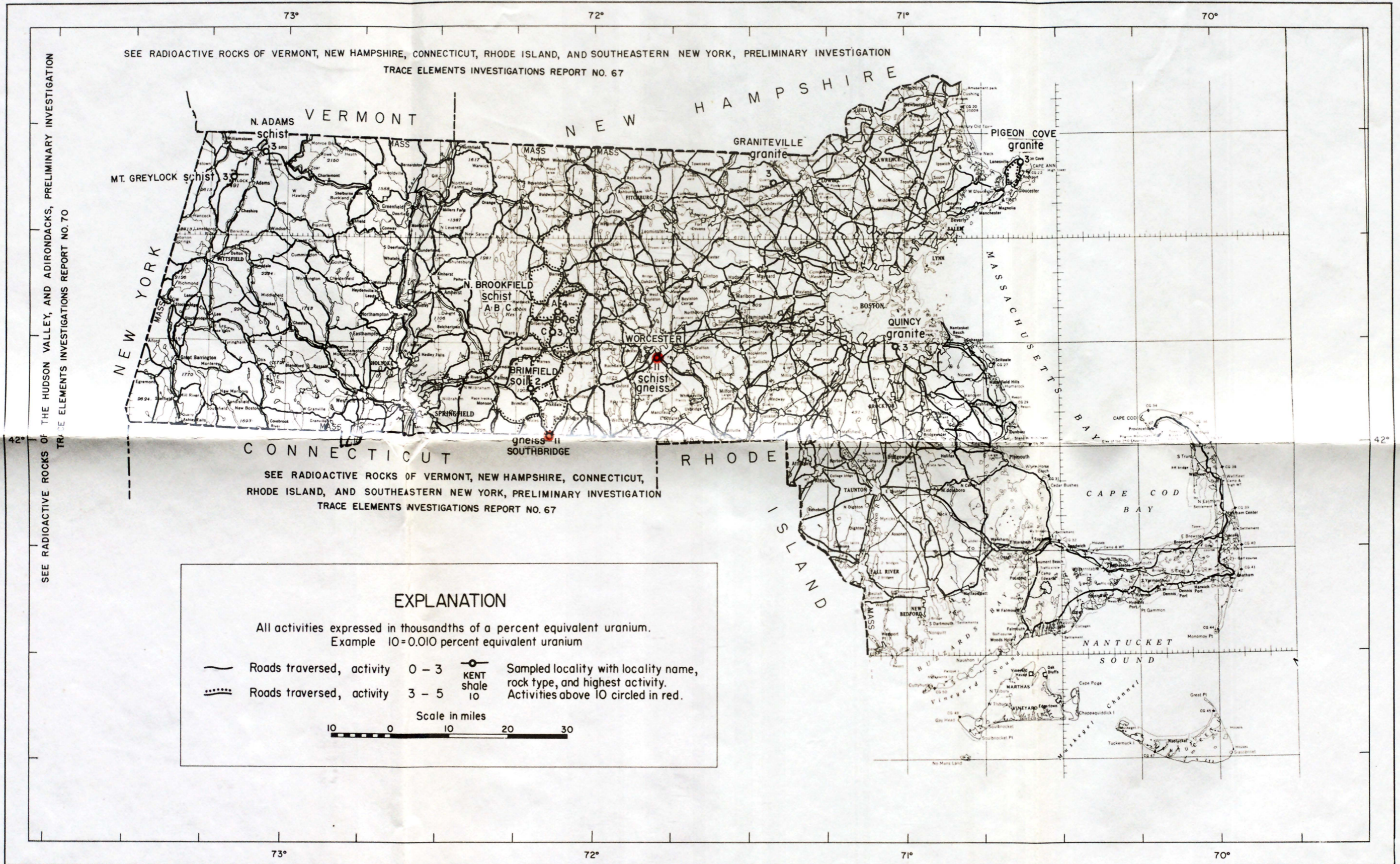
FIGURE 1. RADIOACTIVE ROCKS OF MASSACHUSETTS
