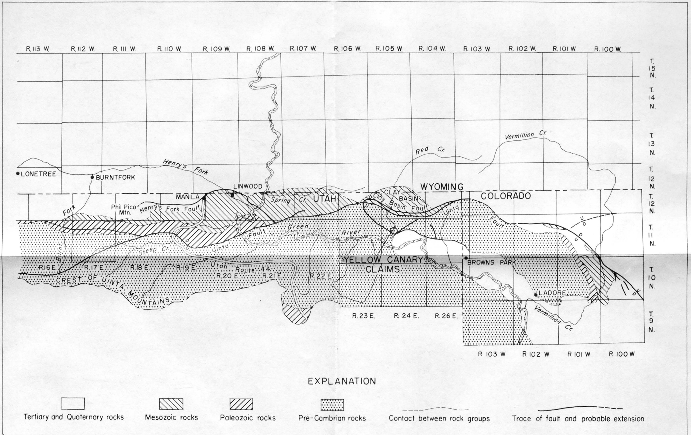
FIGURE 2.— GEOLOGIC MAP, NORTH FLANK UINTA MOUNTAINS, COLORADO, UTAH, AND WYOMING
