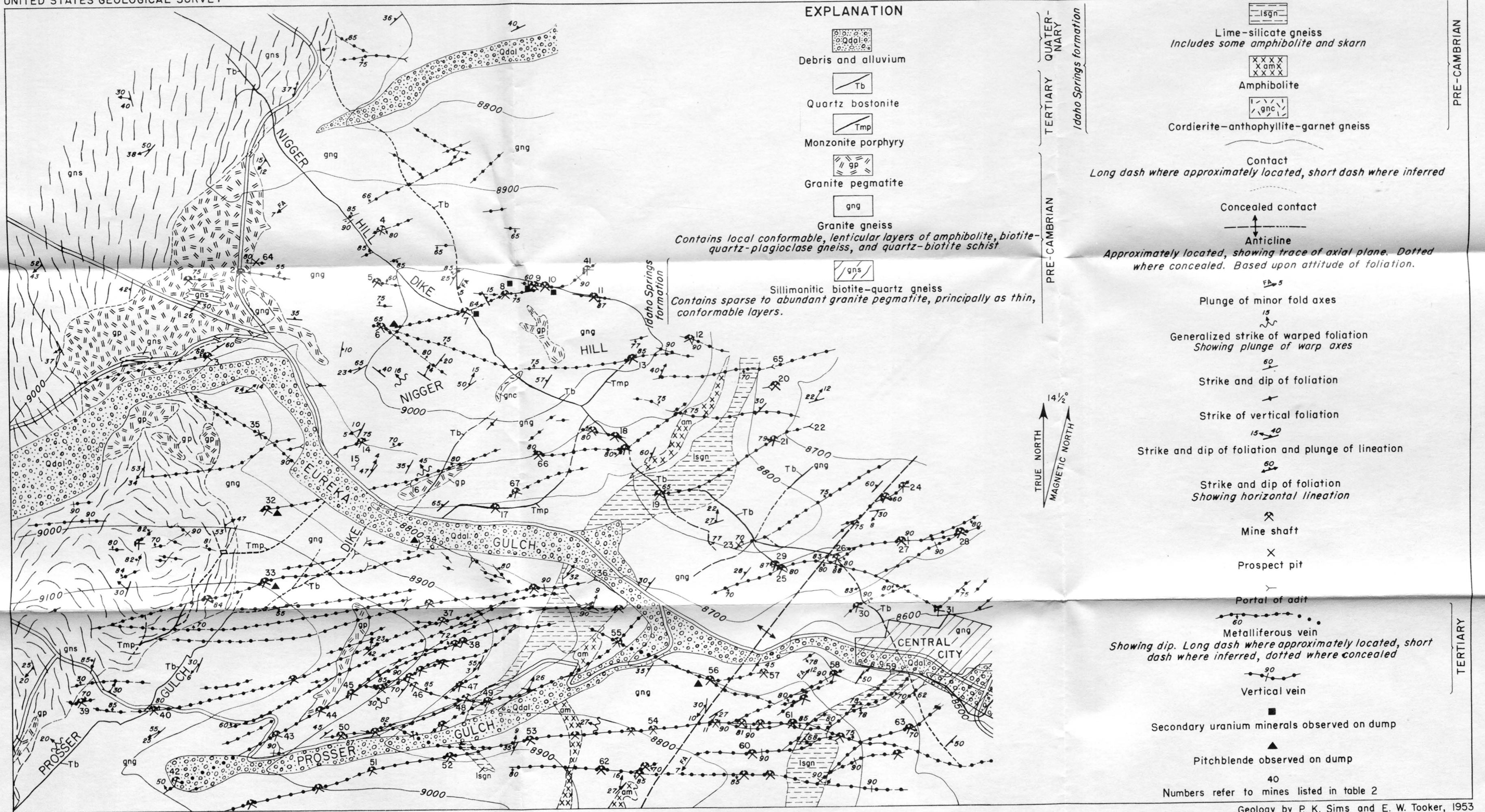
FIGURE 2.-GEOLOGIC MAP OF EUREKA GULCH AREA, CENTRAL CITY DISTRICT, GILPIN COUNTY, COLORADO
