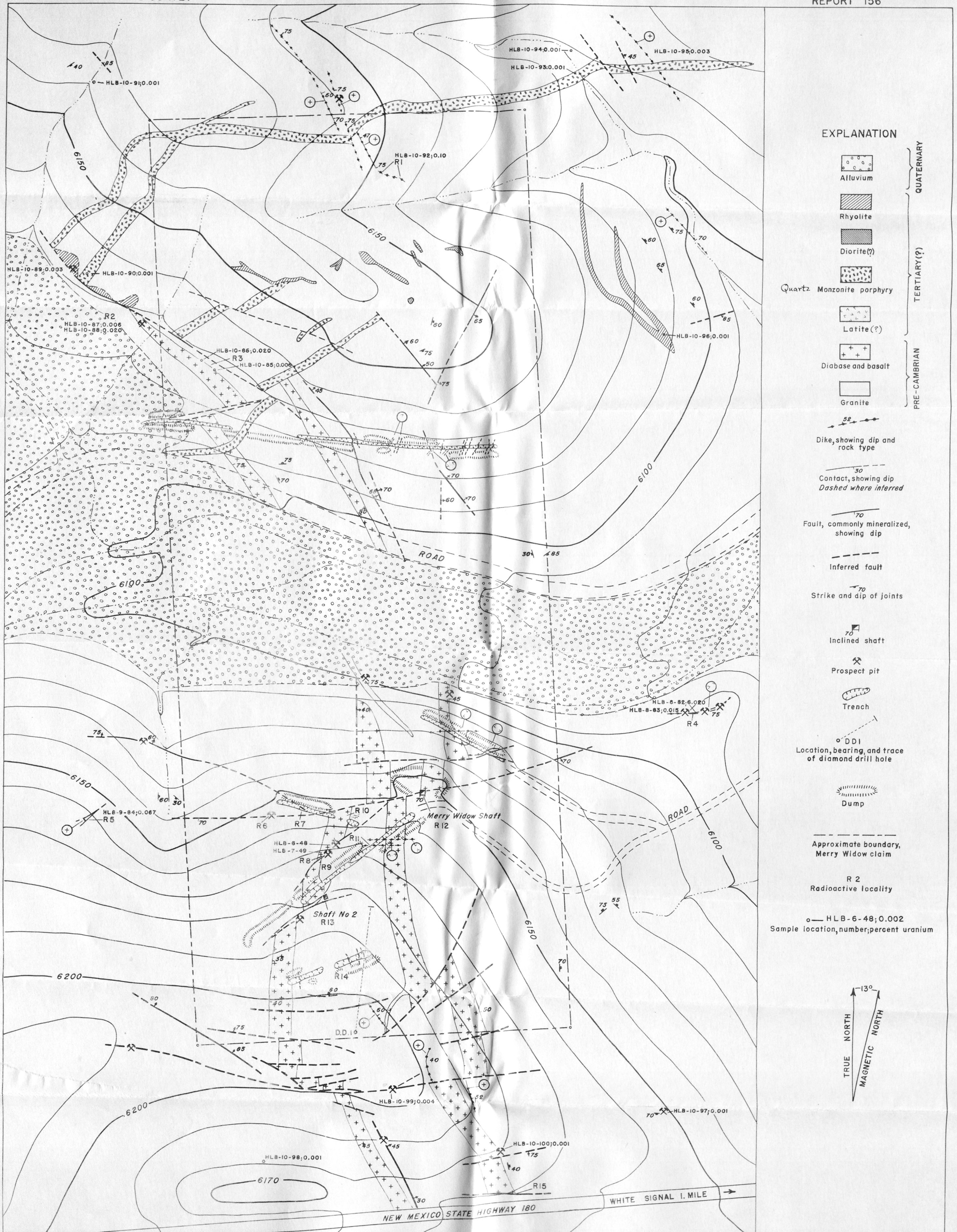
FIGURE 2.—GEOLOGIC MAP, MERRY WIDOW CLAIM, WHITE SIGNAL DISTRICT, GRANT COUNTY, NEW MEXICO.
