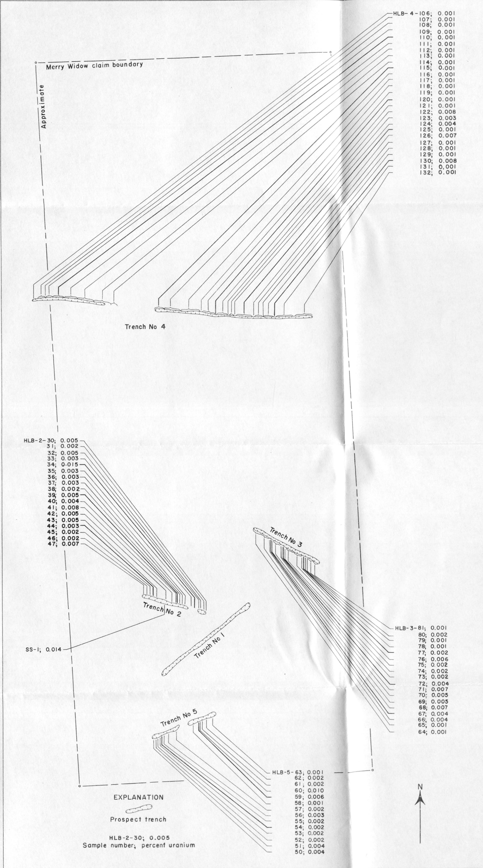
FIGURE 3—ASSAY PLAN, TRENCHES NOS. 2, 3, 4, AND 5, MERRY WIDOW CLAIM, WHITE SIGNAL DISTRICT, GRANT COUNTY, NEW MEXICO
