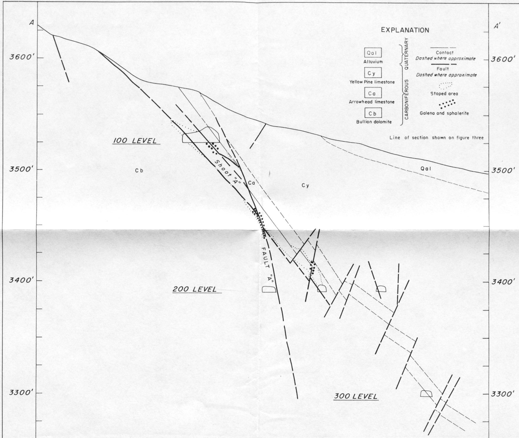
FIGURE 4.-GEOLOGIC SECTION, GREEN MONSTER MINE, CLARK COUNTY, NEVADA.
