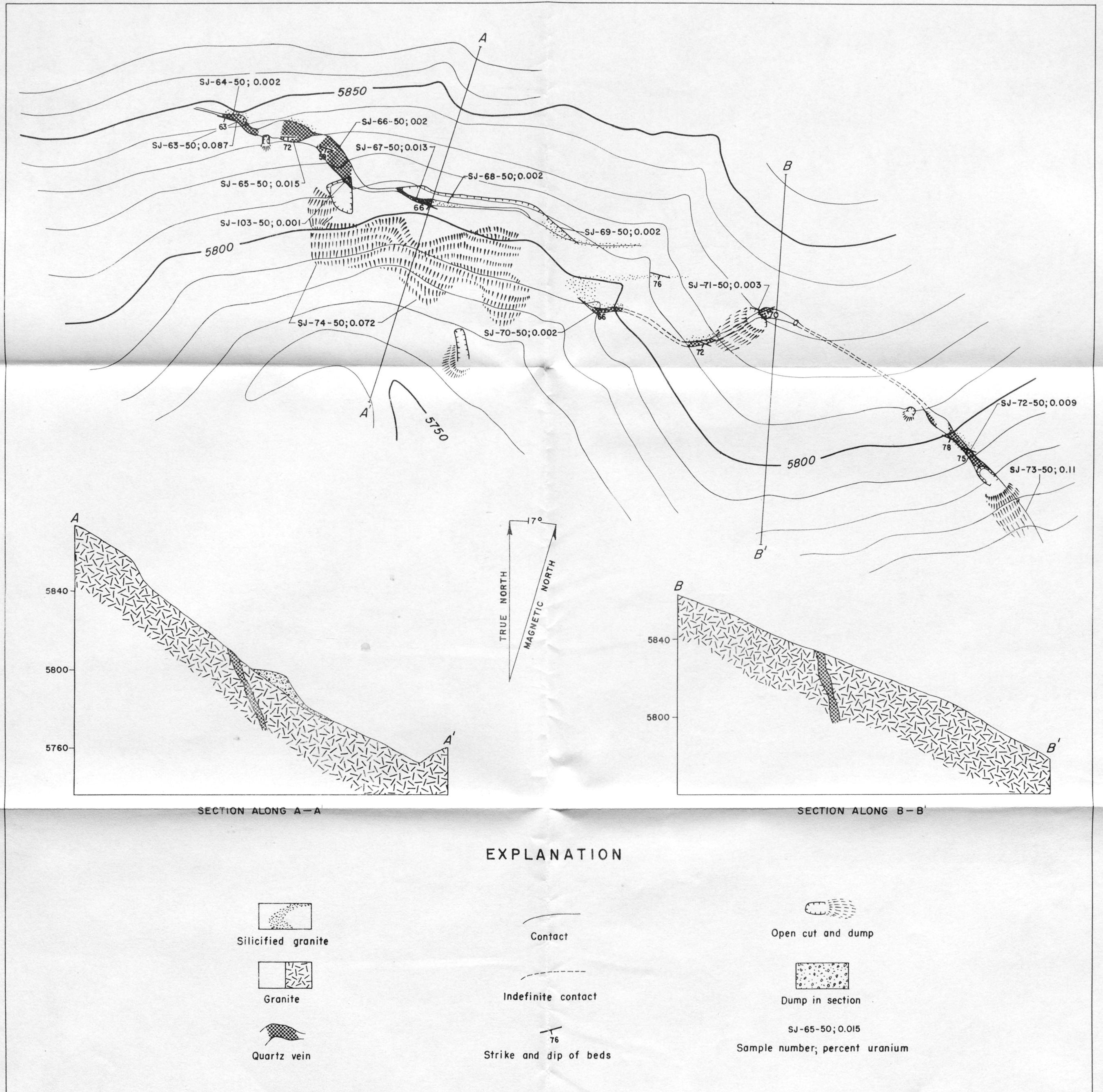
FIGURE 5. - GEOLOGIC MAP AND SECTIONS OF THE WEST WILLYS CLAIM, LYON COUNTY, NEVADA
