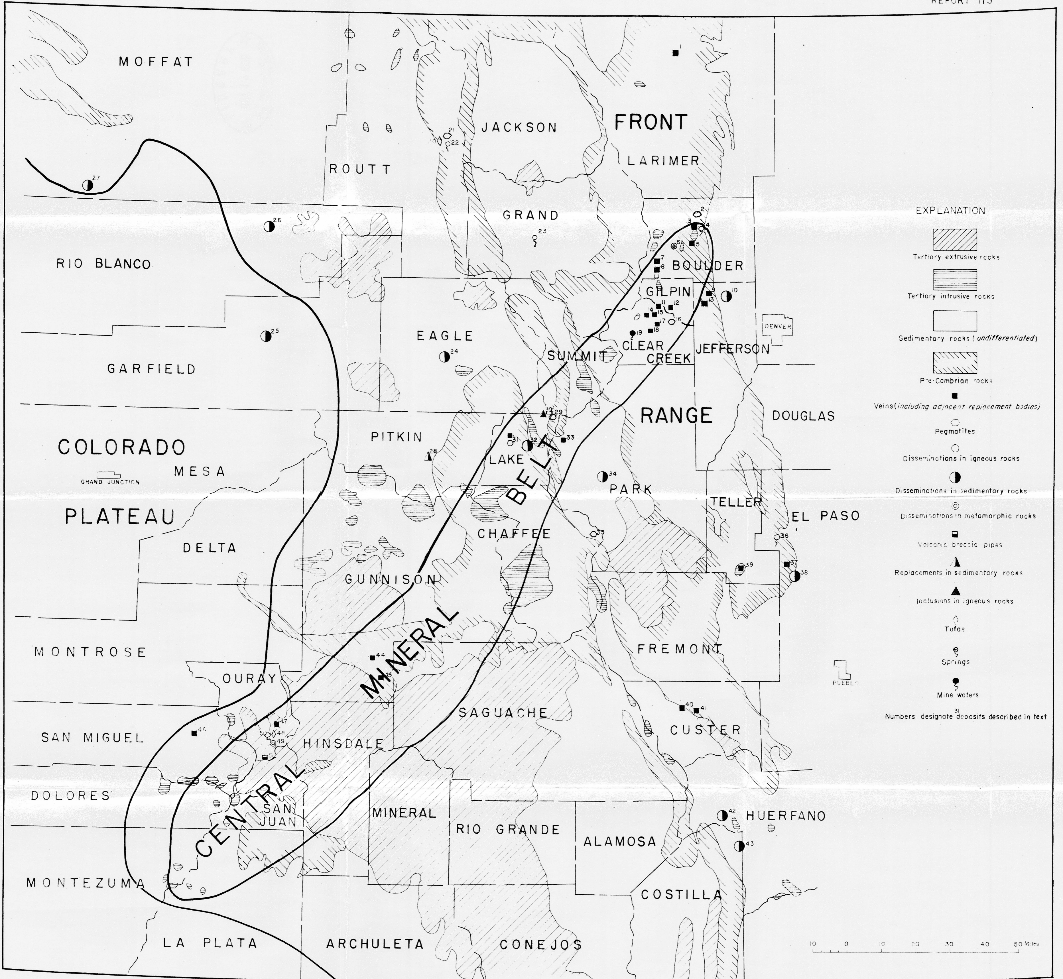
FIG. 1—INDEX MAP SHOWING DISTRIBUTION OF URANIUM DEPOSITS IN COLORADO, GENERALLY EXCLUSIVE OF THE COLORADO PLATEAU.
