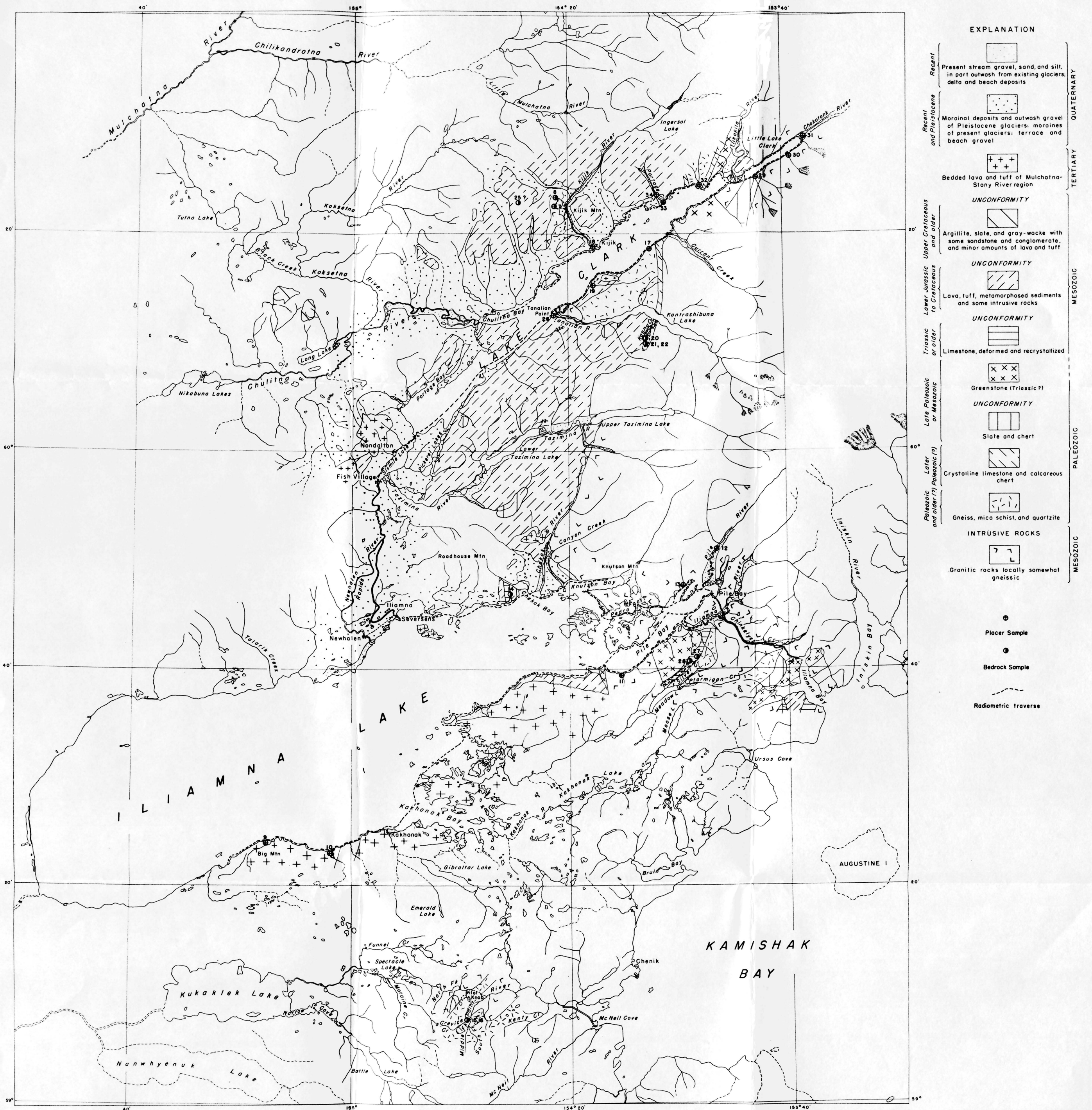
GEOLOGIC MAP OF THE ILIAMNA LAKE - LAKE CLARK REGION SHOWING SAMPLE LOCALITIES AND RADIOMETRIC TRAVERSES
