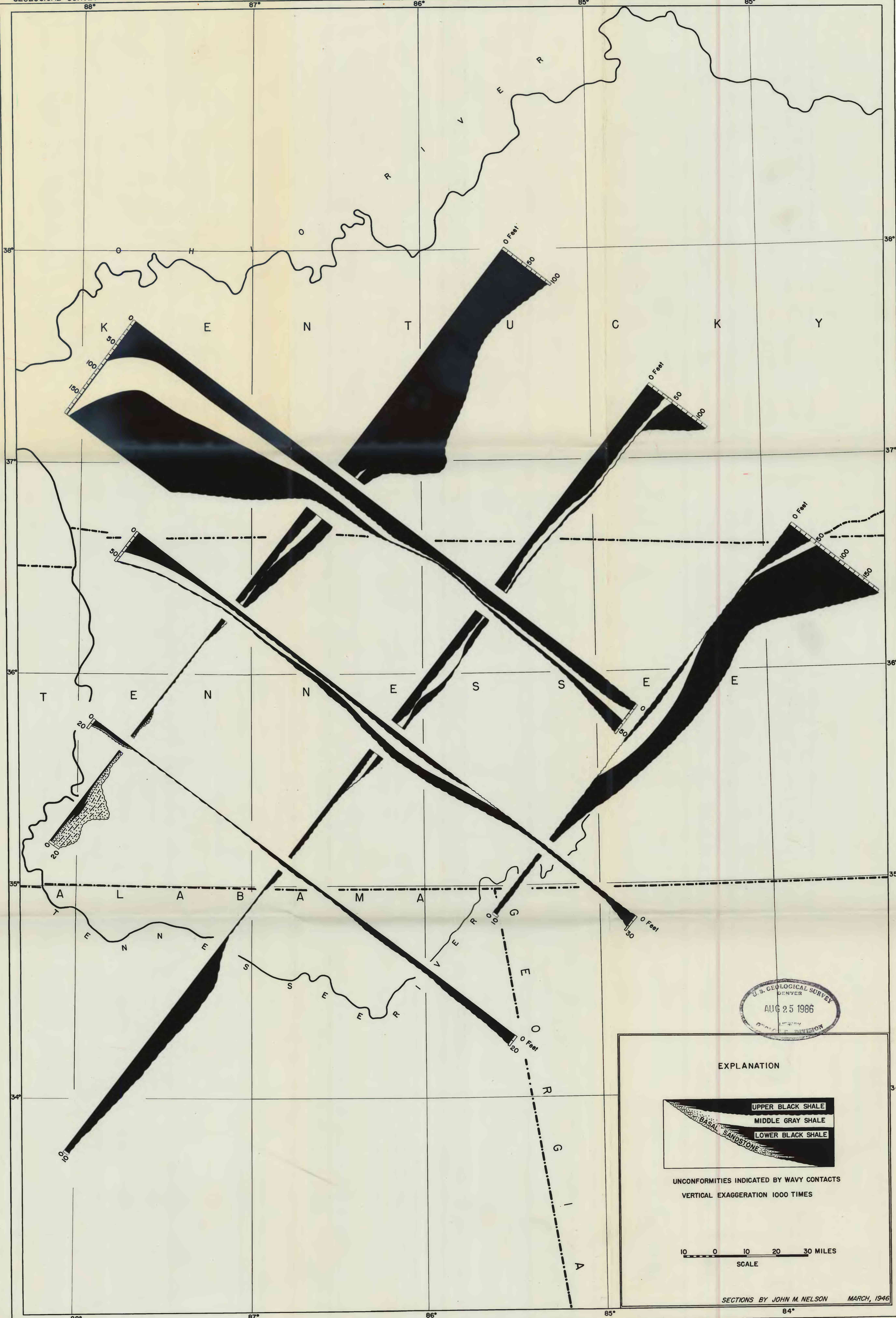
FIG. 3 STRATIGRAPHY OF THE CHATTANOOGA SHALE
