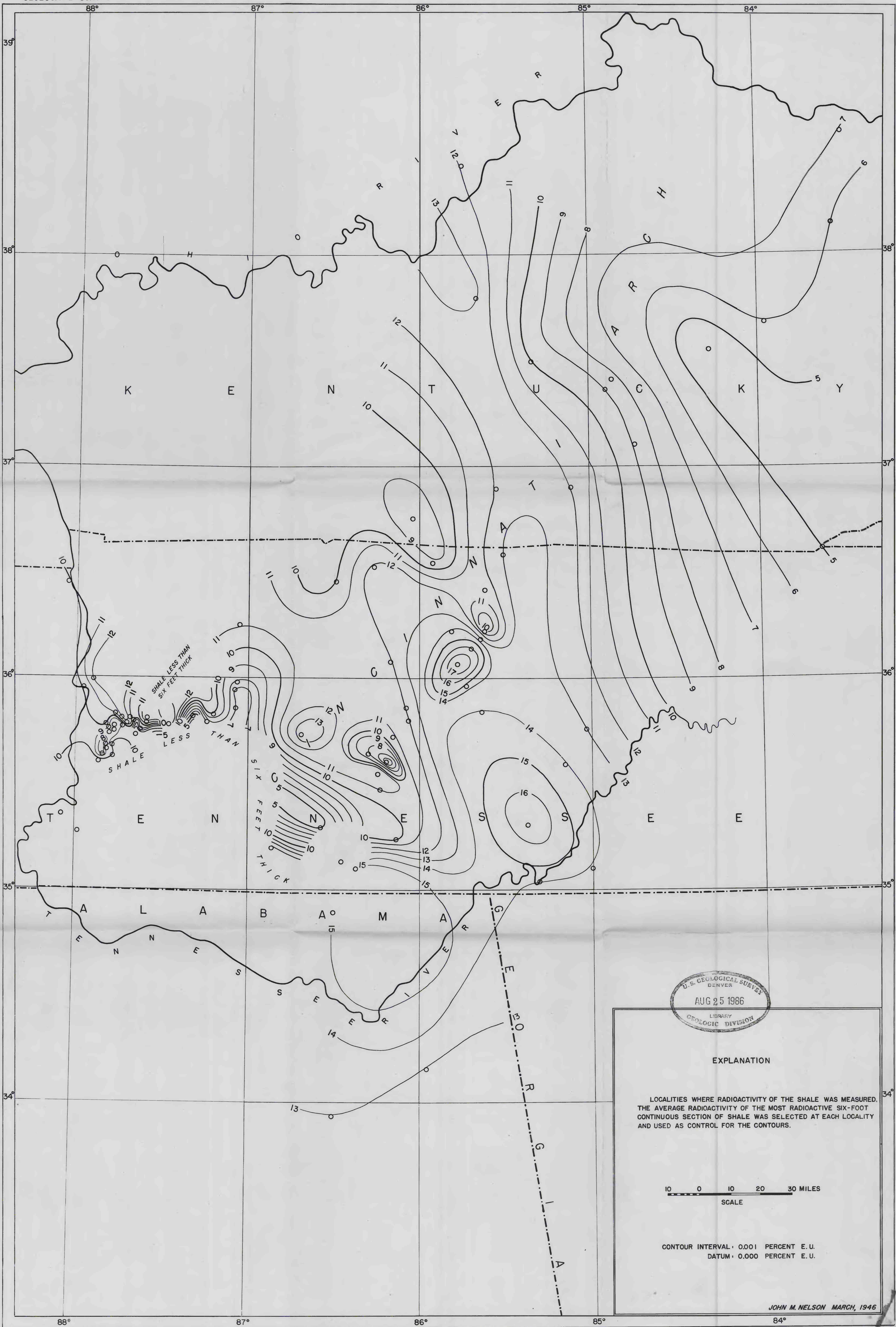
FIG. 7 ISORADIOACTIVITY MAP OF THE CHATTANOOGA SHALE
