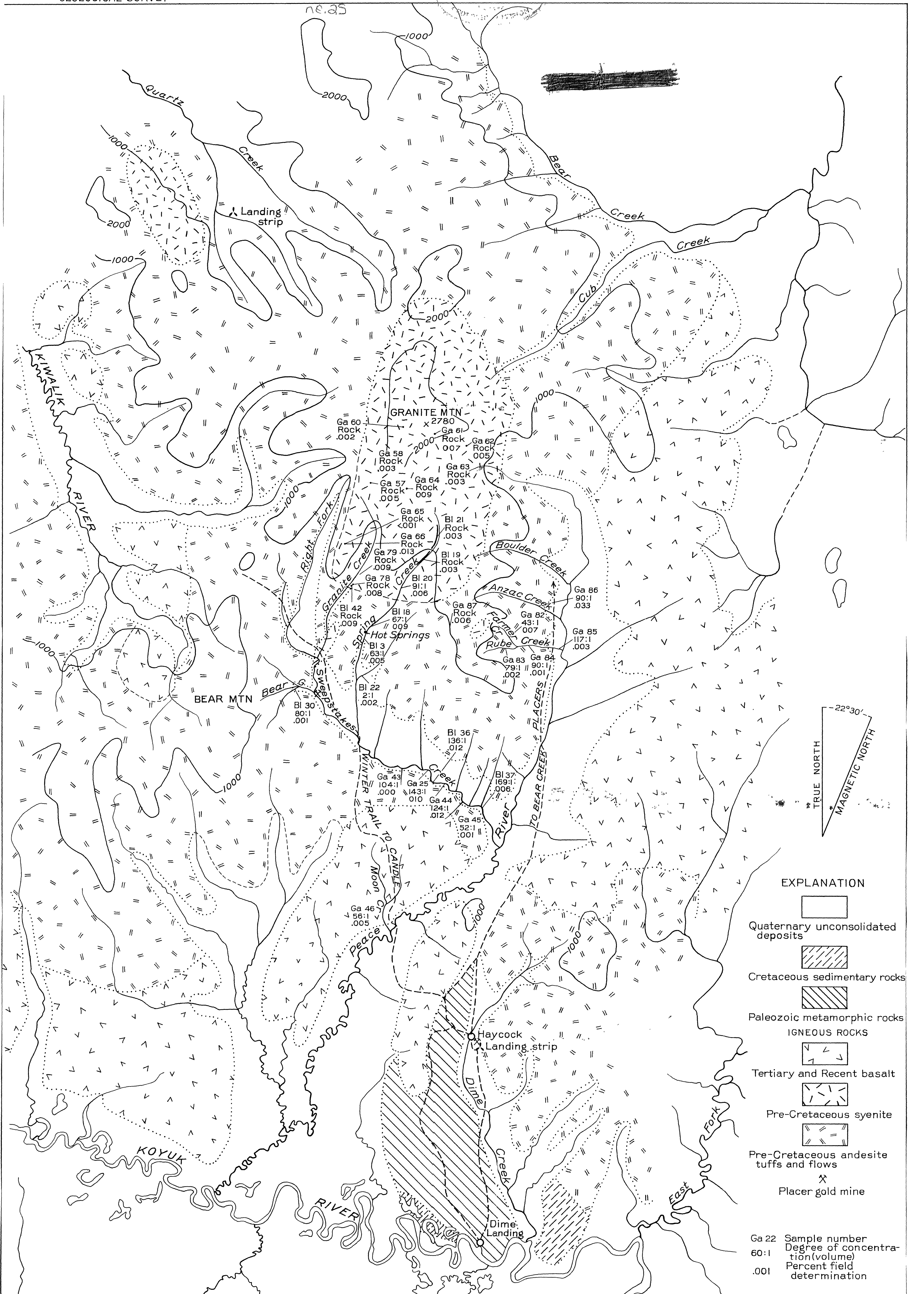
FIGURE 2 GEOLOGIC SKETCH MAP OF SWEEPSTAKES CREEK AND VICINITY, KOYUK DISTRICT, SEWARD PENINSULA, ALASKA
