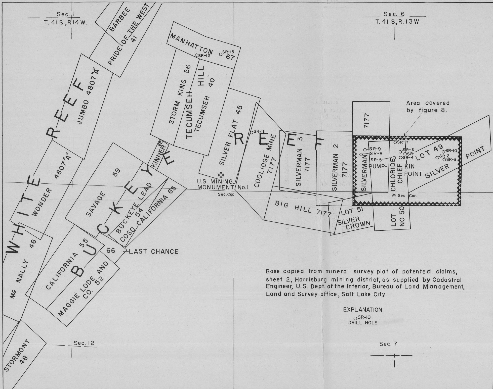
FIGURE 2.-MINERAL SURVEY PLAT SHOWING LOCATIONS OF DRILL HOLES, SILVER REEF DISTRICT, WASHINGTON COUNTY, UTAH.
