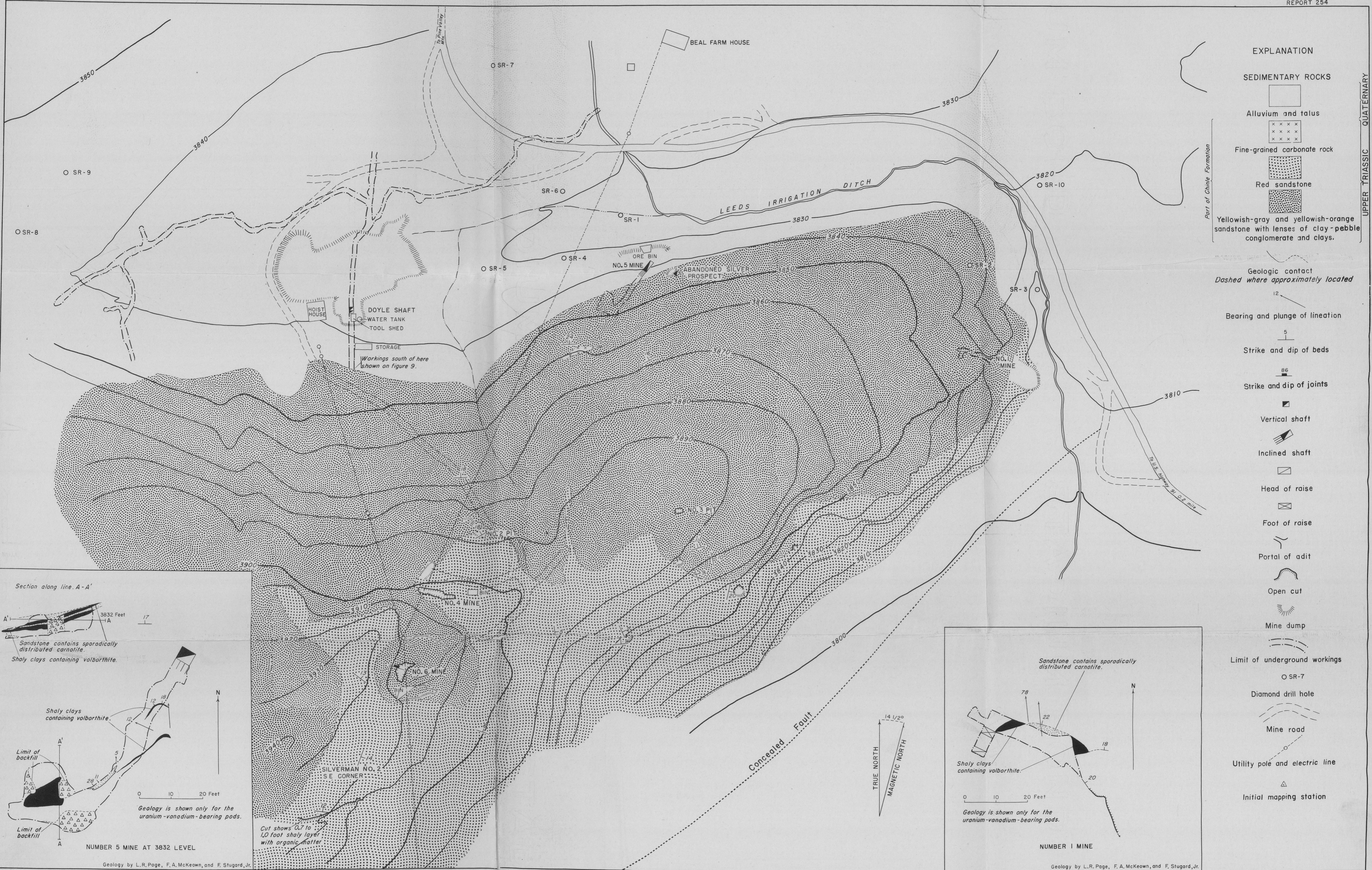
FIGURE 8.- GEOLOGY OF PUMPKIN POINT AREA, SILVER REEF DISTRICT, WASHINGTON COUNTY, UTAH.
