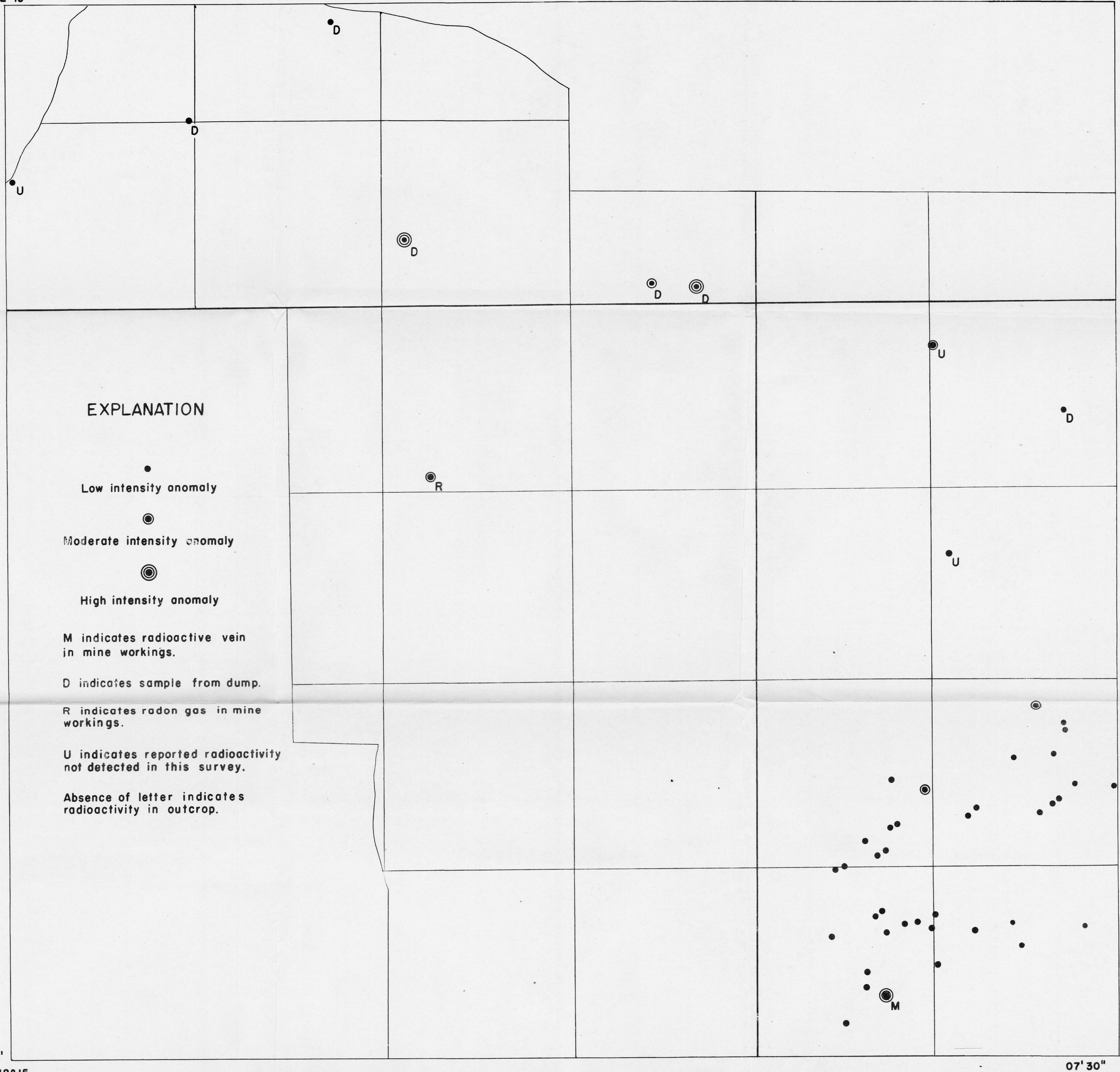
FIGURE 3 OVERLAY, SHOWING RADIOACTIVITY ANOMALIES, TO ACCOMPANY THE GEOLOGIC MAP OF THE COMET AREA, JEFFERSON CITY QUADRANGLE JEFFERSON COUNTY, MONTANA
