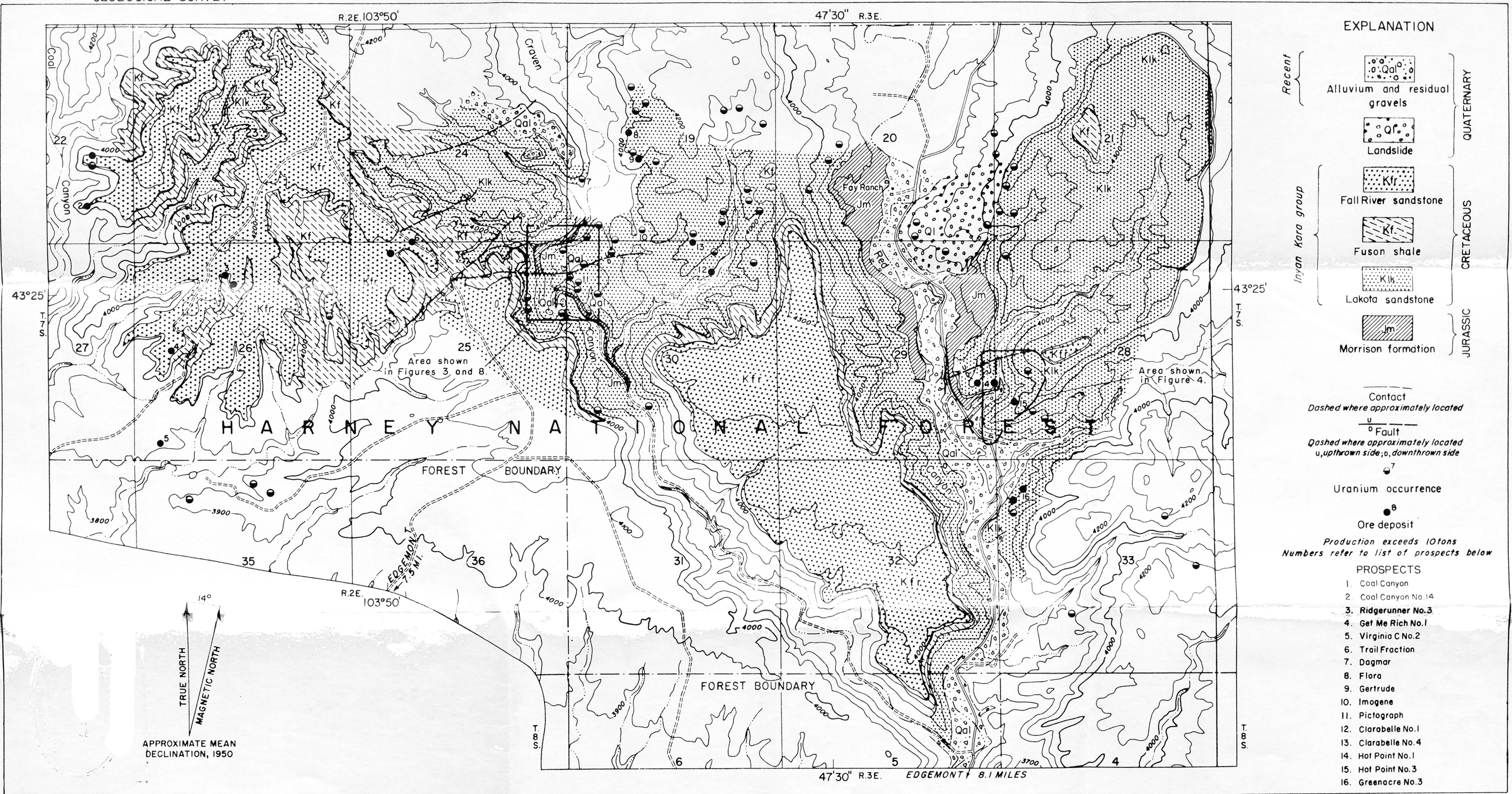
FIGURE 5—GEOLOGIC MAP, CRAVEN AND RED CANYON AREAS, FALL RIVER COUNTY, SOUTH DAKOTA
