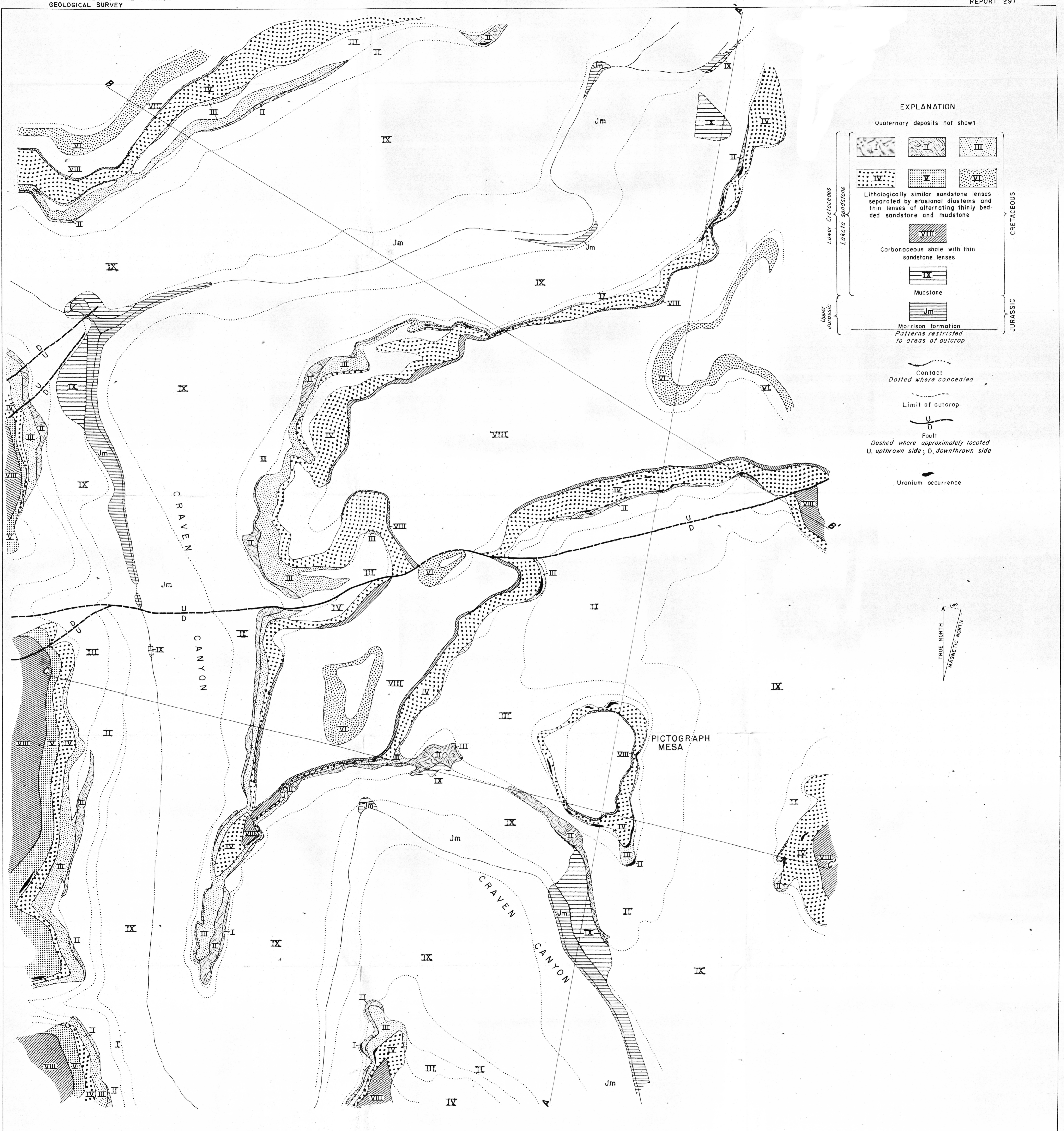
FIGURE 10.—OUTCROP MAP OF PART OF CRAVEN CANYON, FALL RIVER COUNTY, SOUTH DAKOTA, SHOWING LENSES IN THE LAKOTA SANDSTONE
