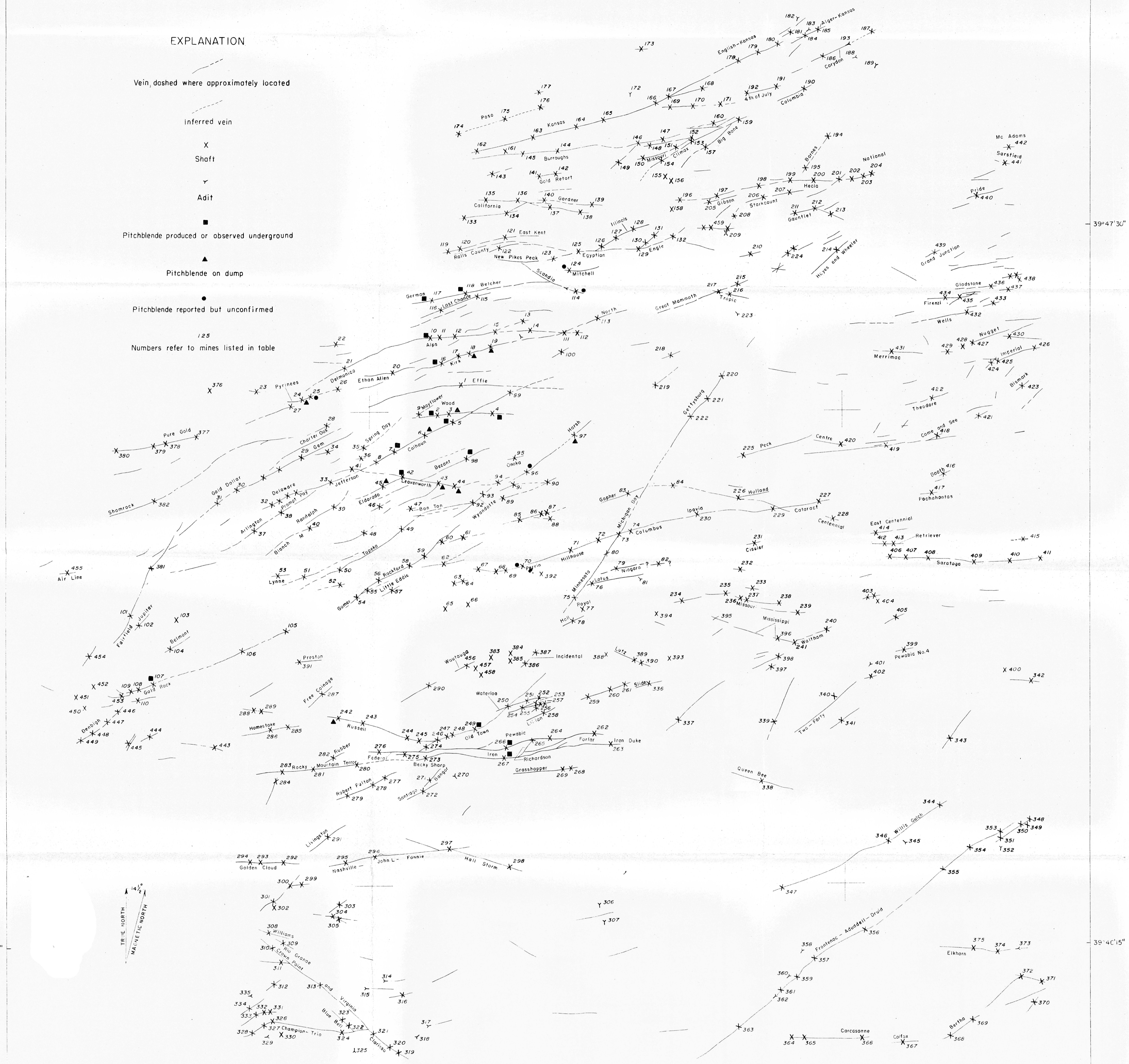
FIGURE 3.-PRELIMINARY MAP OF PART OF THE CENTRAL CITY DISTRICT, COLORADO, SHOWING VEINS AND PRINCIPAL MINES
