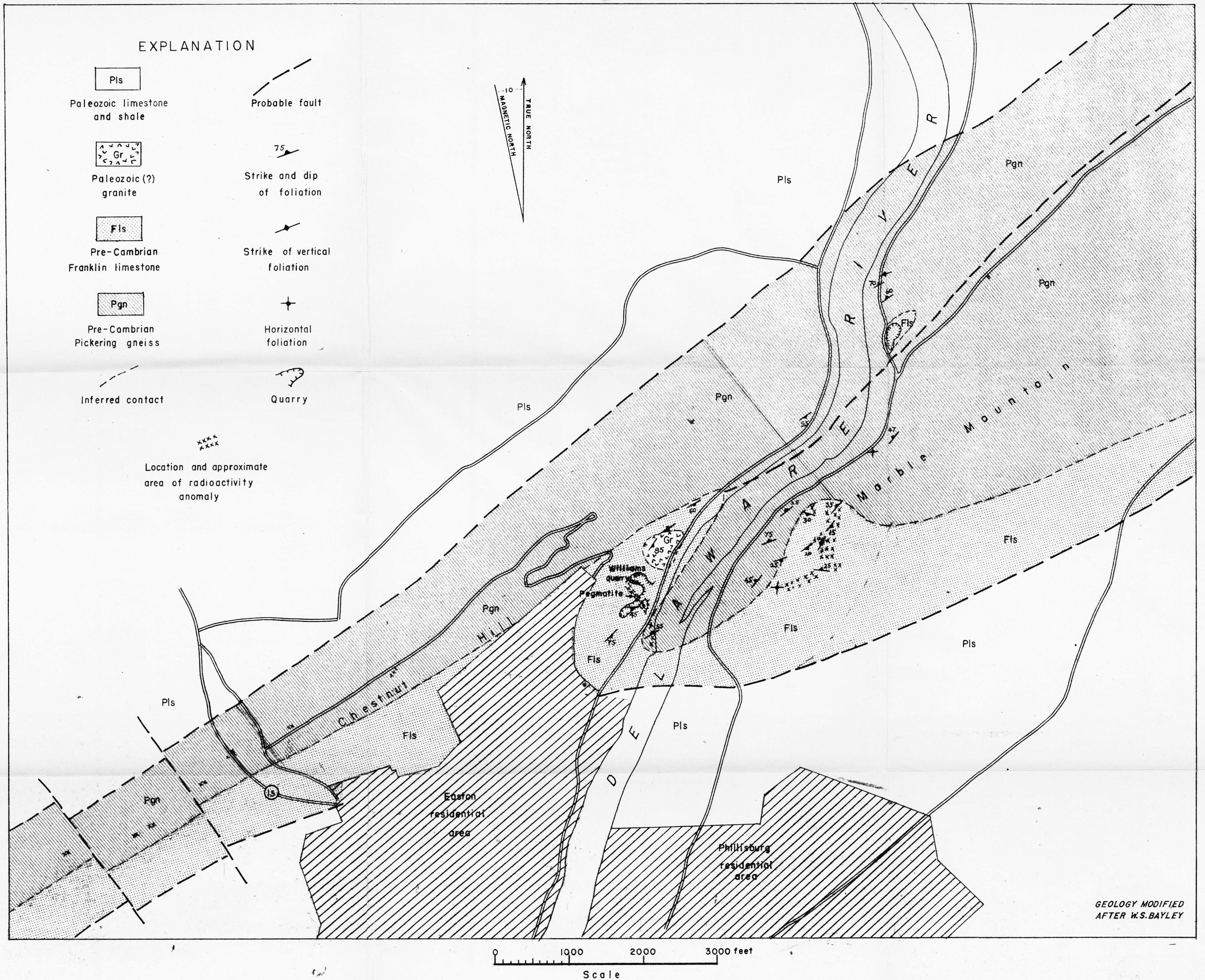
FIGURE 6—SKETCH MAP SHOWING GEOLOGY AND LOCATION OF RADIOACTIVITY ANOMALIES, CHESTNUT HILL—MARBLE MOUNTAIN AREA
